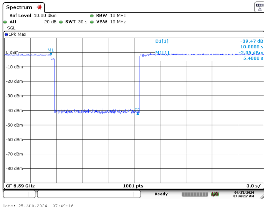
Plot 7-179. Contention Based Protocol Timing Plot (320MHz (UNII Band 7) – Ch. 159 Low)
