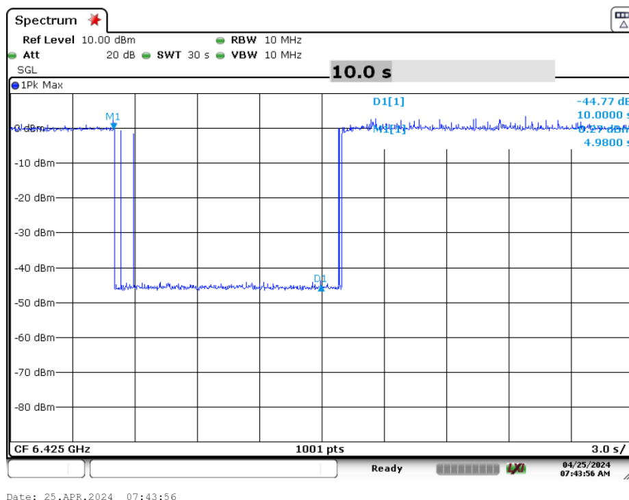
Plot 7-176. Contention Based Protocol Timing Plot (320MHz (UNII Band 6) – Ch. 95 Mid)
