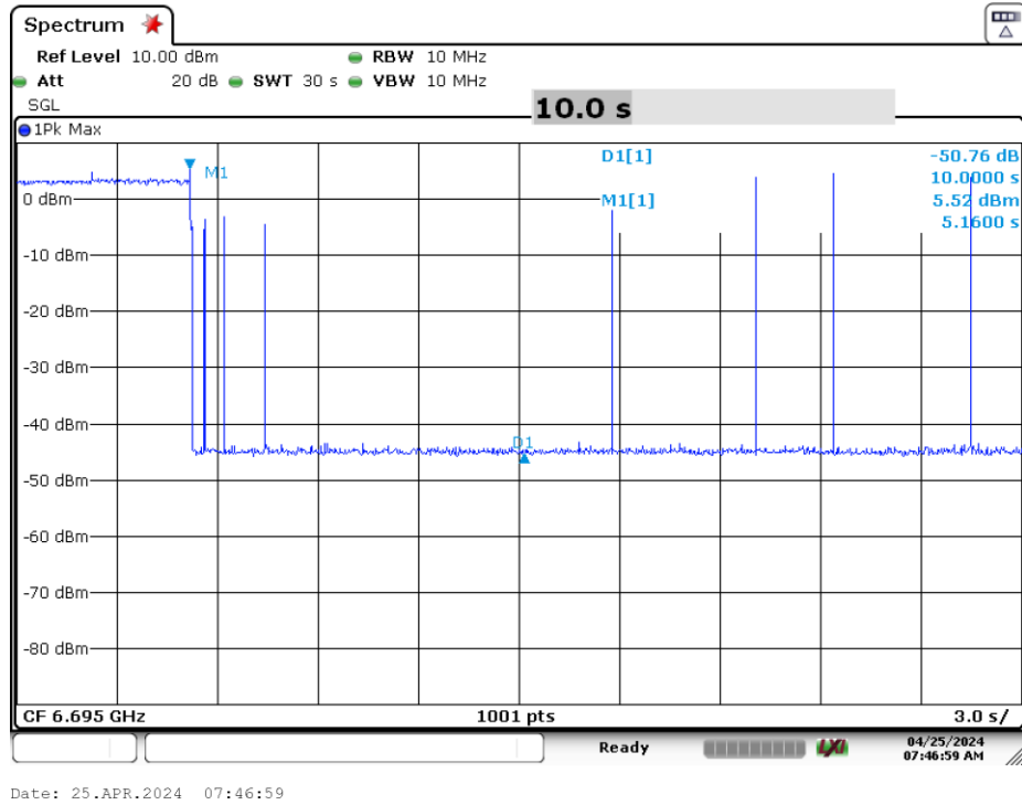
Plot 7-178. Contention Based Protocol Timing Plot (20MHz (UNII Band 7) – Ch. 149)
