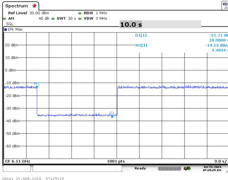
Plot 7-171. Contention Based Protocol Timing Plot (320MHz (UNII Band 5) – Ch. 31 Low)
