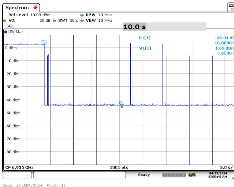
Plot 7-182. Contention Based Protocol Timing Plot (20MHz (UNII Band 8) – Ch. 197)
