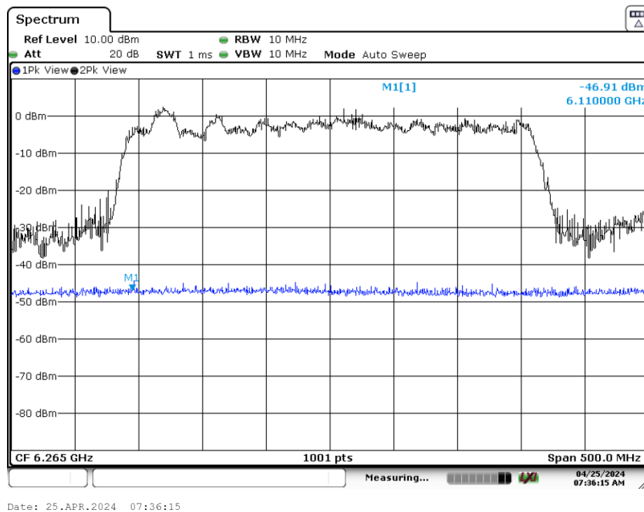
Plot 7-186. CBP 320MHz Channel - Injection Lower Edge – [6110 MHz]
