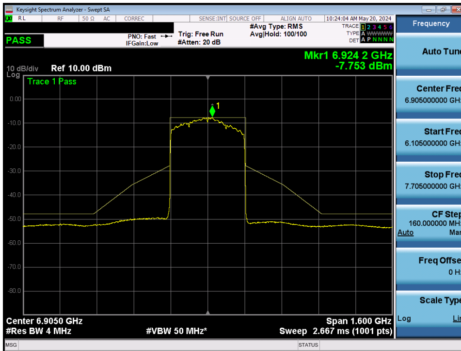
Plot 7-168. In-Band Emission MIMO ANT2 (320MHz 802.11ax/be (UNII Band 7/8) – Ch. 191) – LPI
