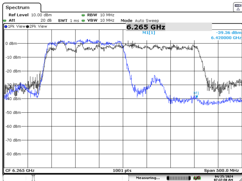
Plot 7-188. CBP 320MHz Channel - Injection Upper Edge – [6420 MHz]
