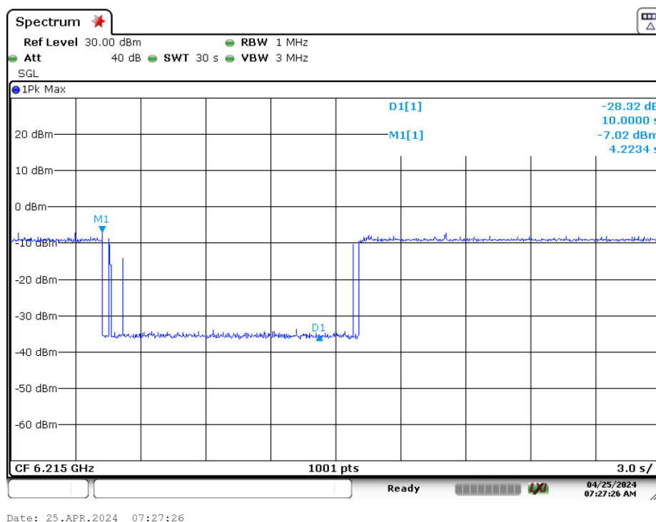
Plot 7-170. Contention Based Protocol Timing Plot (20MHz (UNII Band 5) – Ch. 53)
