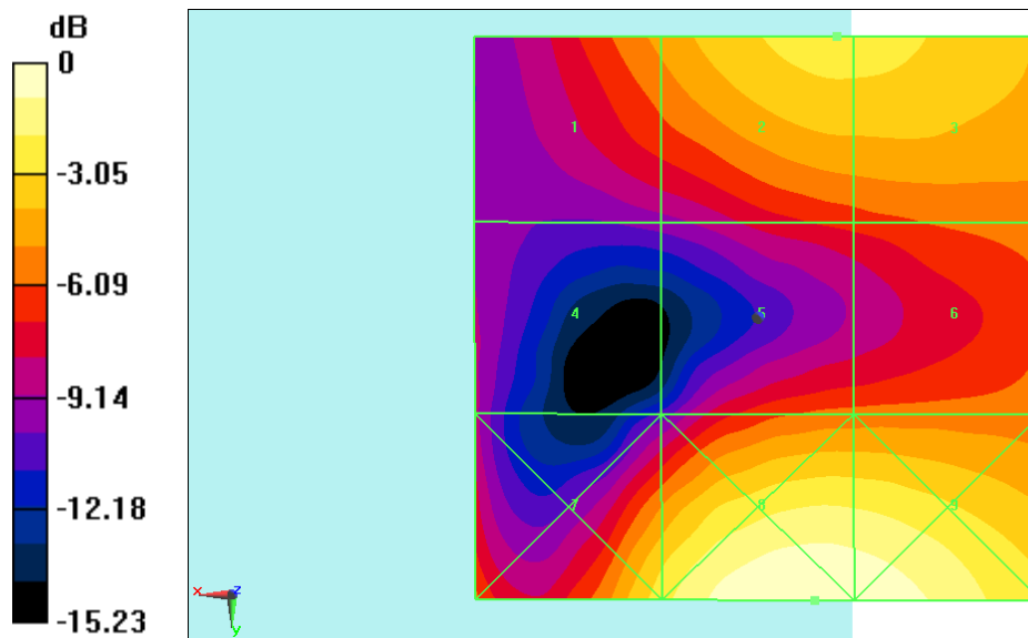
Fig B.3 HAC RF E-Field LTE Band41 PC2 QPSK
