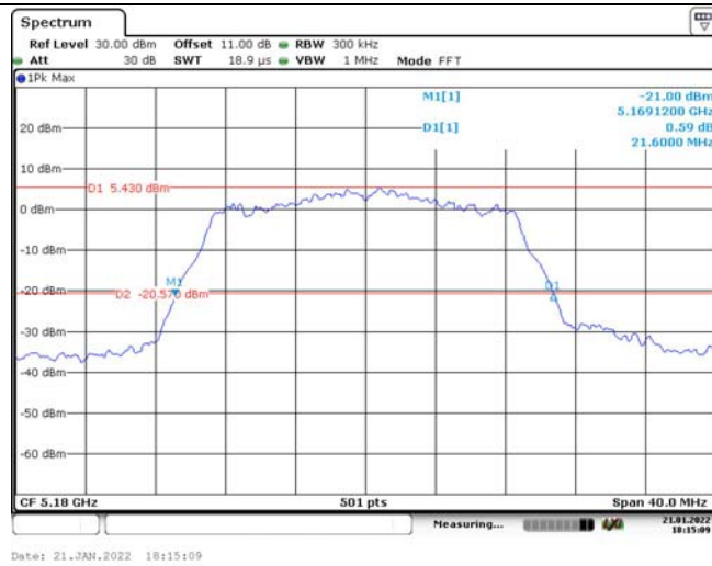
26dB Emission Bandwidth
