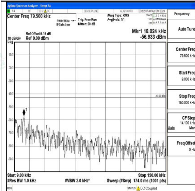
Band4_20MHz_QPSK_20300_1RB#0_0.009~0.15_0.009~ 0.15
