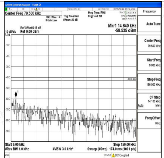
Band4_15MHz_16QAM_20325_1RB#0_0.009~0.15_0.009~0.15
