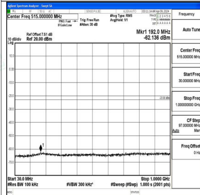
Band4_20MHz_QPSK_20175_1RB#0_30~1000_30~1000
