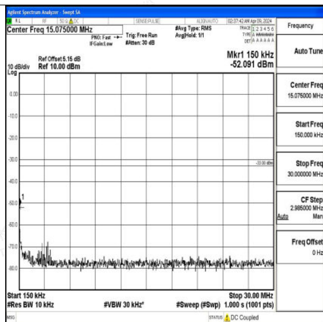
Band4_10MHz_QPSK_20175_1RB#0_0.15~30_0.15~30
