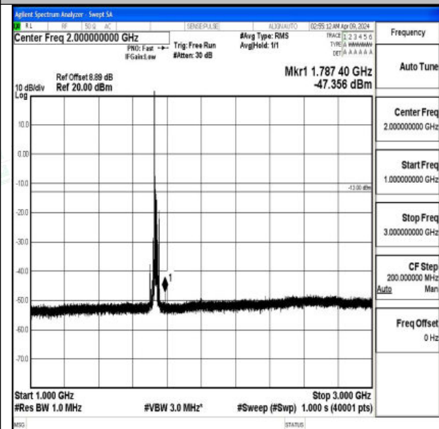
Band4_15MHz_16QAM_20175_1RB#0_1000~3000_1000 ~3000
