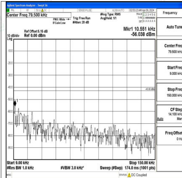
Band4_15MHz_QPSK_20025_1RB#0_0.009~0.15_0.009~0.15
