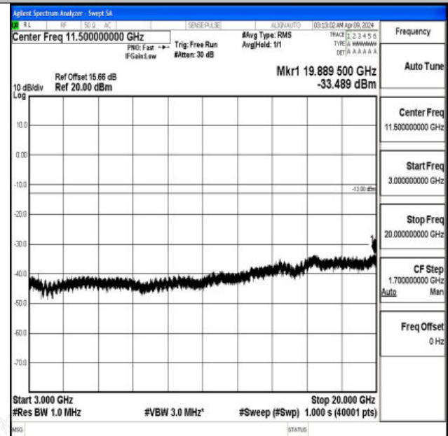
Band4_20MHz_16QAM_20300_1RB#0_3000~20000_3000~20000
