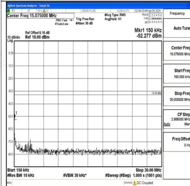
Band4_15MHz_16QAM_20325_1RB#0_0.15~30_0.15~30
