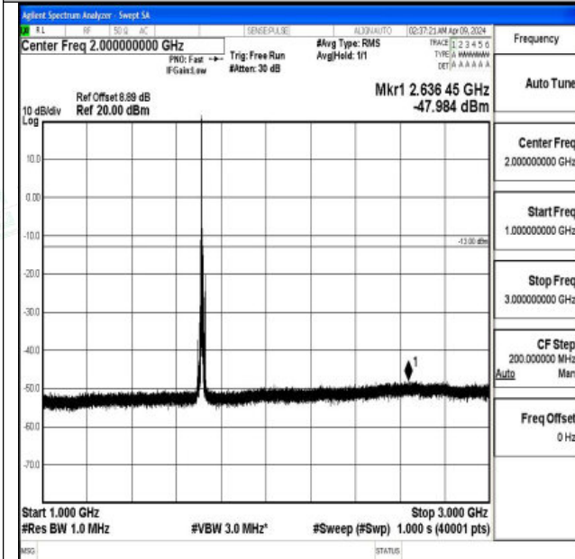
Band4_10MHz_16QAM_20000_1RB#0_1000~3000_1000~3000
