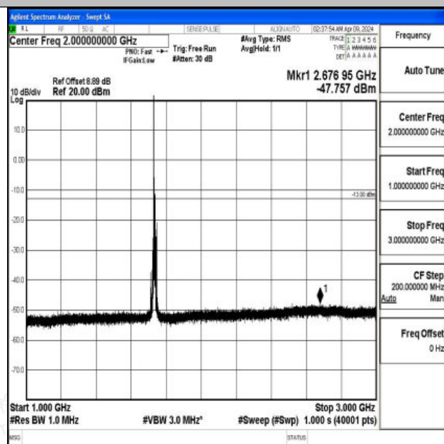
Band4_10MHz_QPSK_20175_1RB#0_1000~3000_1000~3000
