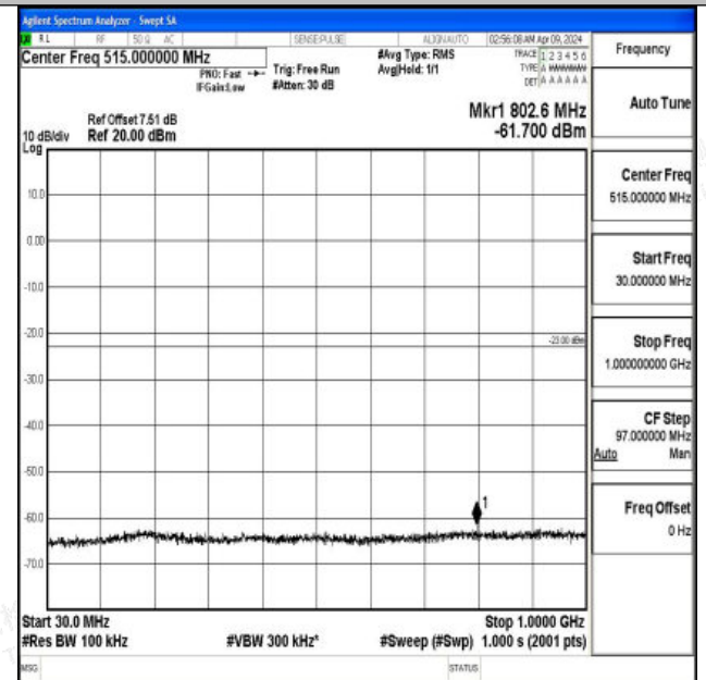
Band4_15MHz_16QAM_20325_1RB#0_30~1000_30~1000
