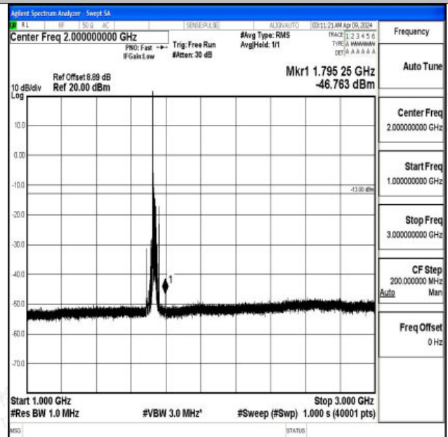
Band4_20MHz_QPSK_20175_1RB#0_1000~3000_1000~3000
