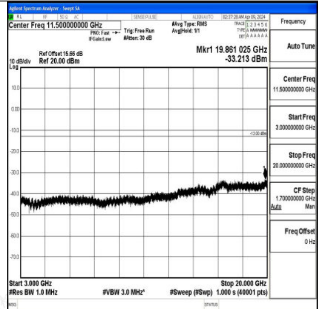
Band4_10MHz_16QAM_20000_1RB#0_3000~20000_3000~20000
