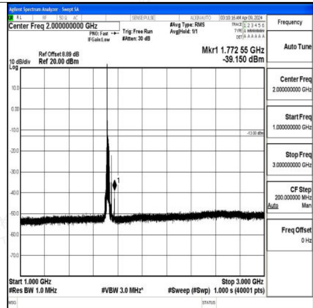
Band4_20MHz_QPSK_20050_1RB#0_1000~3000_1000~3000
