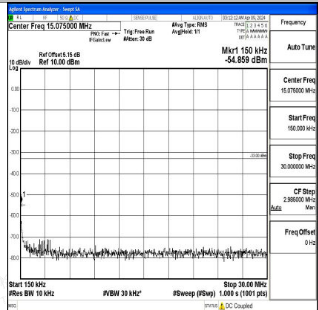
Band4_20MHz_QPSK_20300_1RB#0_0.15~30_0.15~30
