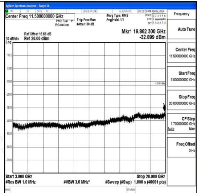
Band4_20MHz_16QAM_20175_1RB#0_3000~20000_3000 ~20000
