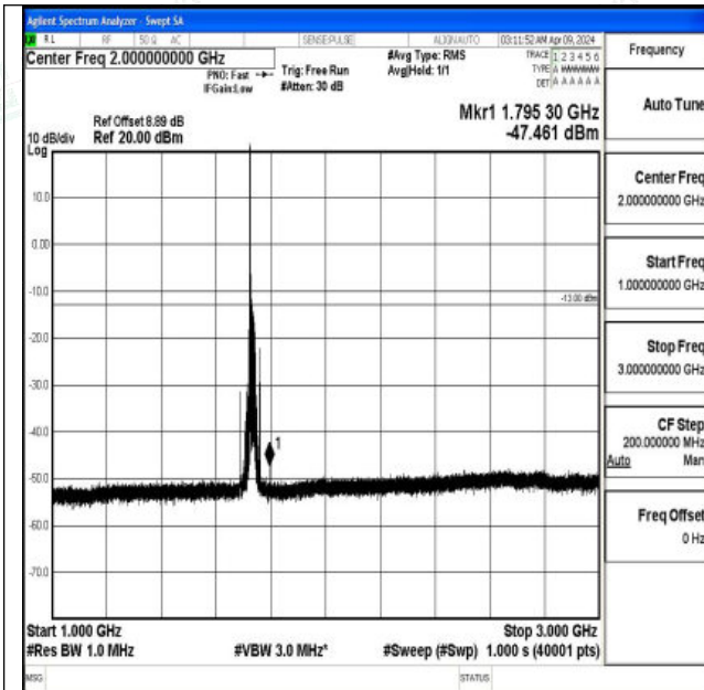
Band4_20MHz_16QAM_20175_1RB#0_1000~3000_1000 ~3000
