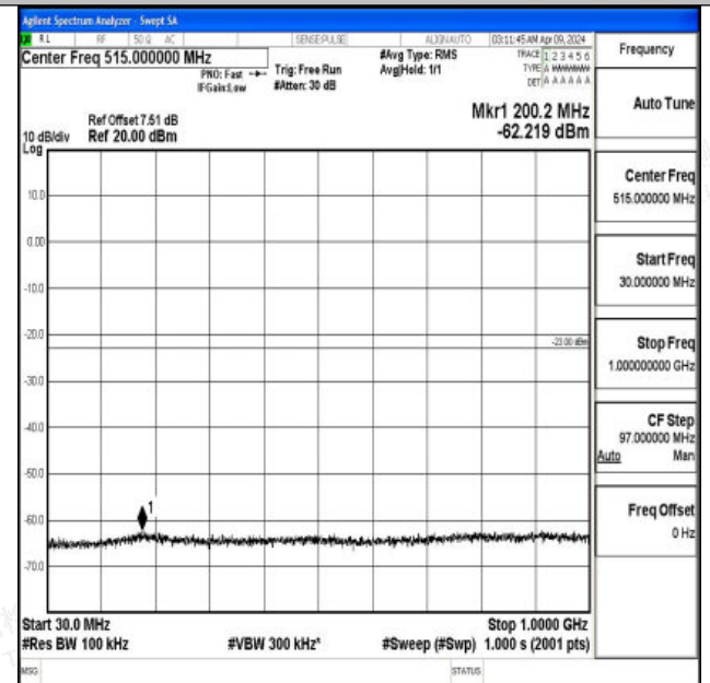
Band4_20MHz_16QAM_20175_1RB#0_30~1000_30~1000
