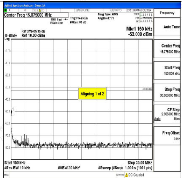
Band4_20MHz_QPSK_20175_1RB#0_0.15~30_0.15~30
