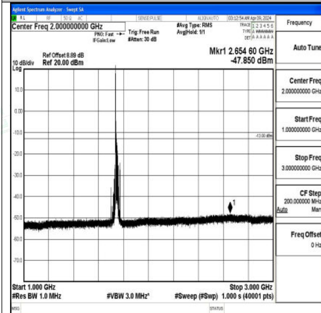
Band4_20MHz_16QAM_20300_1RB#0_1000~3000_1000~3000
