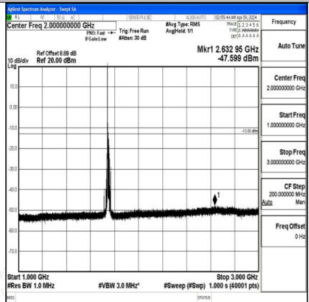
Band4_15MHz_QPSK_20325_1RB#0_1000~3000_1000~3000
