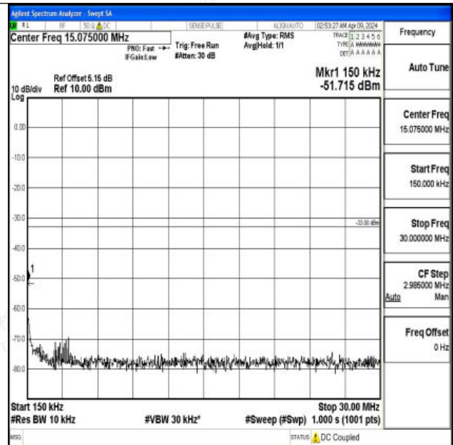
Band4_15MHz_QPSK_20025_1RB#0_0.15~30_0.15~30
