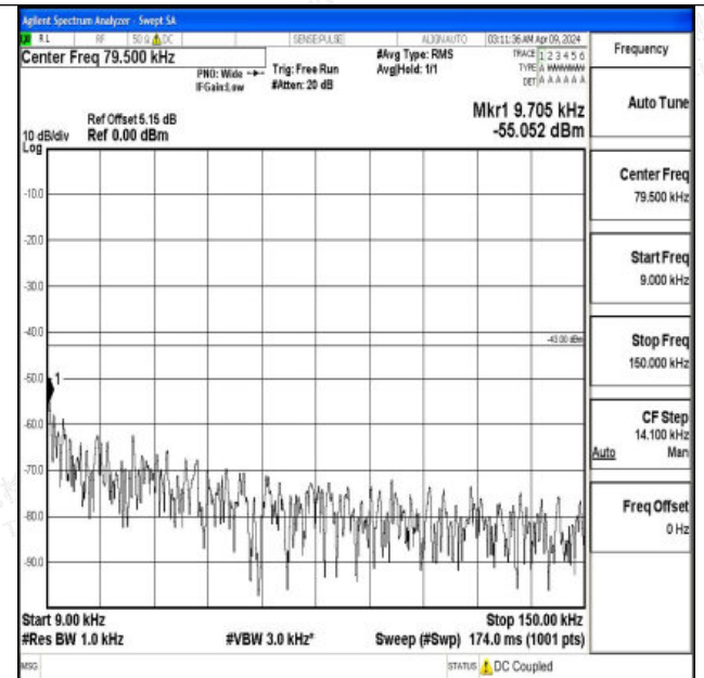
Band4_20MHz_16QAM_20175_1RB#0_0.009~0.15_0.009~0.15
