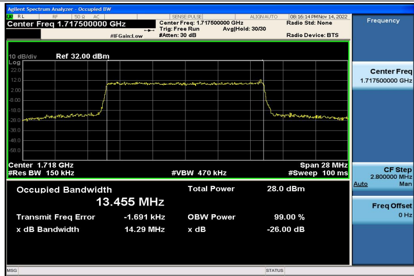
Band4-15MHz-16QAM-20025-75RB#0-13.455
