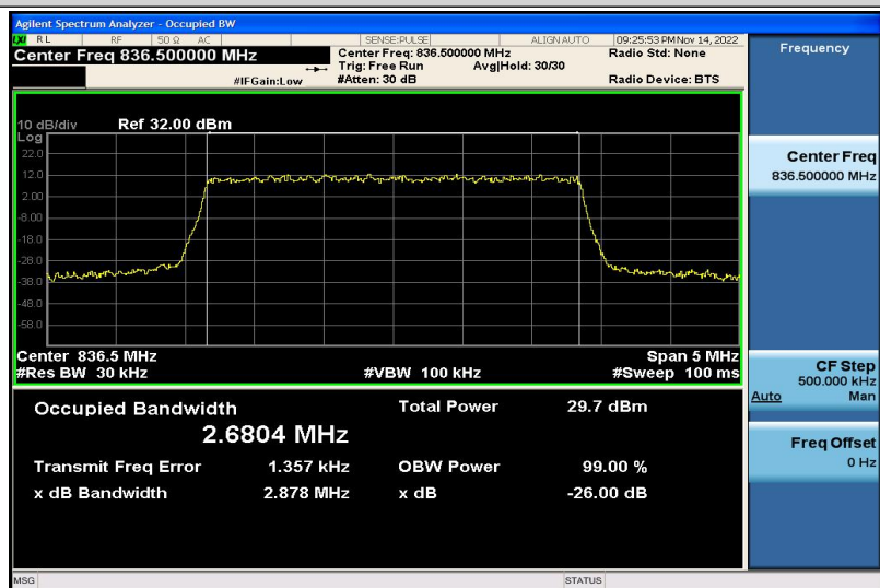
Band5-3MHz-QPSK-20525-15RB#0-2.6804
