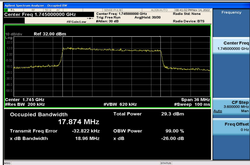
Band4-20MHz-QPSK-20300-100RB#0-17.874
