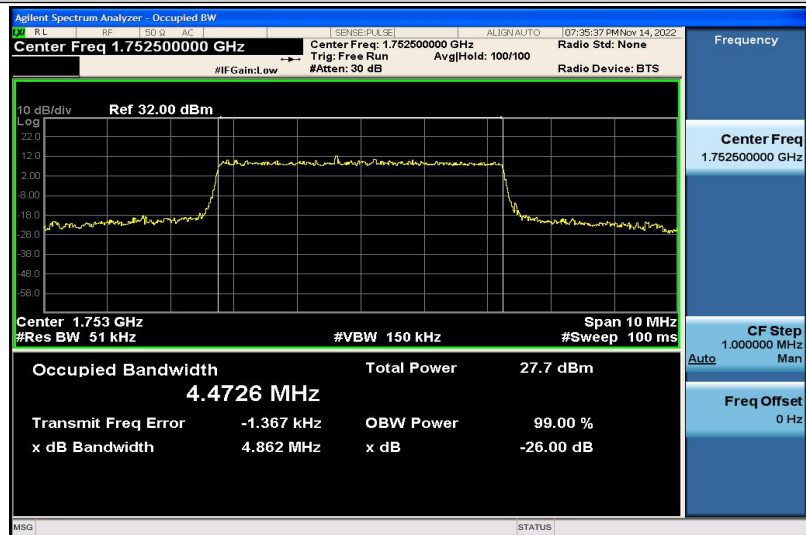
Band4-5MHz-16QAM-20375-25RB#0-4.4726
