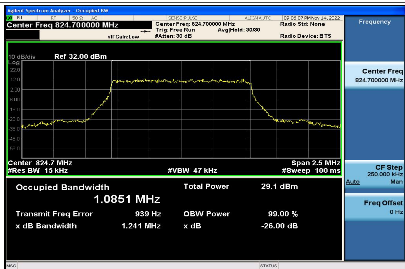
Band5-1.4MHz-QPSK-20407-6RB#0-1.0851
