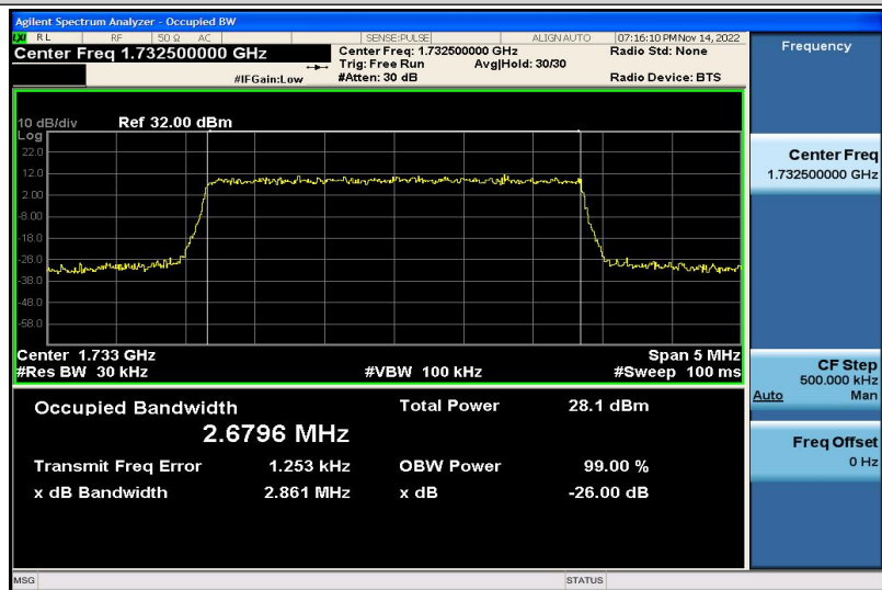
Band4-3MHz-QPSK-20175-15RB#0-2.6796
