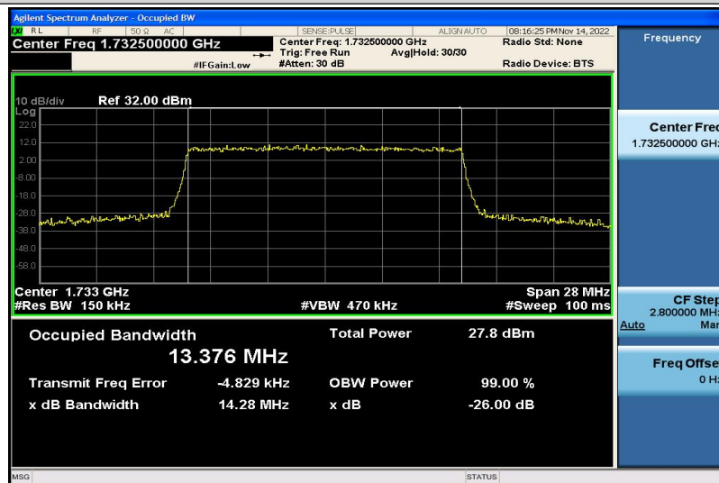
Band4-15MHz-QPSK-20175-75RB#0-13.376
