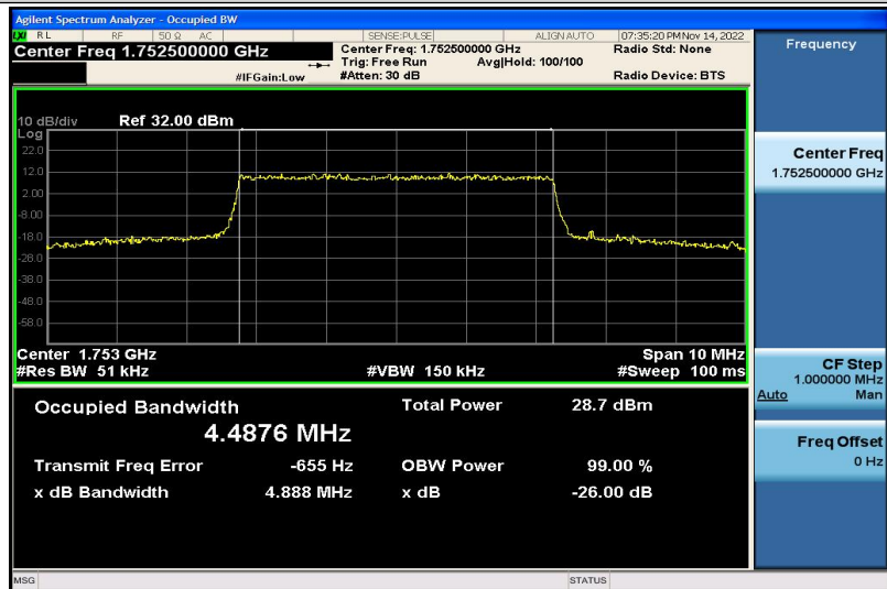
Band4-5MHz-QPSK-20375-25RB#0-4.4876
