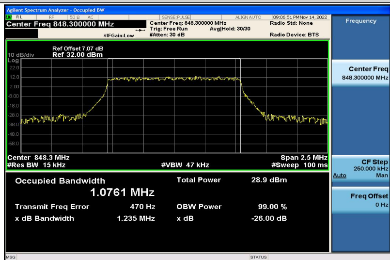
Band5-1.4MHz-QPSK-20643-6RB#0-1.0761
