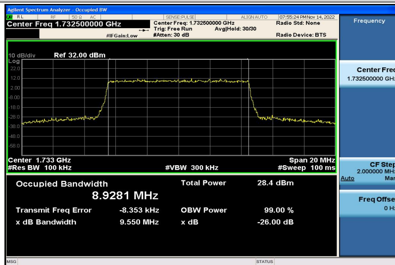
Band4-10MHz-QPSK-20175-50RB#0-8.9281
