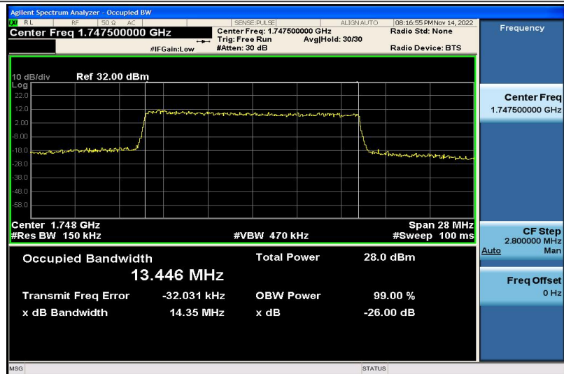
Band4-15MHz-16QAM-20325-75RB#0-13.446
