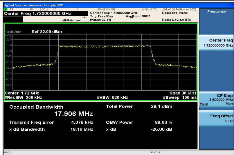
Band4-20MHz-QPSK-20050-100RB#0-17.906
