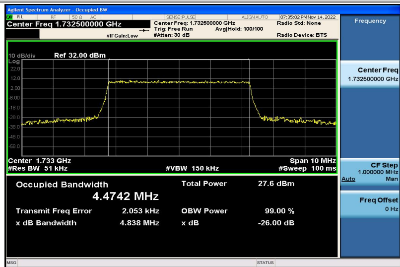
Band4-5MHz-16QAM-20175-25RB#0-4.4742
