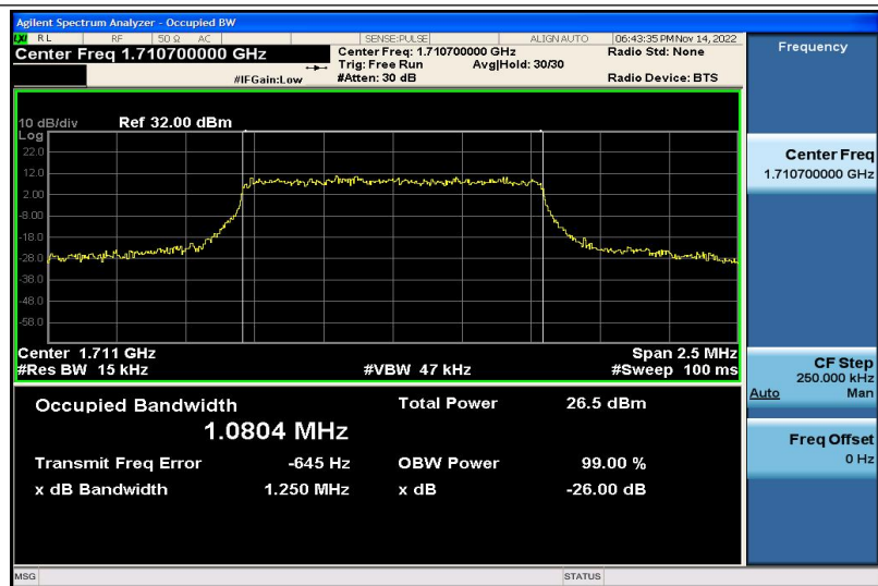
Band4-1.4MHz-16QAM-19957-6RB#0-1.0804
