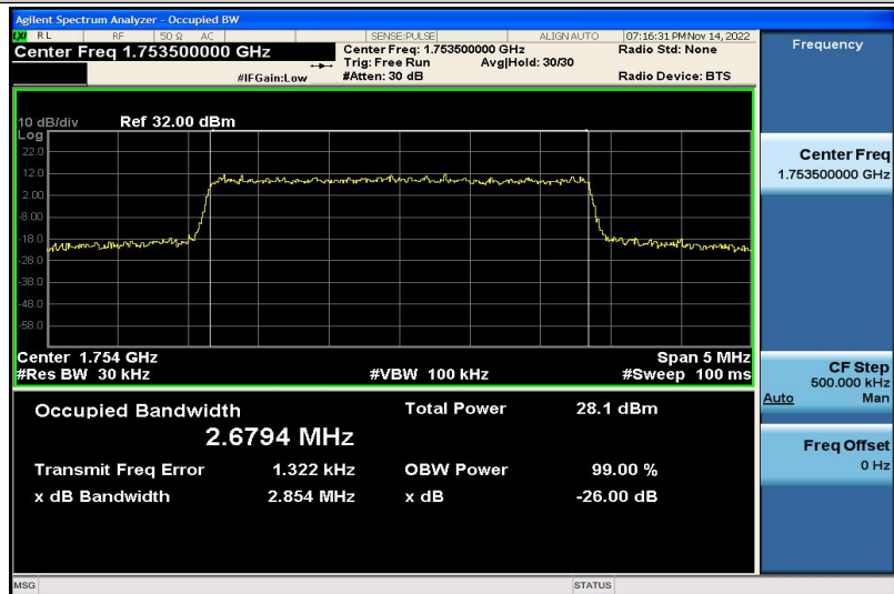
Band4-3MHz-QPSK-20385-15RB#0-2.6794
