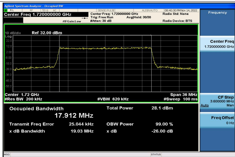
Band4-20MHz-16QAM-20050-100RB#0-17.912
