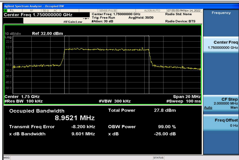
Band4-10MHz-16QAM-20350-50RB#0-8.9521
