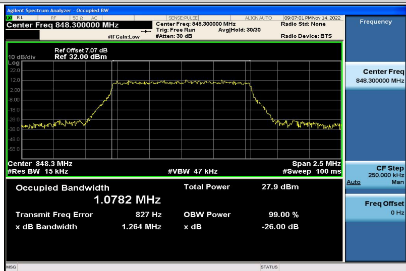
Band5-1.4MHz-16QAM-20643-6RB#0-1.0782
