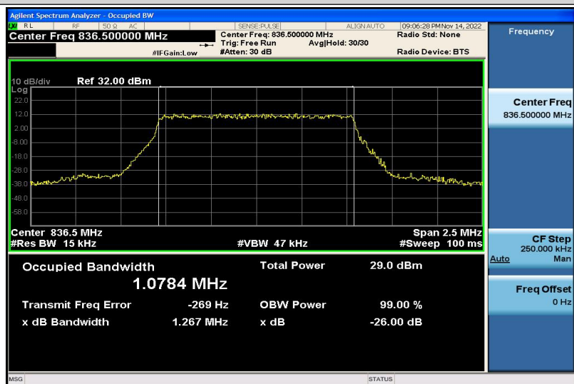
Band5-1.4MHz-QPSK-20525-6RB#0-1.0784
