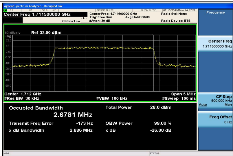
Band4-3MHz-QPSK-19965-15RB#0-2.6781
