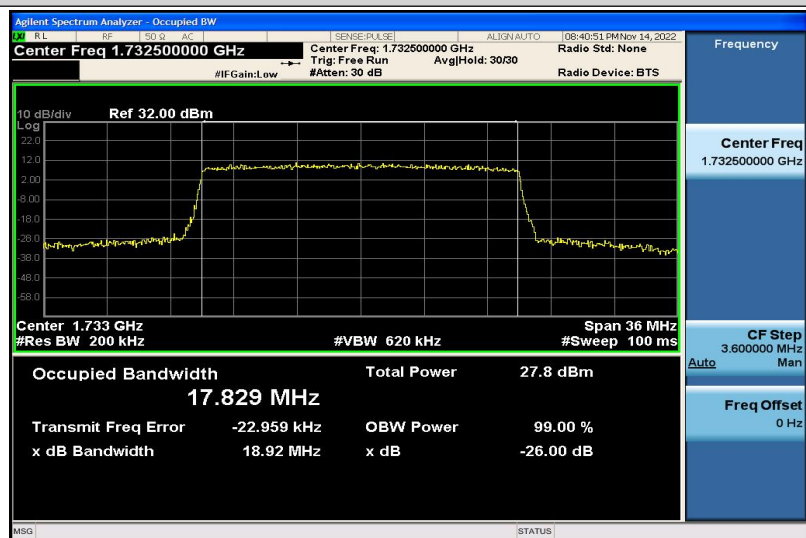
Band4-20MHz-16QAM-20175-100RB#0-17.829
