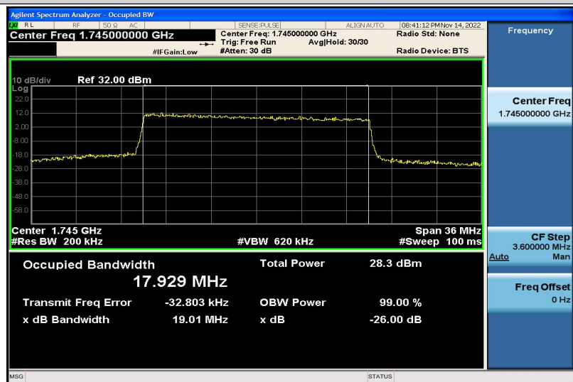
Band4-20MHz-16QAM-20300-100RB#0-17.929
