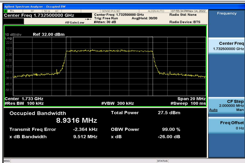
Band4-10MHz-16QAM-20175-50RB#0-8.9316
