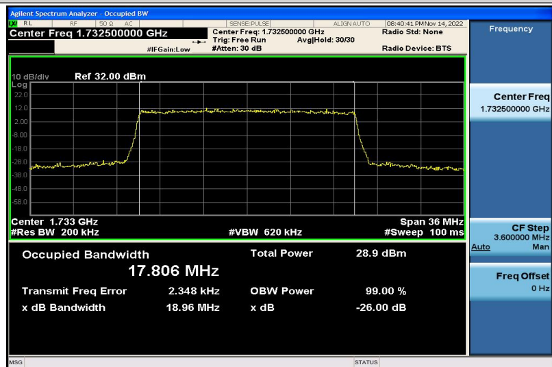
Band4-20MHz-QPSK-20175-100RB#0-17.806
