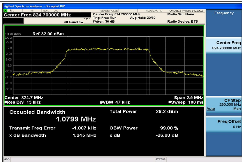
Band5-1.4MHz-16QAM-20407-6RB#0-1.0799
