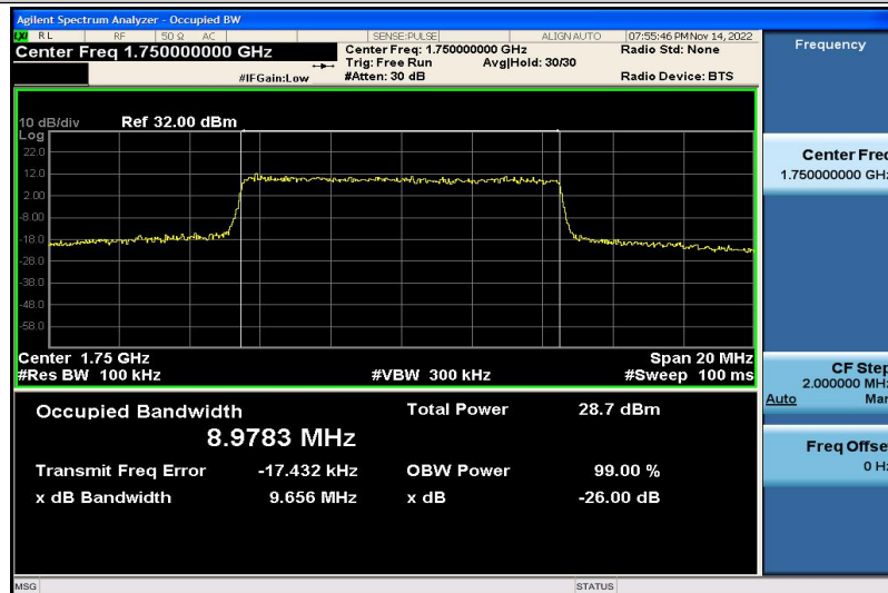
Band4-10MHz-QPSK-20350-50RB#0-8.9783
