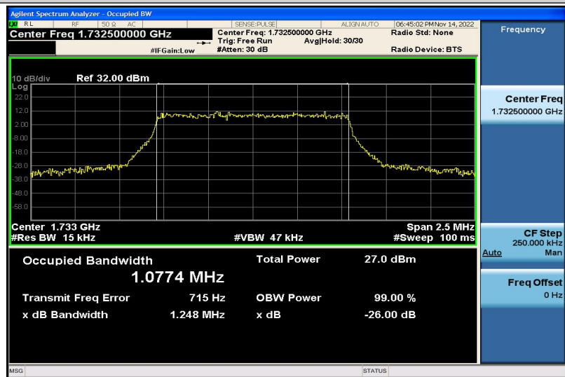
Band4-1.4MHz-16QAM-20175-6RB#0-1.0774
