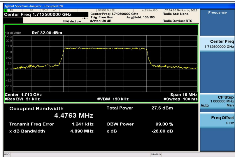
Band4-5MHz-16QAM-19975-25RB#0-4.4763
