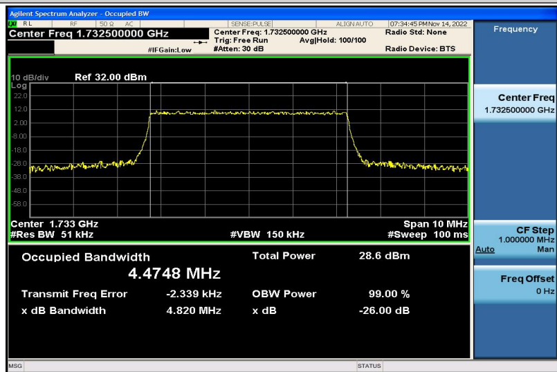
Band4-5MHz-QPSK-20175-25RB#0-4.4748
