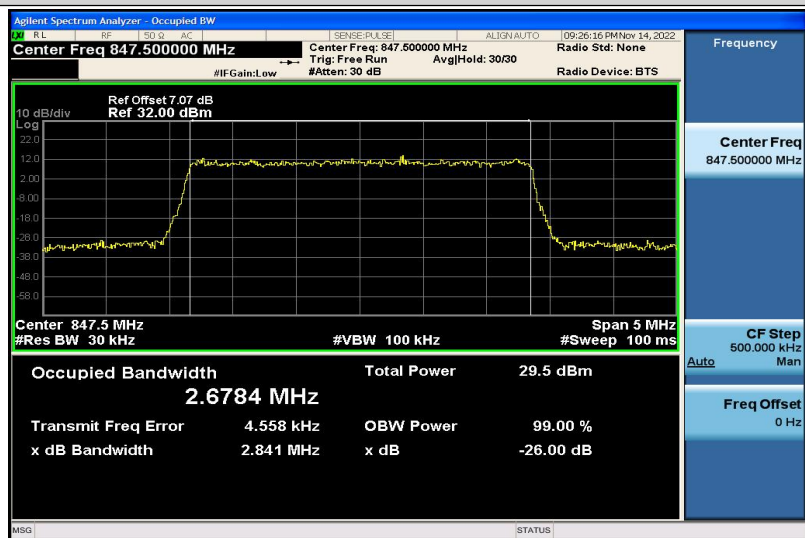
Band5-3MHz-QPSK-20635-15RB#0-2.6784
