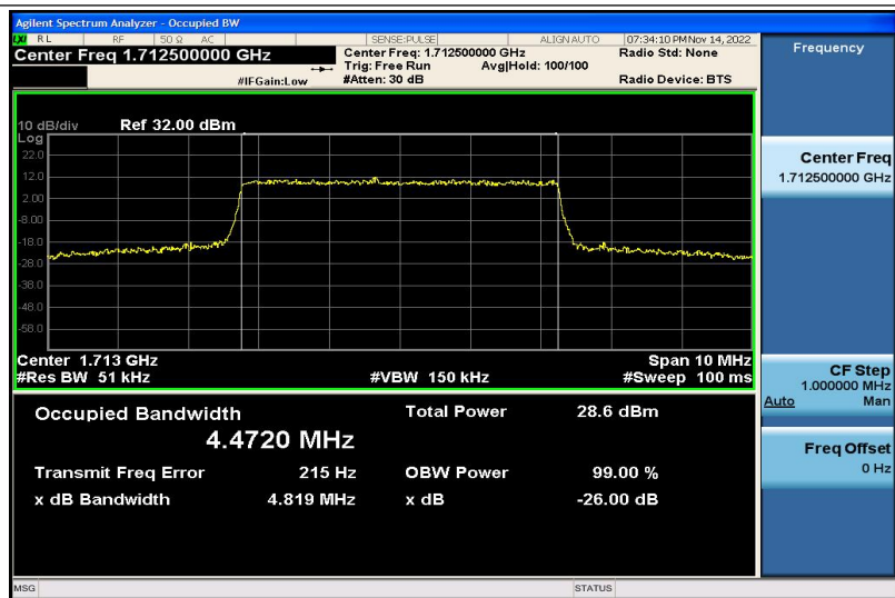
Band4-5MHz-QPSK-19975-25RB#0-4.4720
