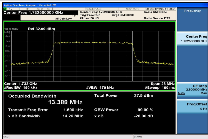
Band4-15MHz-16QAM-20175-75RB#0-13.388
