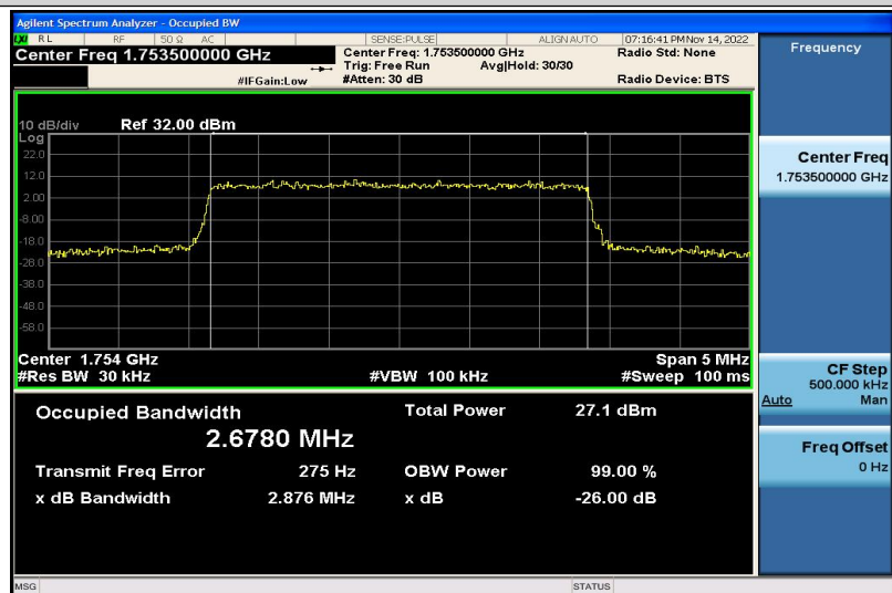
Band4-3MHz-16QAM-20385-15RB#0-2.6780
