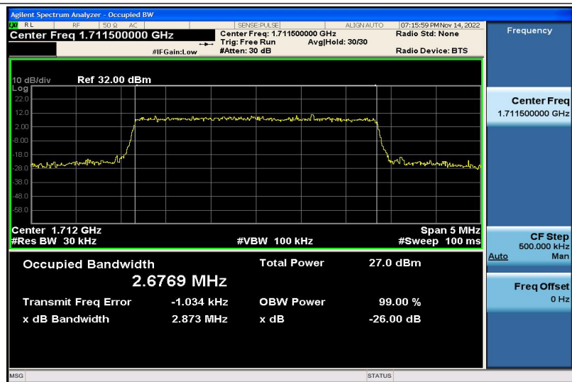
Band4-3MHz-16QAM-19965-15RB#0-2.6769
