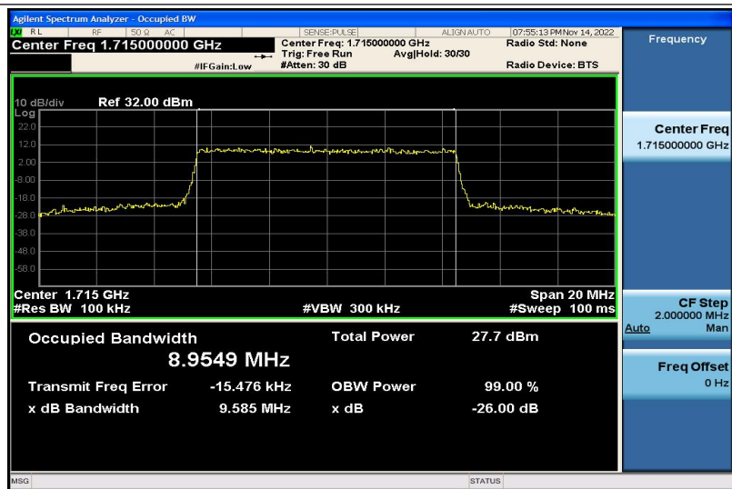
Band4-10MHz-16QAM-20000-50RB#0-8.9549
