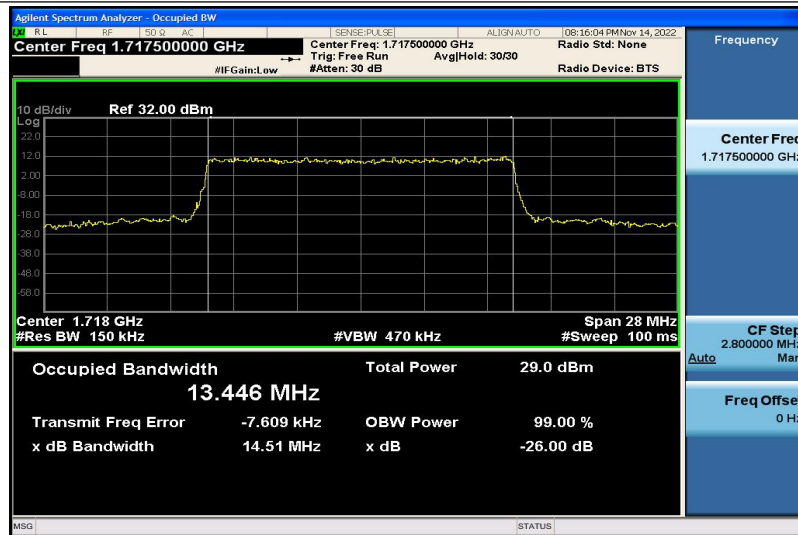
Band4-15MHz-QPSK-20025-75RB#0-13.446
