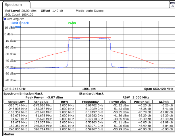
802.11ax (160MHz) 6345MHz Chain C NSS-1
