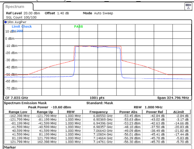
802.11ax (80MHz) 7025MHz Chain D NSS-1
