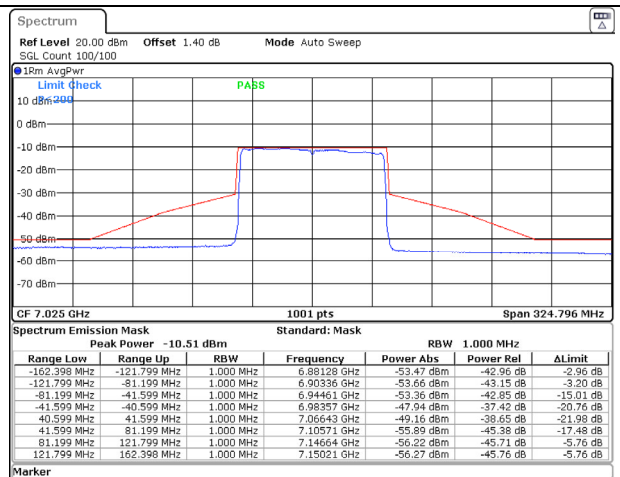
802.11ax (80MHz) 7025MHz Chain B NSS-1
