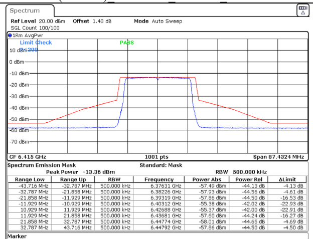
802.11ax (20MHz) 6415MHz Chain B NSS-2
