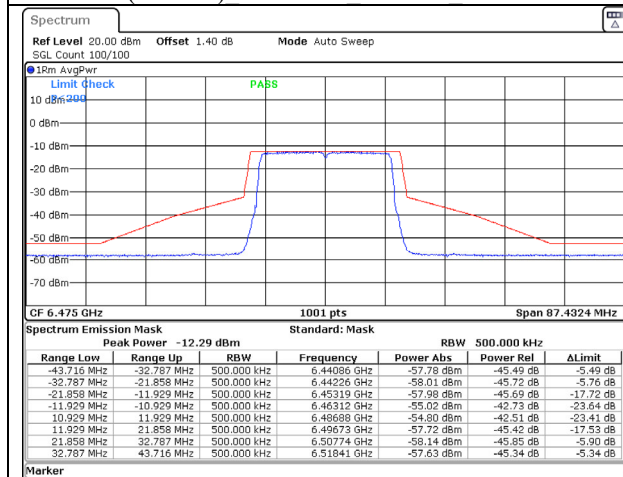
802.11ax (20MHz) 6475MHz Chain A NSS-2
