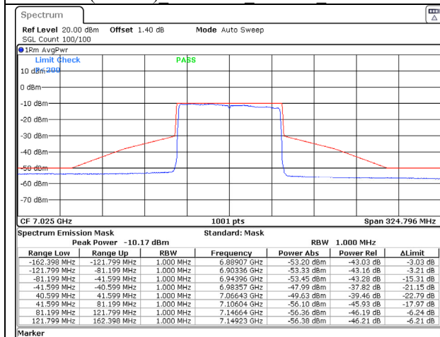
802.11ax (80MHz) 7025MHz Chain C NSS-1
