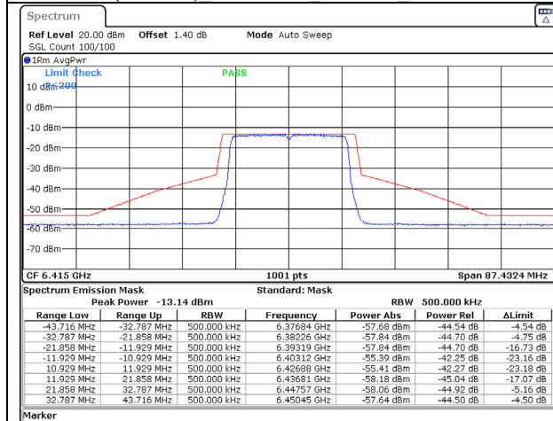
802.11ax (20MHz) 6415MHz Chain C NSS-2
