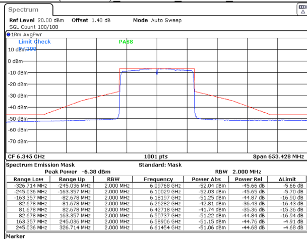
802.11ax (160MHz) 6345MHz Chain A NSS-1
