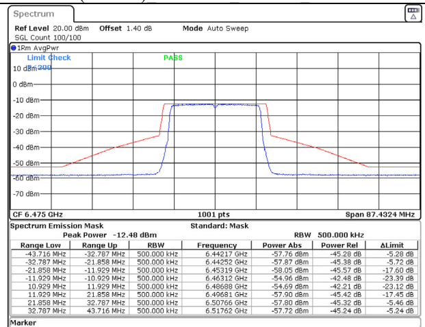
802.11ax (20MHz) 6475MHz Chain B NSS-2
