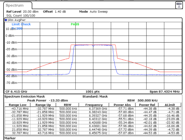
802.11ax (20MHz) 6415MHz Chain D NSS-2
