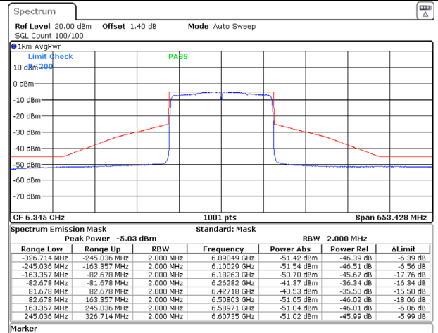
802.11ax (160MHz) 6345MHz Chain D NSS-1
