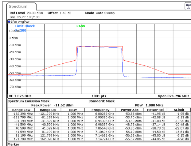
802.11ax (80MHz) 7025MHz Chain A NSS-1
