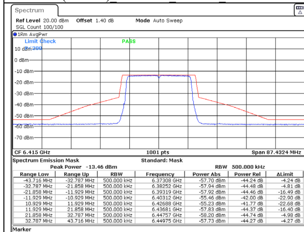
802.11ax (20MHz) 6415MHz Chain A NSS-2
