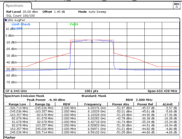
802.11ax (160MHz) 6345MHz Chain B NSS-1
