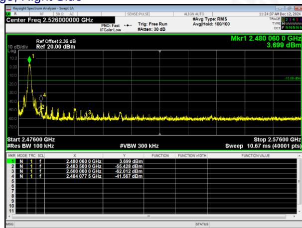
GFSK: Band Edge, Right Side
