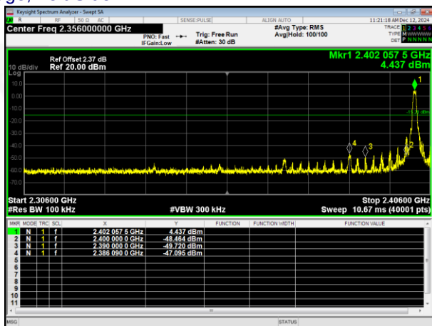
GFSK: Band Edge, Left Side
