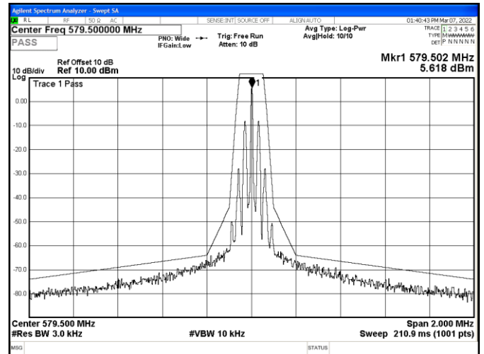
Channel 7/ 579.5 MHz
