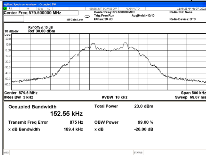
Channel 07 / 579.5 MHz
