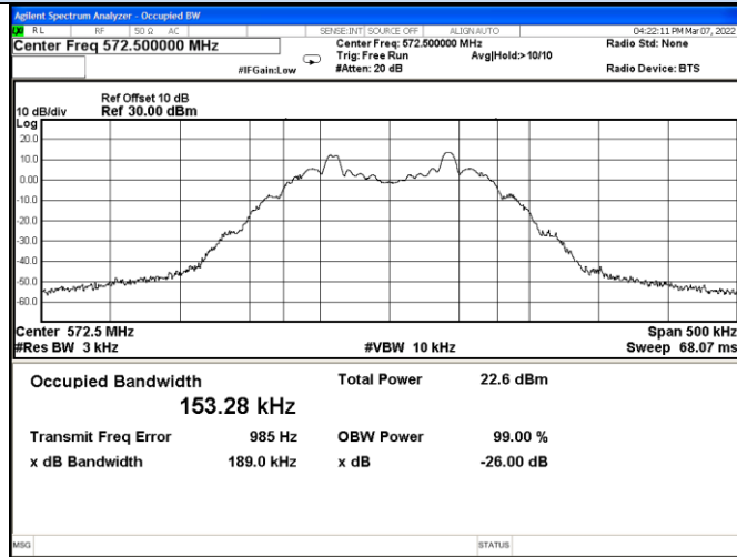
Channel 0 / 572.5MHz
