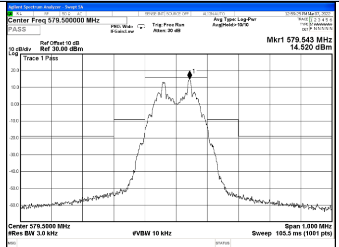
Channel 22 / 579.5 MHz
