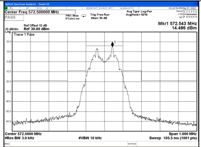
Channel 15 / 572.5MHz
