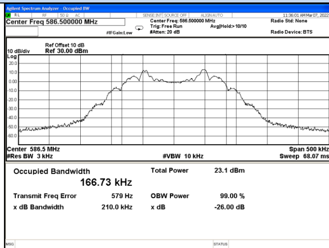
Channel 14/ 586.5 MHz
