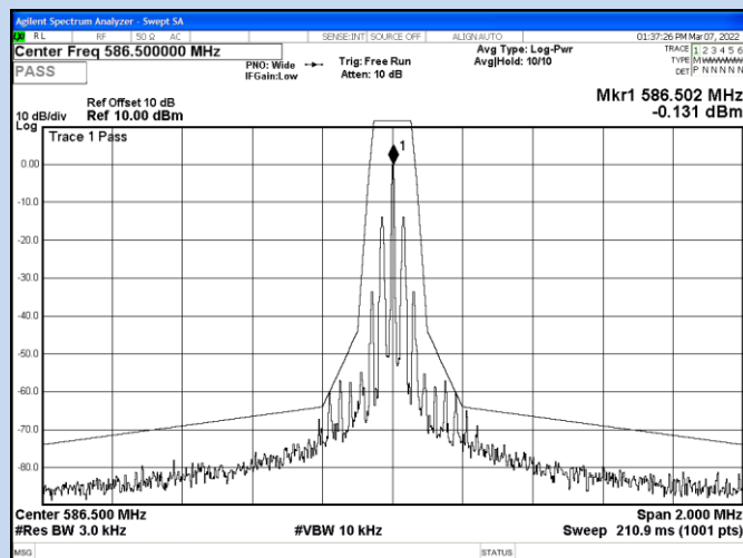
Channel 14/ 586.5 MHz
