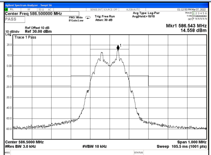
Channel 29 / 586.5 MHz
