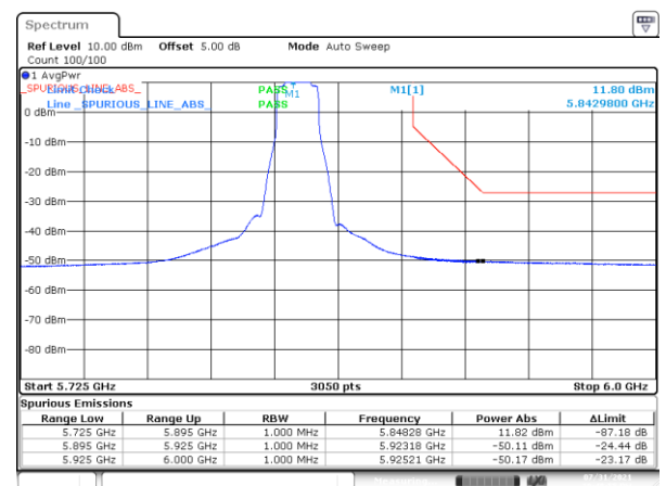
BE-NR-HIGH, SISO-A, 802.11n20-HT0, Ch169
