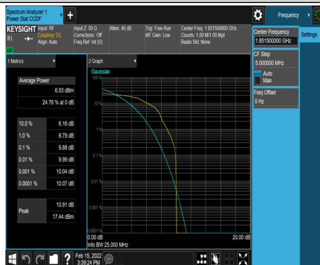
Band25-3MHz-16QAM-26055-1-0-Low-9.88-<=13-PASS
