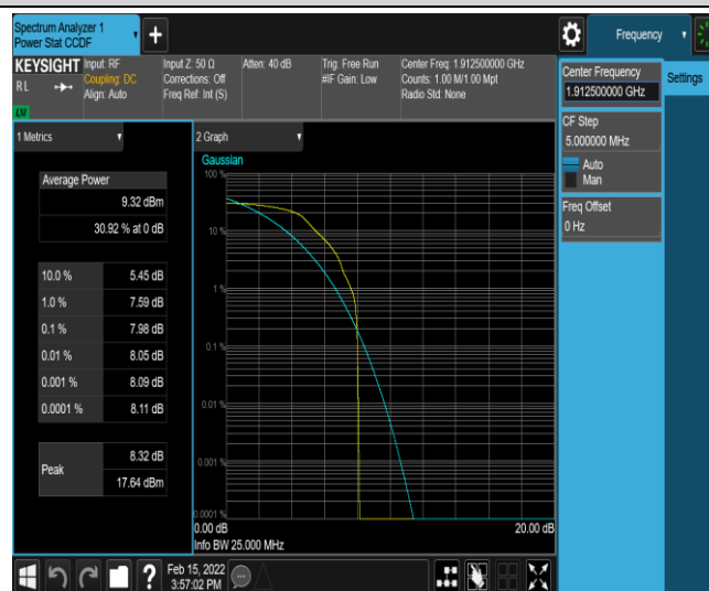
Band25-5MHz-QPSK-26665-1-0-High-7.98-<=13-PASS
