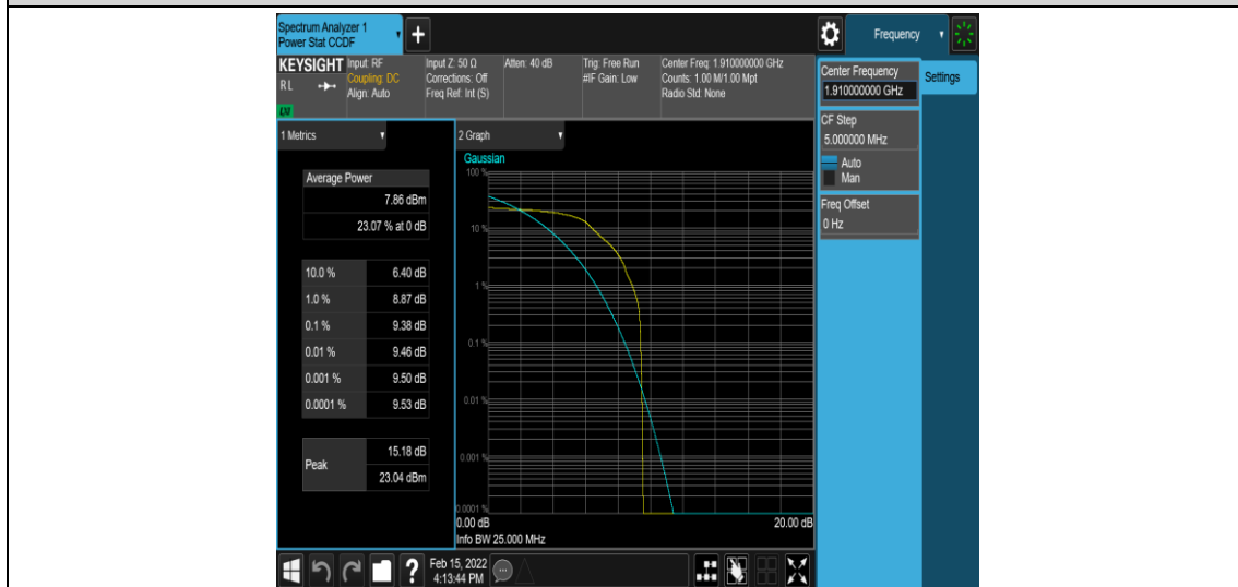
Band25-10MHz-QPSK-26640-1-0-High-9.38-<=13-PASS
