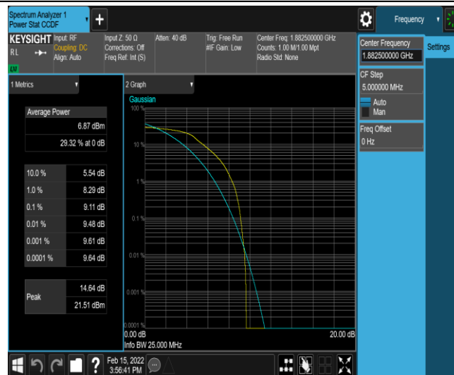
Band25-5MHz-QPSK-26365-6-0-Low-9.11-<=13-PASS
