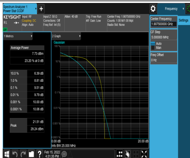
Band25-15MHz-QPSK-26615-6-0-High-9.51-&lt;=13-PASS
