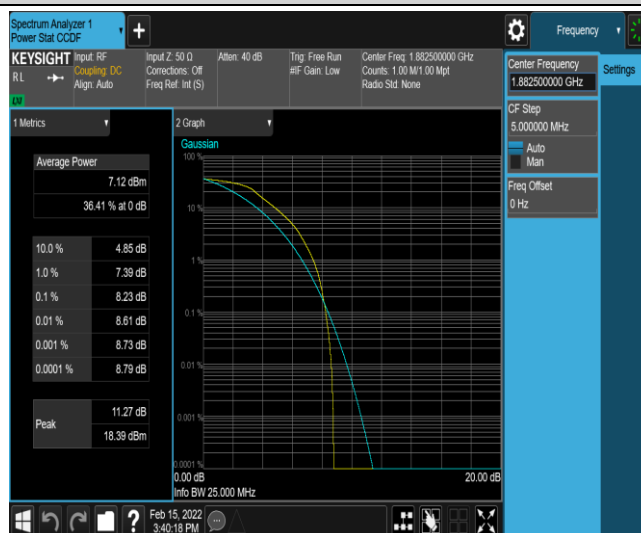
Band25-3MHz-16QAM-26365-6-0-Low-8.23-&lt;=13-PASS
