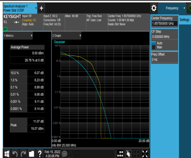
Band25-15MHz-16QAM-26115-1-0-Low-8.99-&lt;=13-PASS
