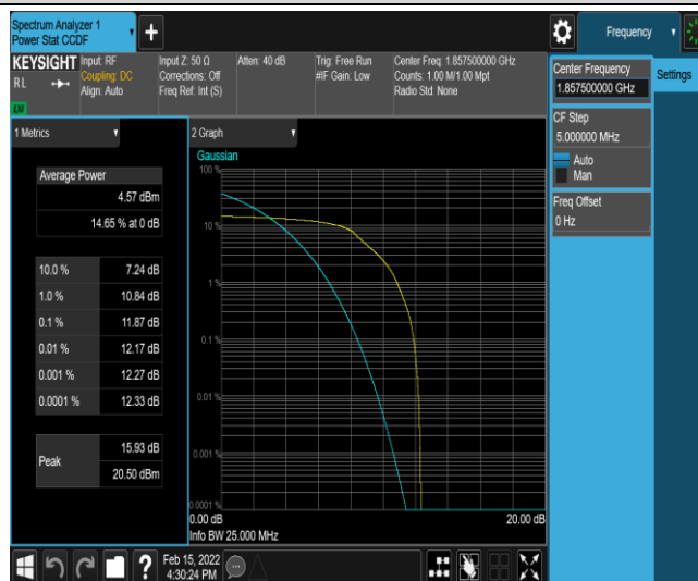
Band25-15MHz-16QAM-26115-6-0-Low-11.87-&lt;=13-PASS
