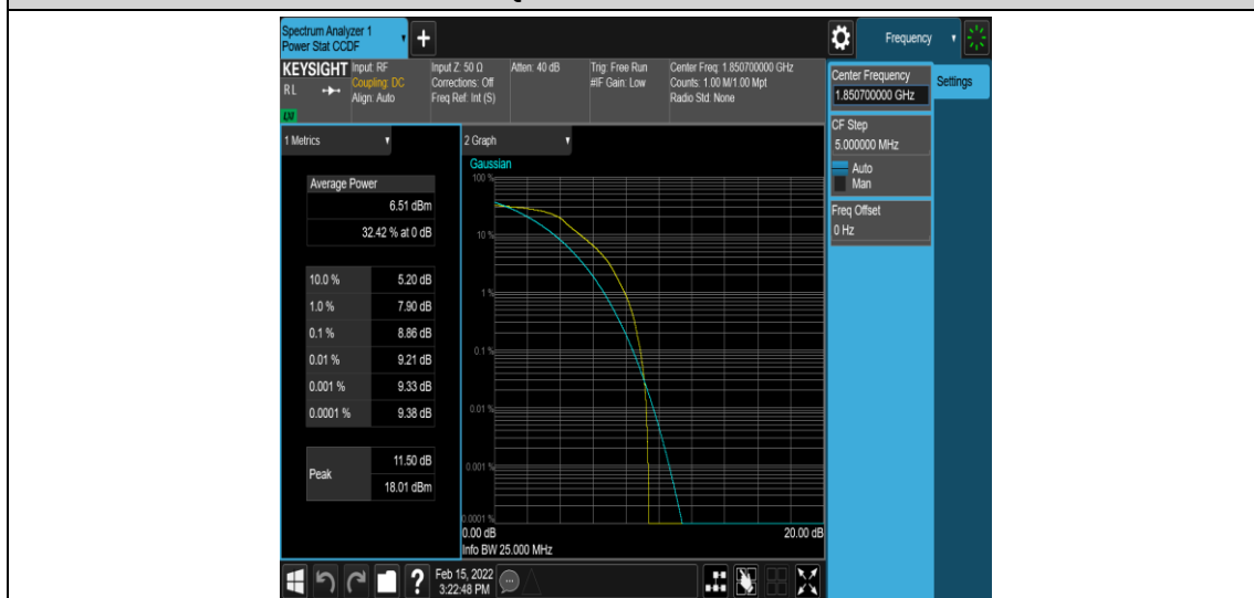
Band25-1.4MHz-16QAM-26047-6-0-Low-8.86-<=13-PASS
