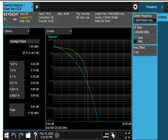
Band25-1.4MHz-QPSK-26047-1-0-Low-8.76-<=13-PASS
