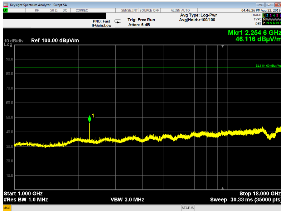
Plot 3.6.7: Spurious Emissions test results, 1 GHz – 18 GHz range, Horizontal polarization, Middle Frequency
