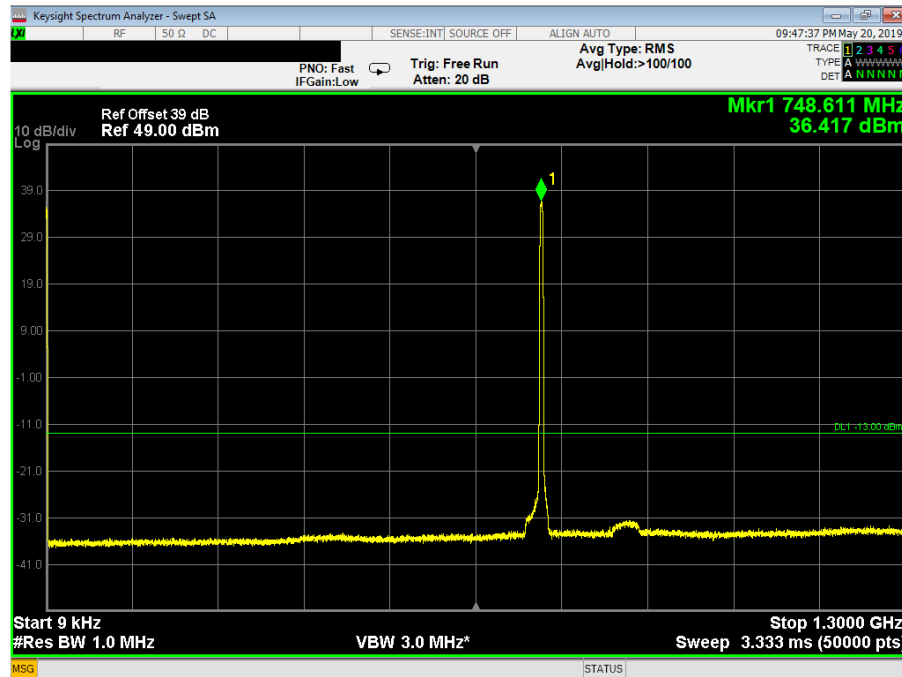
Plot 3.5.1: Spurious Emission Conducted Measurement, AWGN 4.1MHz, F_c = 748.500 MHz, 9 kHz – 1.3 GHz
