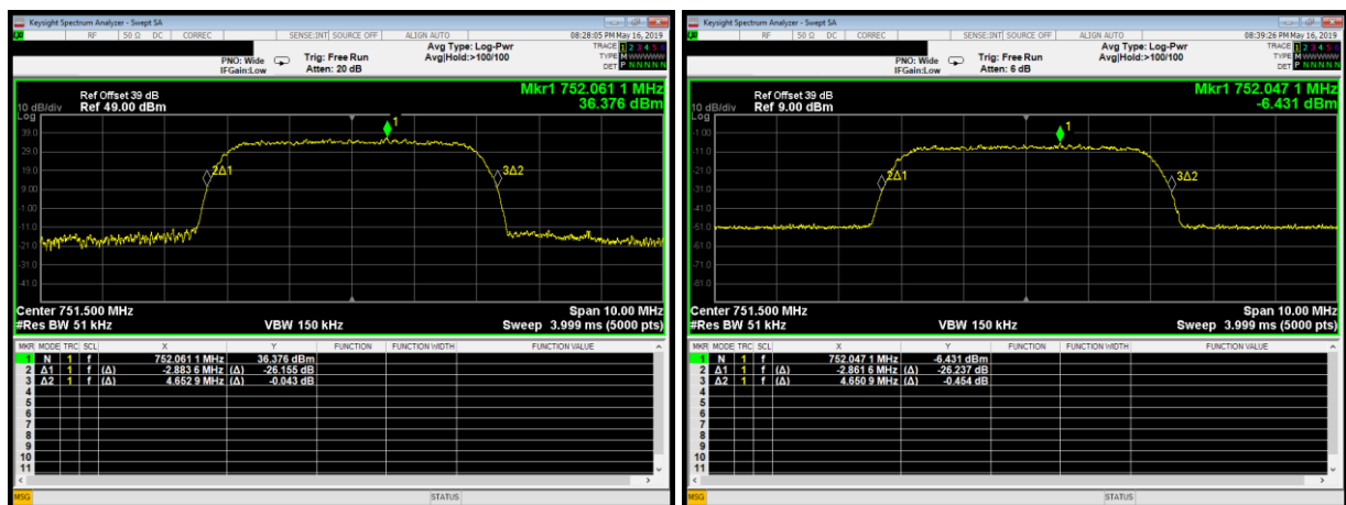
Plot 3.2.2: Input-versus-output signal comparison, AWGN 4.1MHz, 3 dB above AGC threshold level
