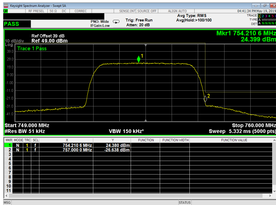
Plot 3.4.3: Band Edge test results, AWGN 4.1MHz, Fc = 754.500 MHz, single test signal
