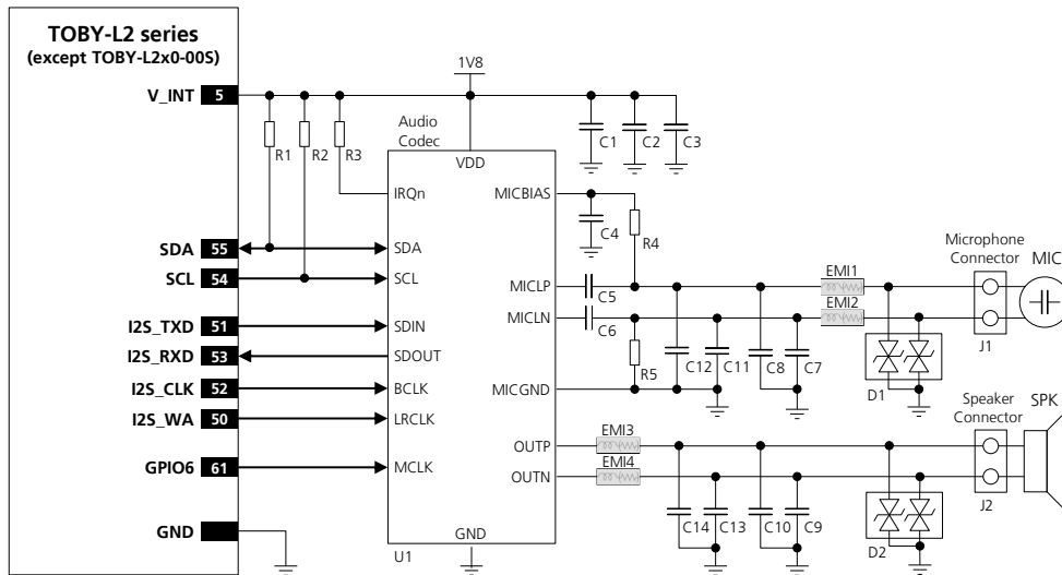
Figure 60: I²S interface application circuit with an external audio codec to provide voice capability
