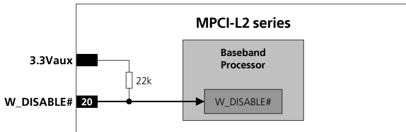
Figure 20: MPCPI-L2 series modules W_DISABLE# input circuit description
