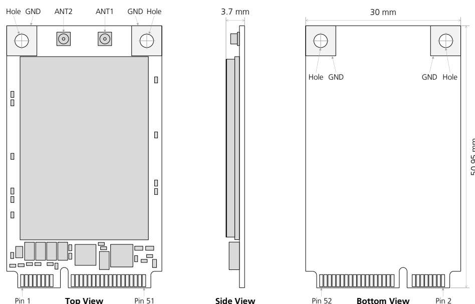
Figure 66: MPC1-L2 series mechanical description (top, side and bottom views)
