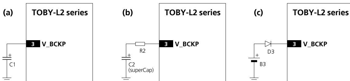
Figure 35: Real time clock supply (V_BCKP) application circuits: (a) using a 100 μF capacitor to let the RTC run for ~80 s after VCC removal; (b) using a 70 mF capacitor to let RTC run for ~15 hours after VCC removal; (c) using a non-rechargeable battery
