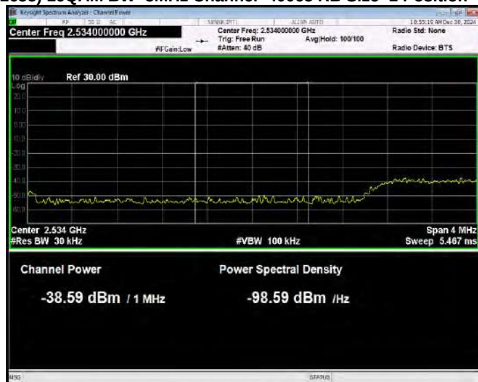
Band41(2535-2655) 16QAM BW=5MHz Channel=40065 RB Size=1 Position=#Max Normal
