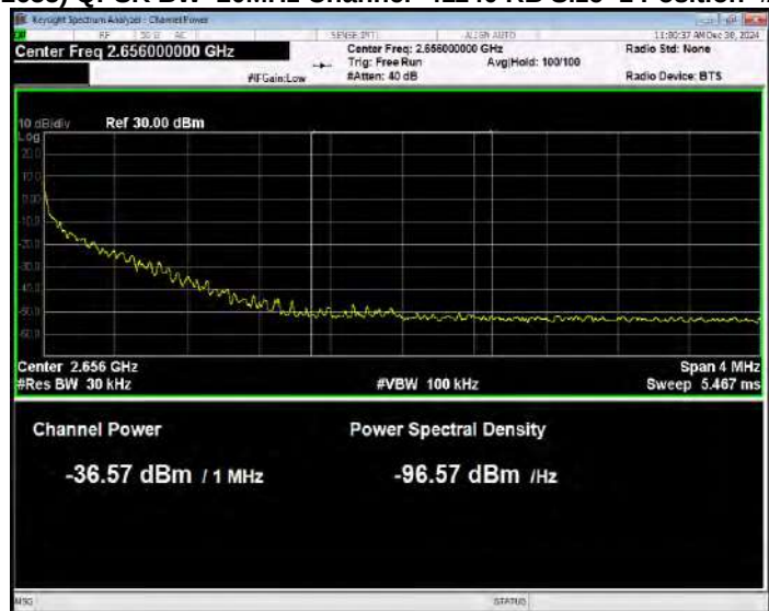
Band41(2535-2655) QPSK BW=20MHz Channel=41140 RB Size=1 Position=#Max Normal
