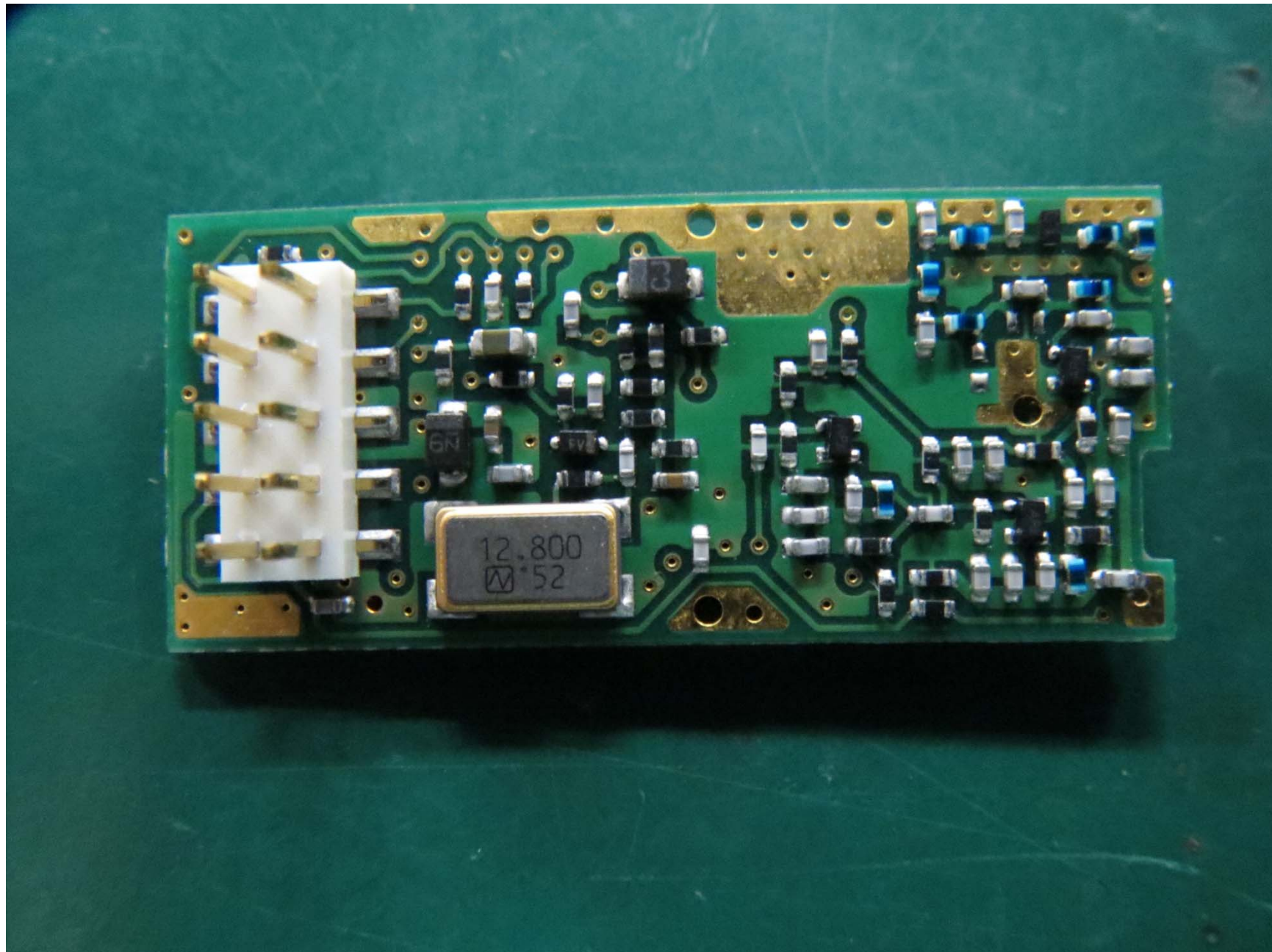
VC0-C6B Bottom (without Shield)
