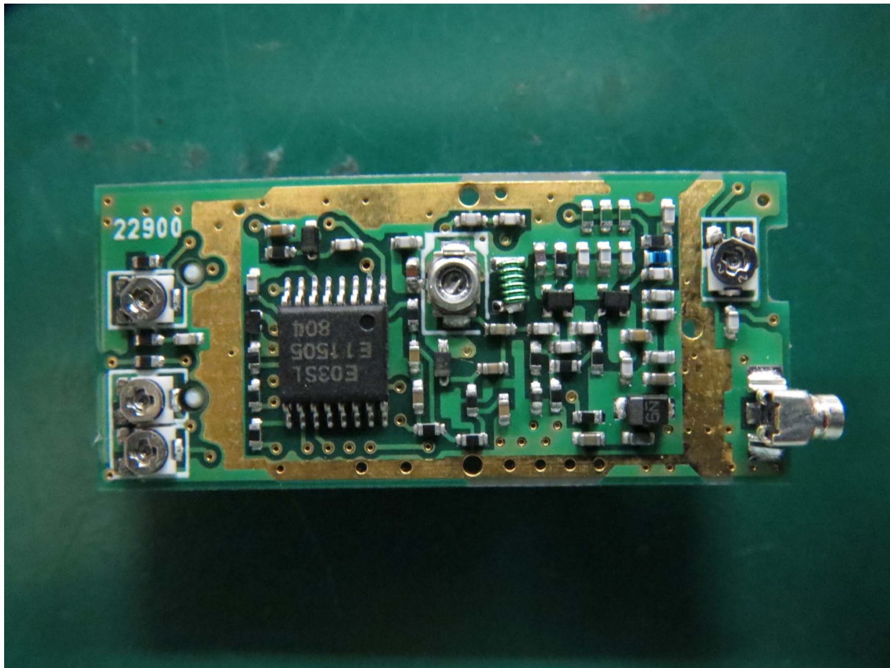
VC0-C6B Top (without Shield)
