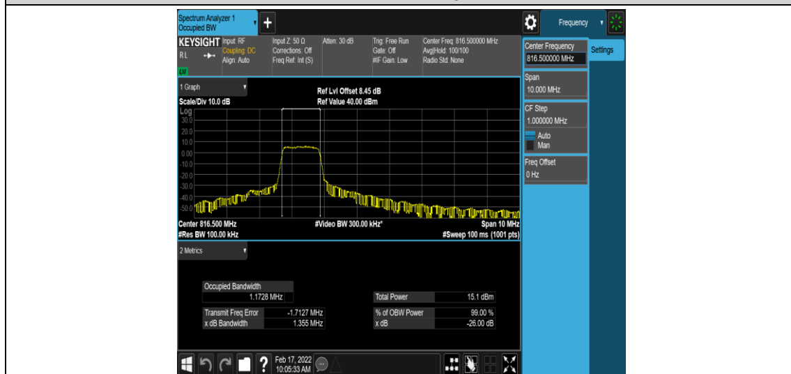
Band26-5MHz-16QAM-26715-6-0-Low-1.1728-1.355-PASS
