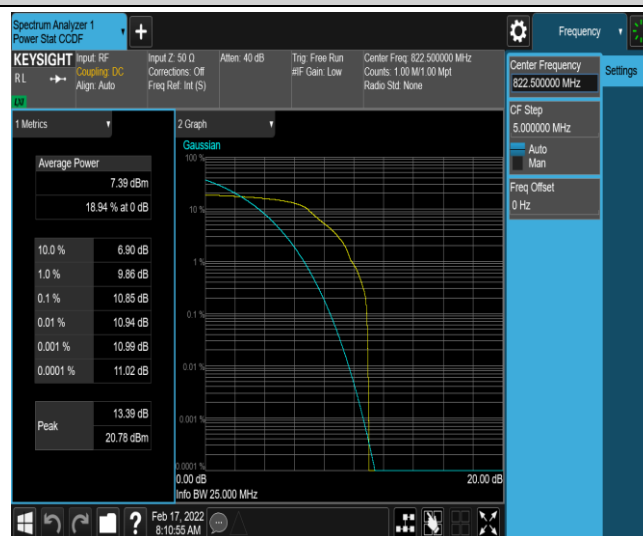
Band26-3MHz-QPSK-26775-1-0-High-10.85-&lt;=13-PASS
