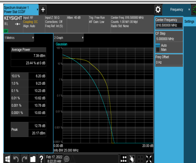
Band26-5MHz-QPSK-26715-6-0-Low-10.23-&lt;=13-PASS
