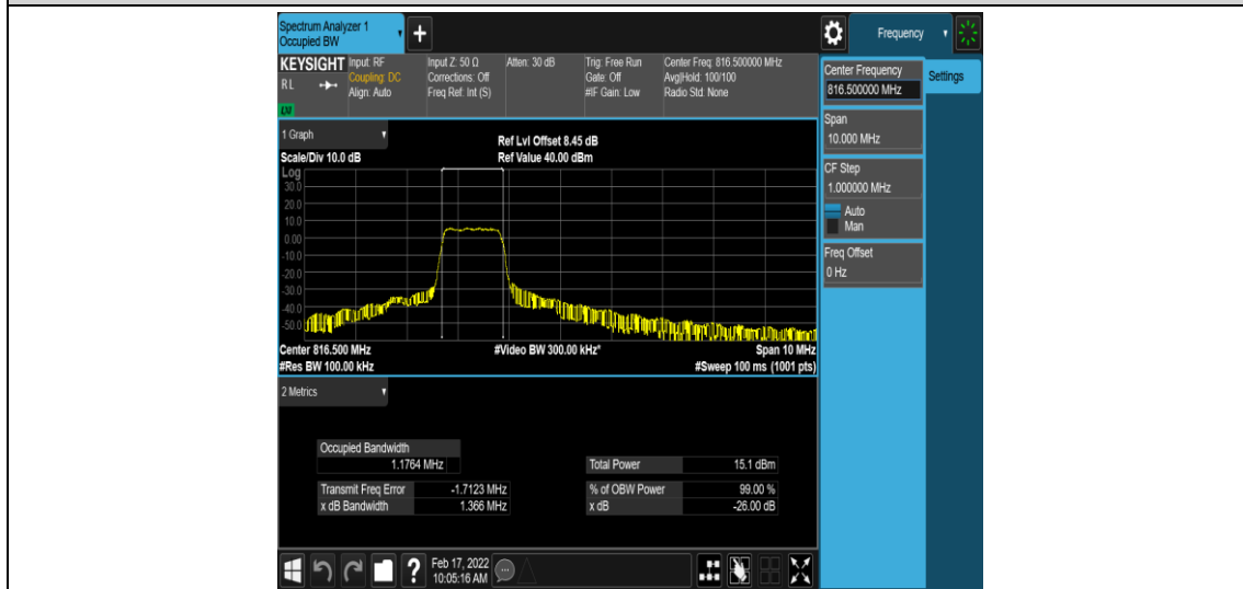
Band26-5MHz-QPSK-26715-6-0-Low-1.1764-1.366-PASS
