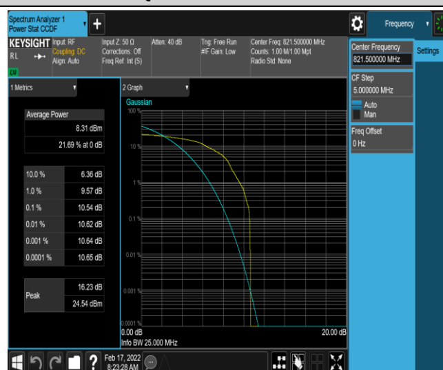
Band26-5MHz-16QAM-26765-1-0-High-10.54-<=13-PASS
