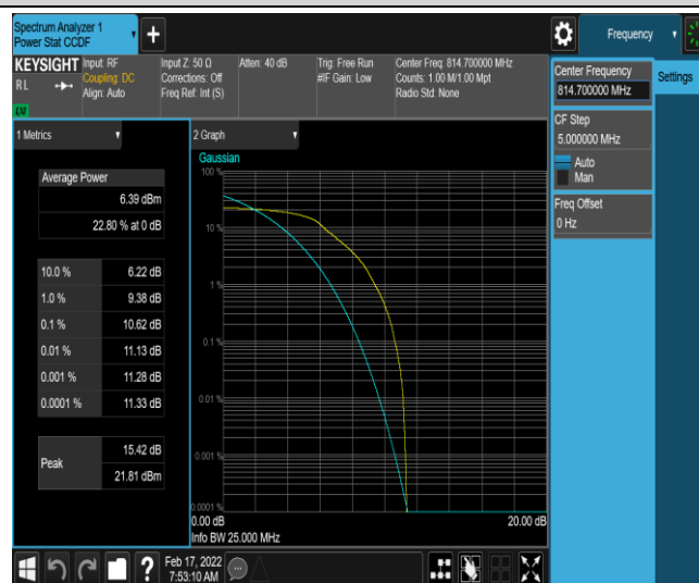
Band26-1.4MHz-16QAM-26697-6-0-Low-10.62-&lt;=13-PASS
