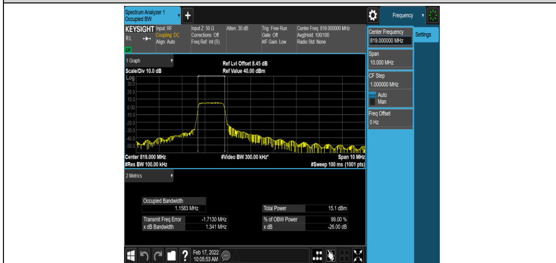
Band26-5MHz-QPSK-26740-6-0-Low-1.1583-1.341-PASS
