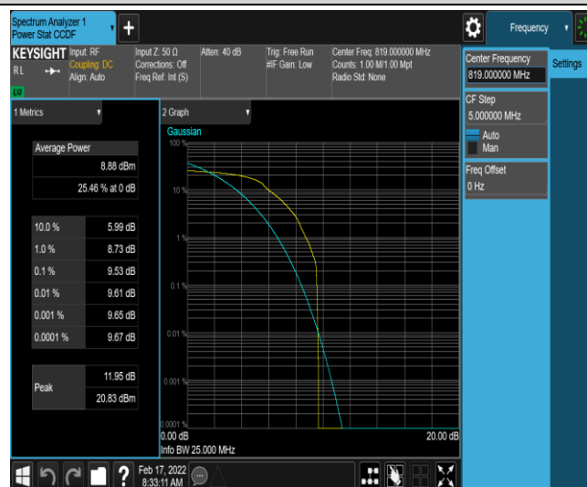
Band26-10MHz-QPSK-26740-1-0-Low-9.53-<=13-PASS
