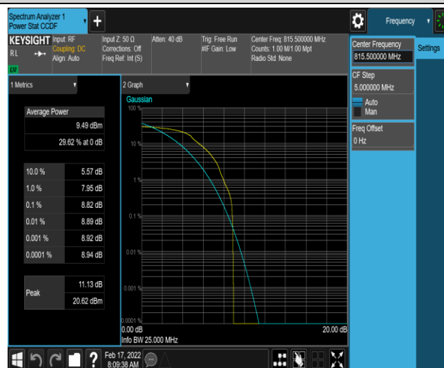
Band26-3MHz-OPSK-26705-1-0-Low-8.82-<=13-PASS
