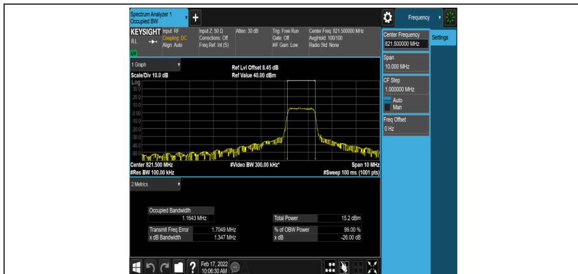
Band26-5MHz-QPSK-26765-6-0-High-1.1643-1.347-PASS
