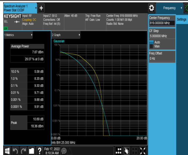
Band26-3MHz-QPSK-26740-6-0-Low-9.30-&lt;=13-PASS
