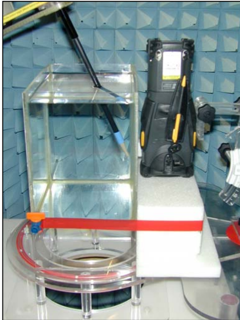
Figure 25. Positional photograph of the MC9060 left-hand side at 1.0cm from Phantom side
