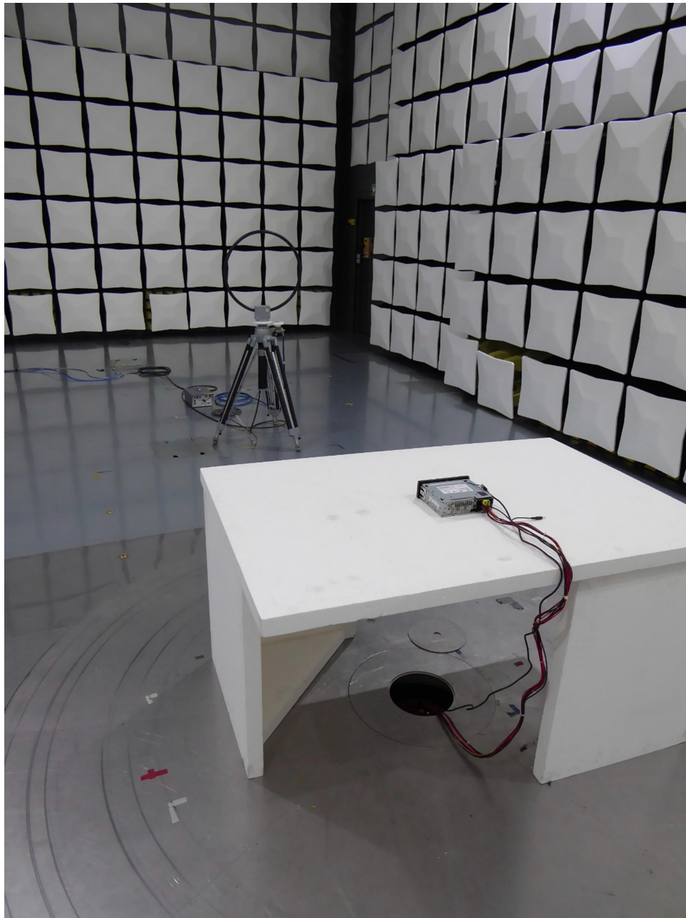
Test setup semi anechoic chamber (9 kHz – 30 MHz) – Pos 1
