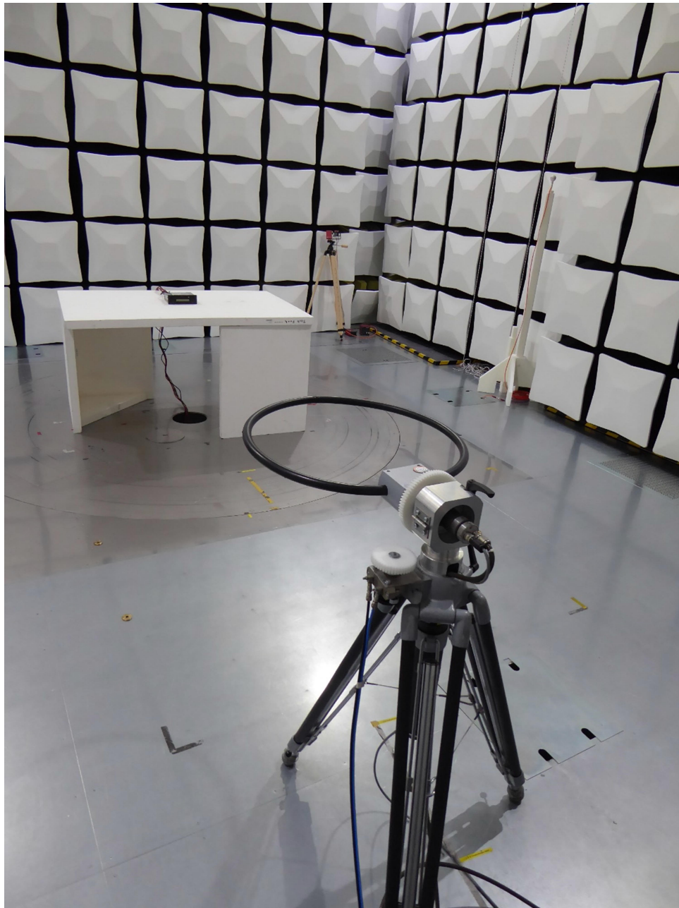
Test setup semi anechoic chamber (9 kHz – 30 MHz) – Pos 3
