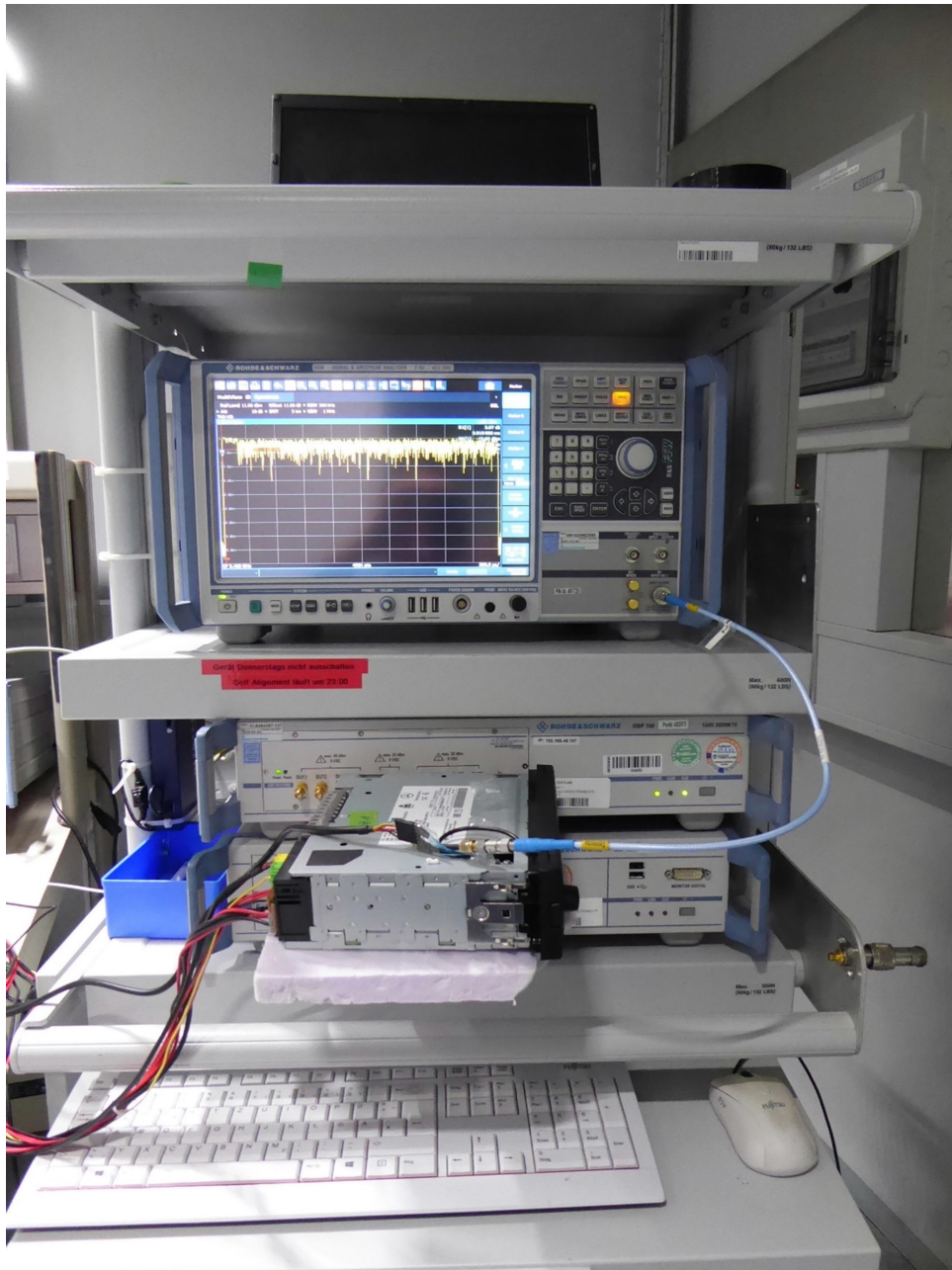
Test setup antenna port conducted at temporary antenna connector
