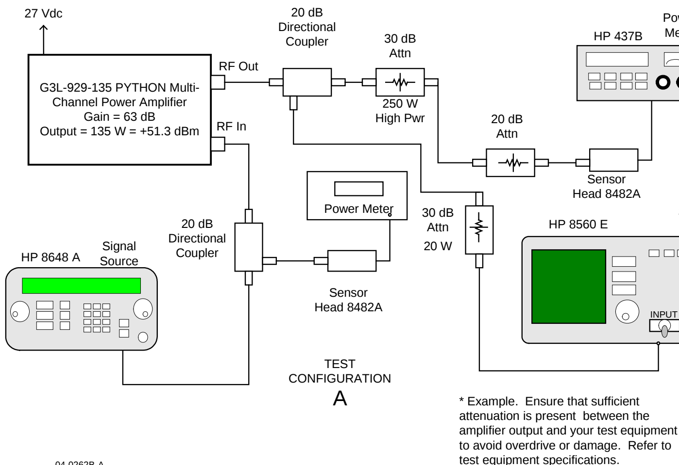
Figure 5-1. Amplifier Test Setup Diagram – Configuration A
