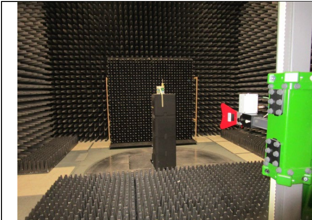
4-18 GHz
