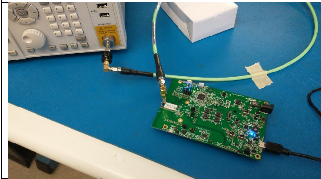
RF Conducted
