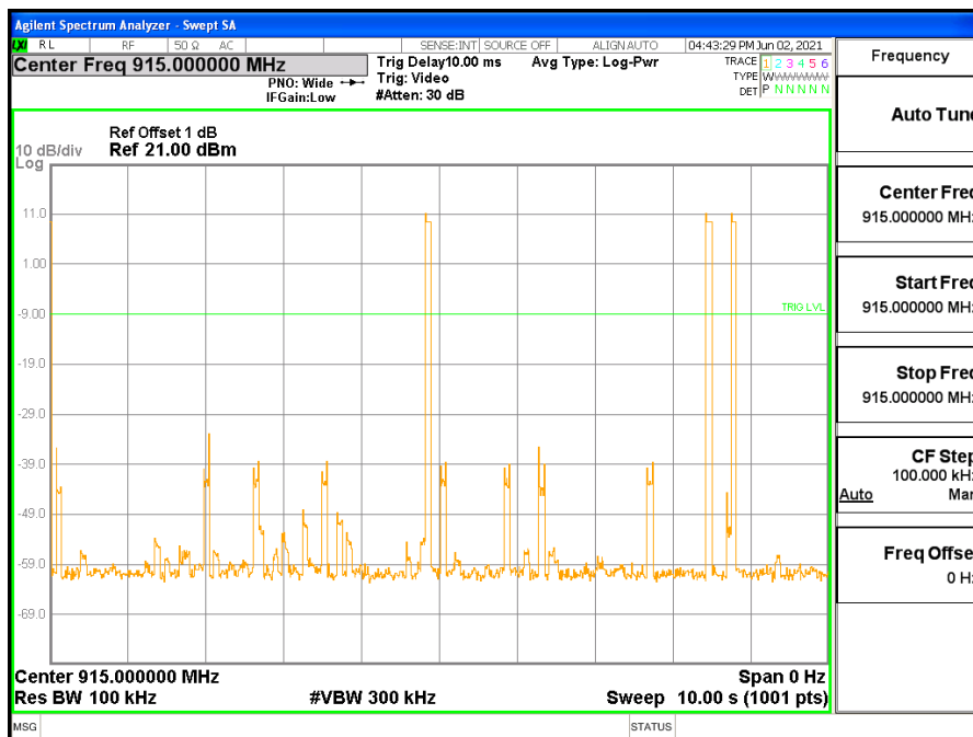
The number of hop channel appear, FSK-250 kbps
