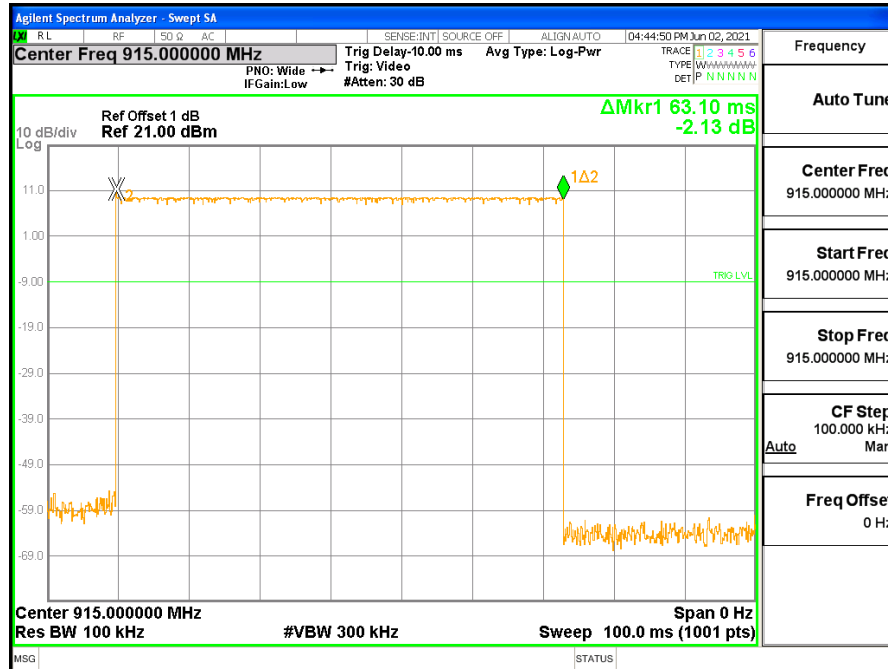
Time of single slot, FSK-250 kbps
