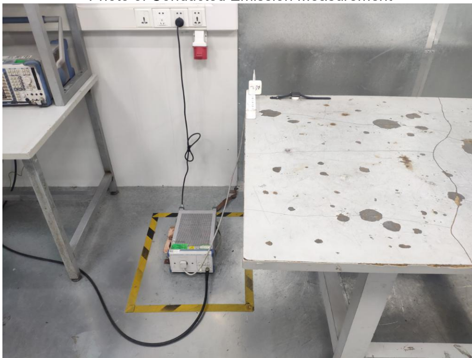
FCC ID: 2AQZHGN373B Photo of Conducted Emission Measurement
