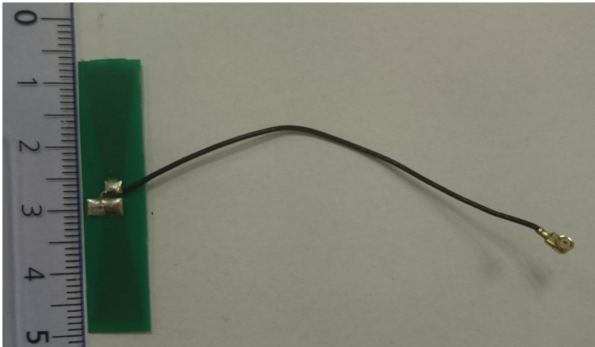
Figure 14 :PCB antenna with UFL connector : bottom
