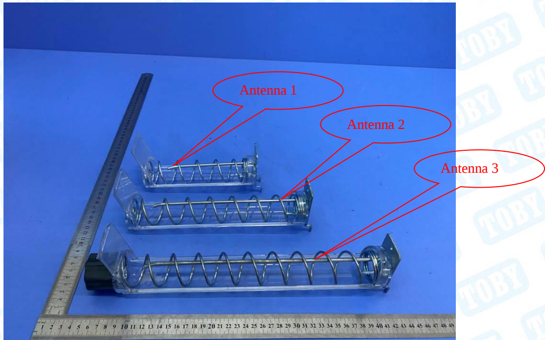
Photo 1 Appearance of EUT
