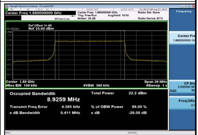
FDD02_MidRange_15_1880_Q16
