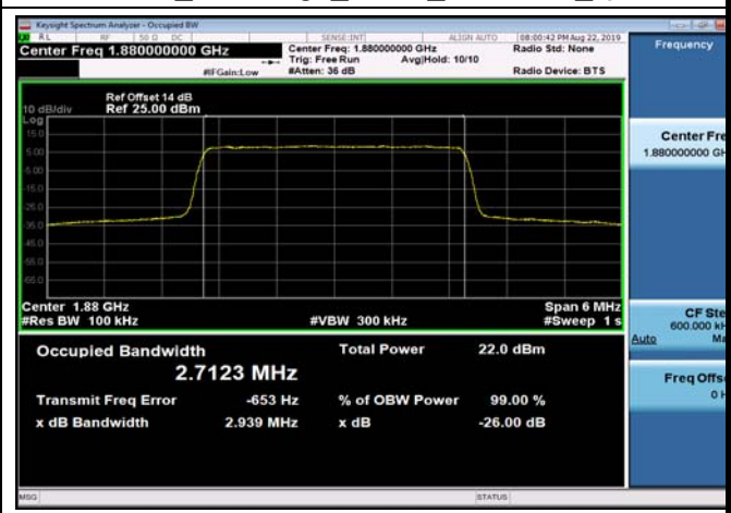
FDD02_MidRange_3MHz_1880MHz_Q16
