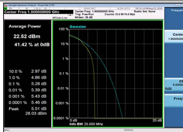
FDD02_HighRange_20MHz_1900_OneRB _high_Q16
