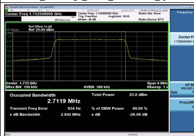
FDD04_MidRange_3MHz_1732.5MHz_QPSK
