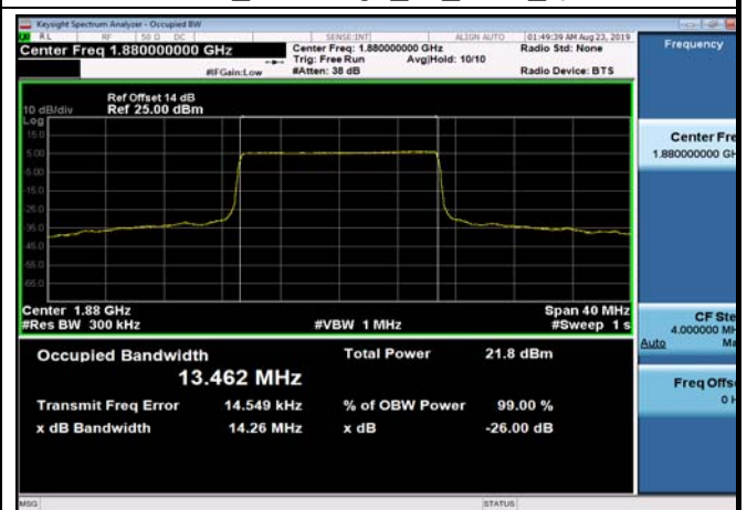
FDD02_MidRange_20_1880_Q16
