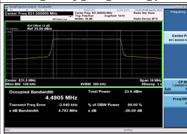
FDD26_MidRange_5MHz_831.5MHz_QPSK
