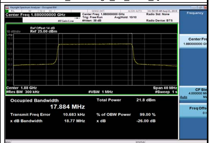
FDD02_MidRange_20_1880_Q16
