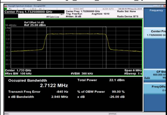
FDD04_MidRange_3MHz_1732.5MHz_Q16
