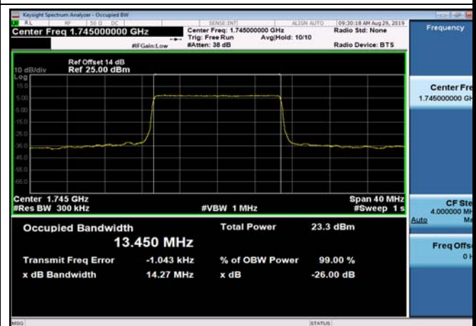
FDD66_MidRange_15_1745_QPSK
