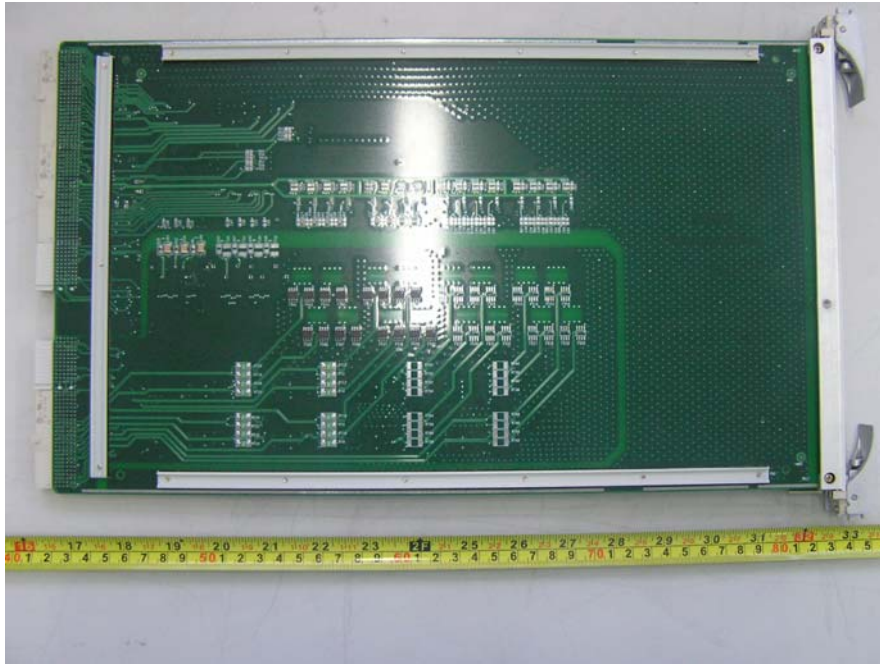
CCMO Top View
