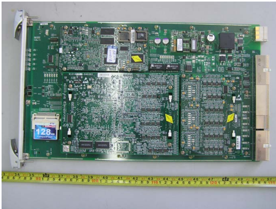
CCM1 Top View
