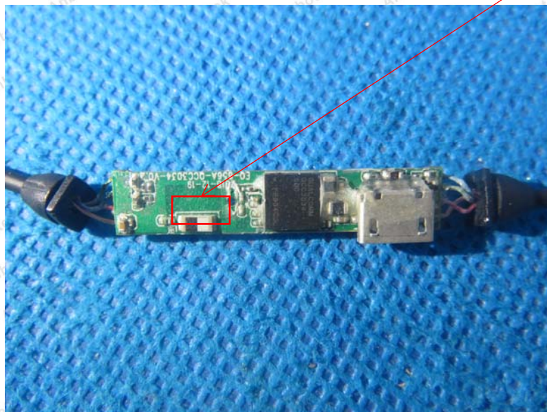
BT Antenna
