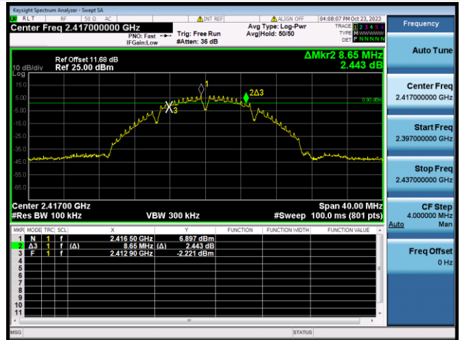
802.11b CHANNEL 2
