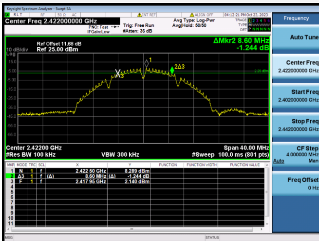
802.11b CHANNEL 3
