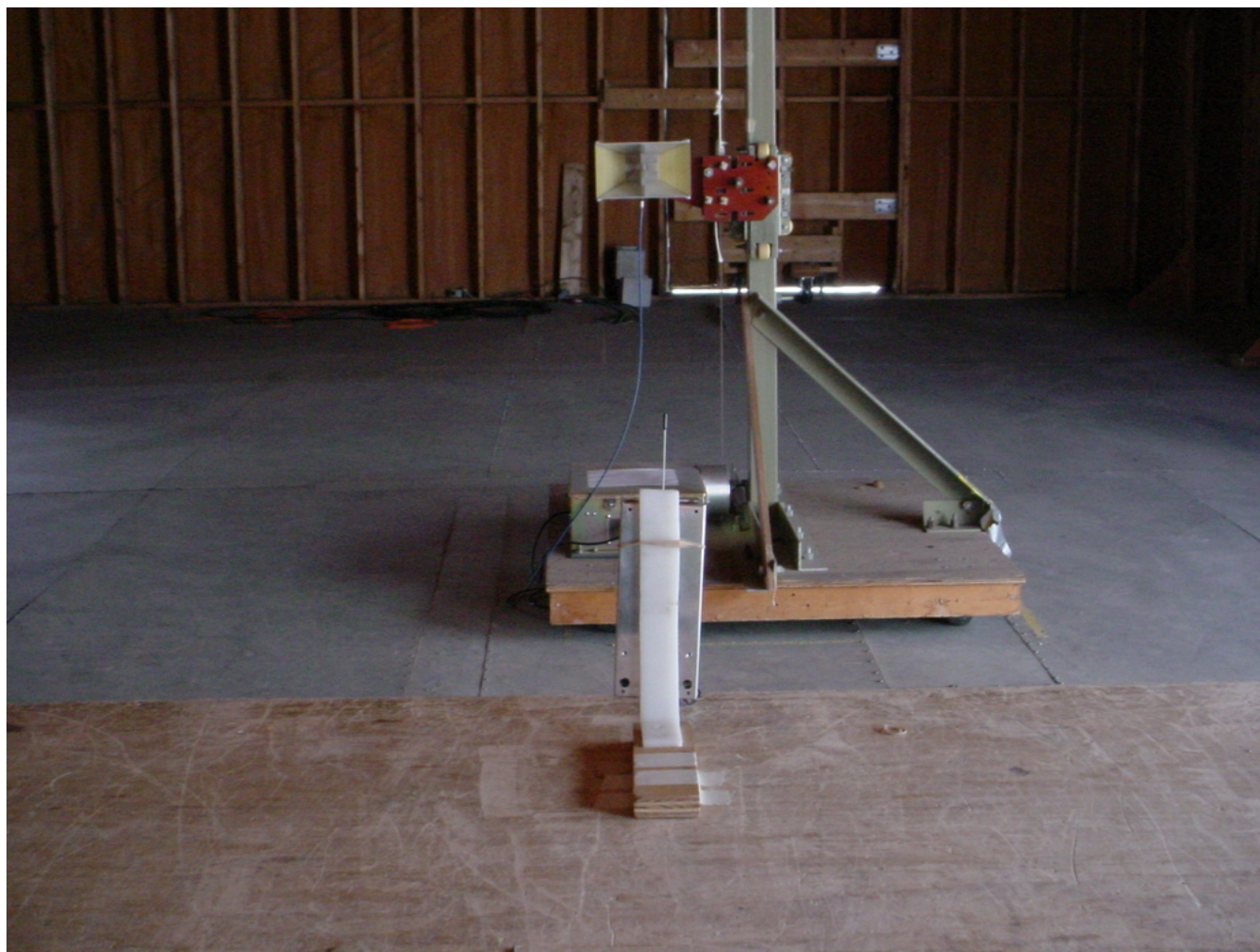
Transmitter Radiated Emissions @ 3 meters Orthogonal Position # 3
