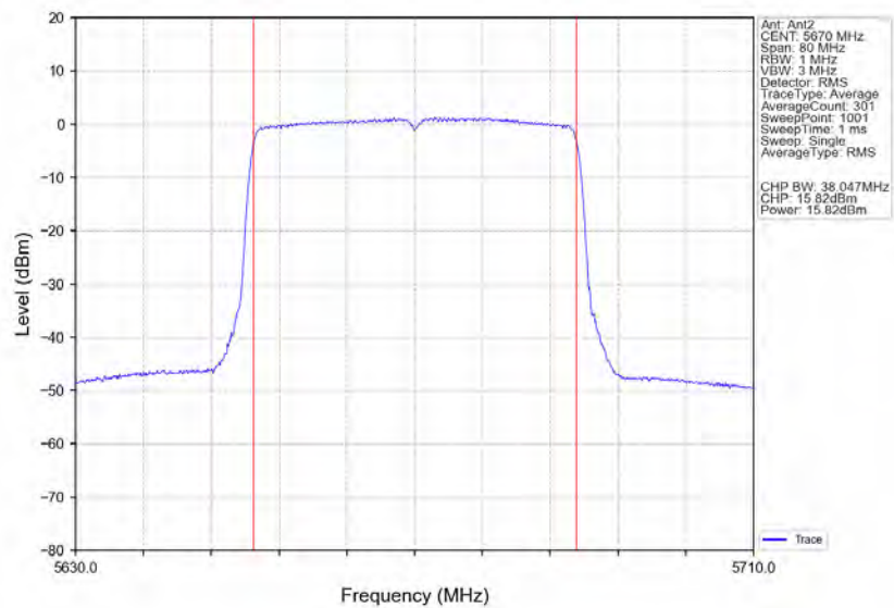
802.11ax(HEW40)_HCH_5670MHz_RU484_Left_Ant2_NTNV
