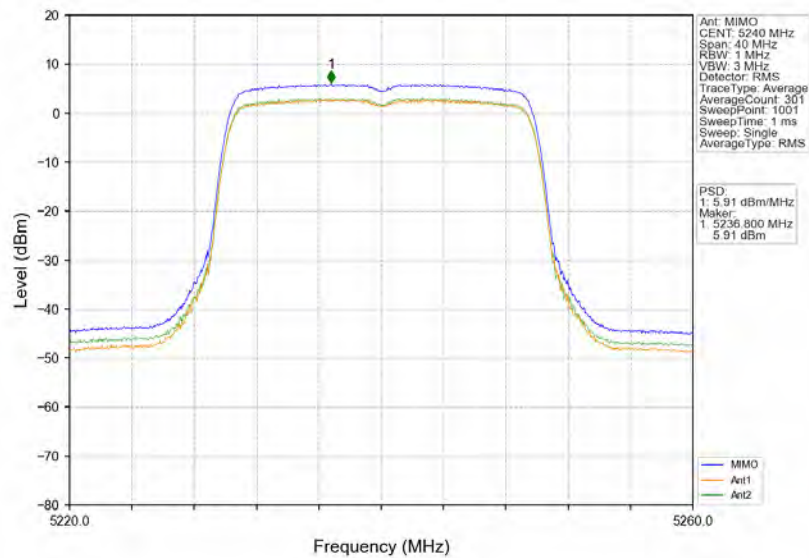
802.11ax(HEW20)_HCH_5240MHz_RU242_Left_MIMO_NTNV
