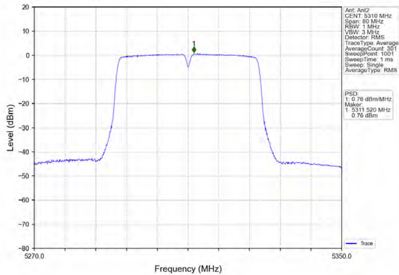
802.11n(HT40)_HCH_5310MHz_MIMO_NTNV
