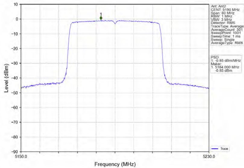
802.11ax(HEW40)_LCH_5190MHz_RU484_Left_MIMO_NTNV
