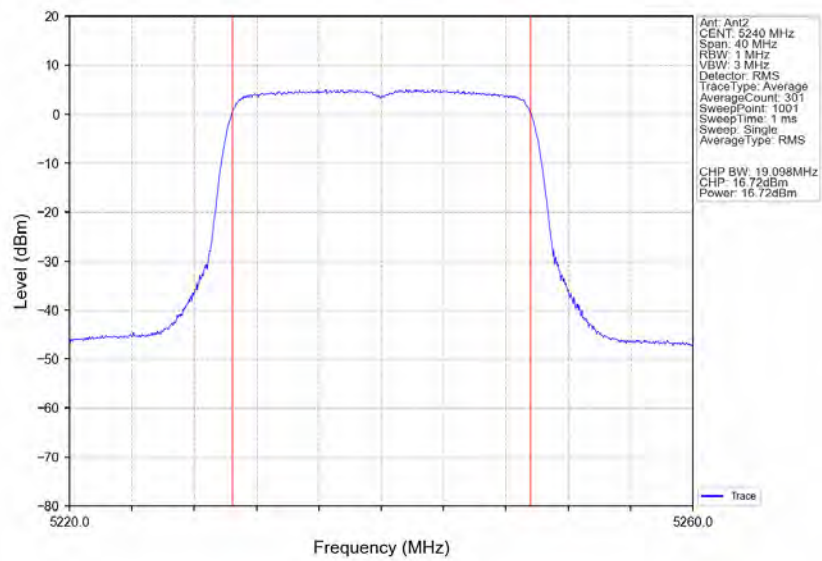
802.11ax(HEW20)_HCH_5240MHz_RU242_Left_Ant2_NTNV
