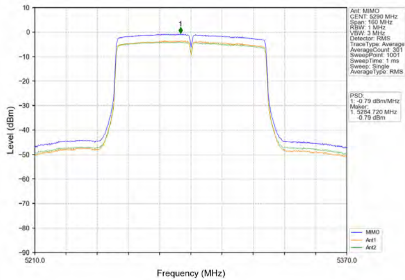
802.11ac(VHT80)_MCH_5290MHz_MIMO_NTNV
