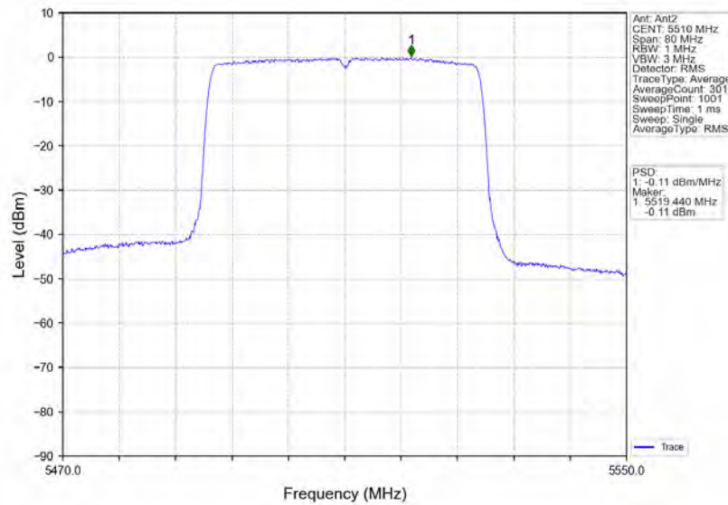
802.11ax(HEW40)_LCH_5510MHz_RU484_Left_MIMO_NTNV
