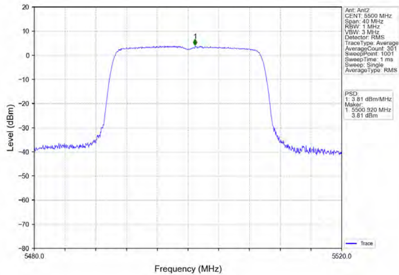
802.11ax(HEW20)_LCH_5500MHz_RU242_Left_MIMO_NTNV
