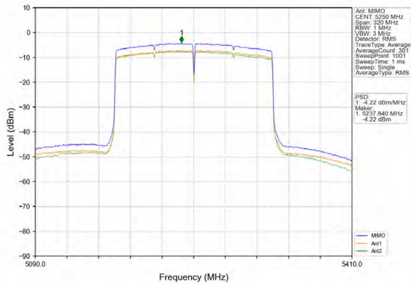
802.11ax(HEW160)_MCH_5250MHz_2xRU996_Left_MIMO_NTNV
