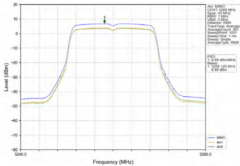
802.11n(HT20)_LCH_5260MHz_MIMO_NTNV
