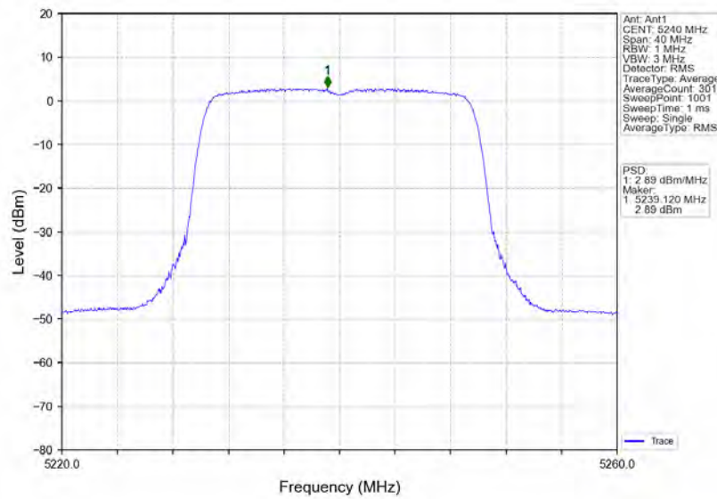
802.11ax(HEW20)_HCH_5240MHz_RU242_Left_Ant1_NTNV
