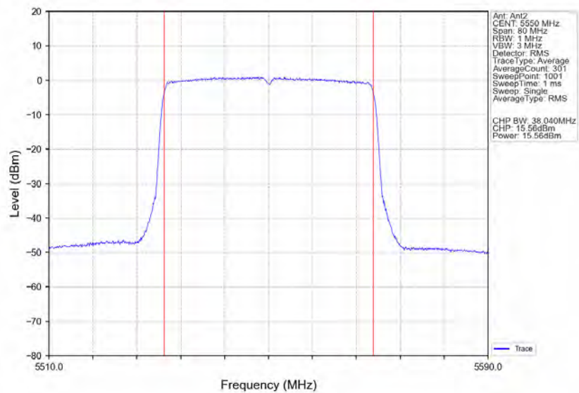
802.11ax(HEW40)_MCH_5550MHz_RU484_Left_Ant2_NTNV
