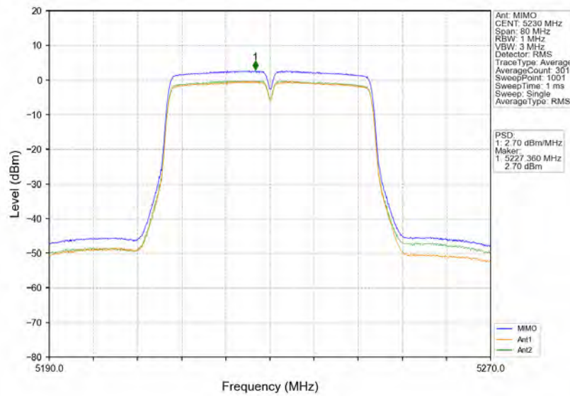
802.11n(HT40)_HCH_5230MHz_MIMO_NTNV
