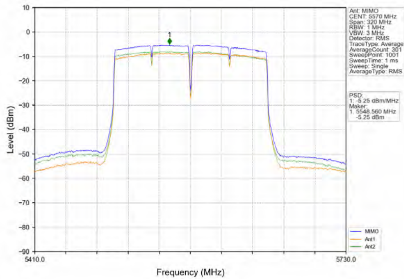
802.11ac(VHT160)_MCH_5570MHz_MIMO_NTNV
