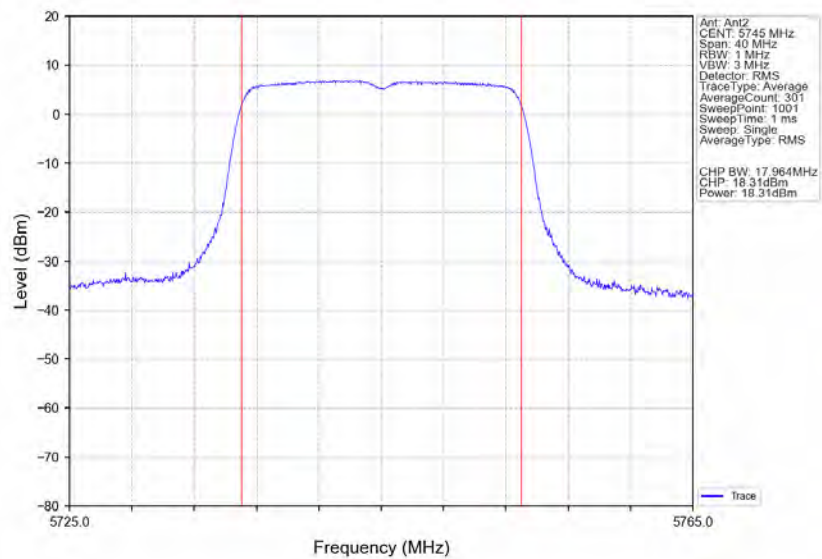
802.11n(HT20)_LCH_5745MHz_Ant2_NTNV
