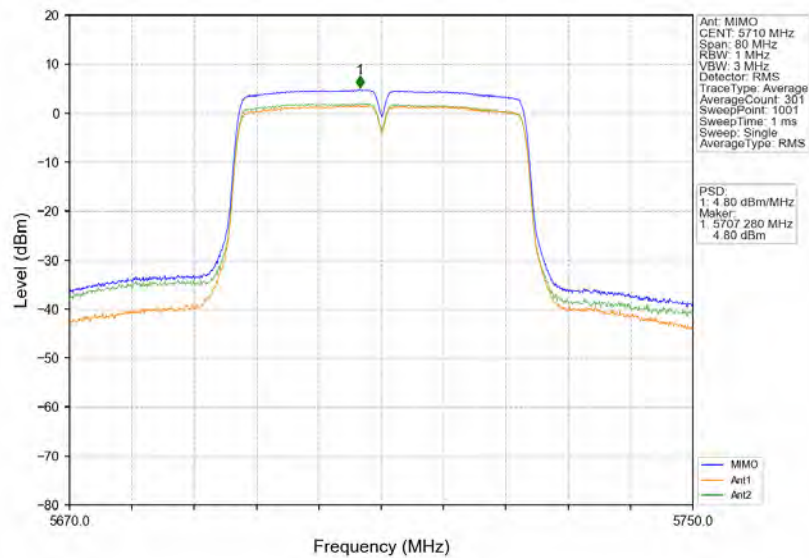
802.11n(HT40)_HCH_5710MHz_MIMO_NTNV
