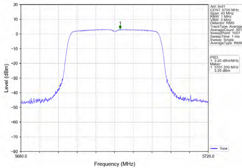
802.11ax(HEW20)_HCH_5700MHz_RU242_Left_Ant1_NTNV
