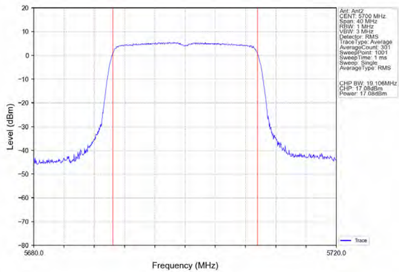
802.11ax(HEW20)_HCH_5700MHz_RU242_Left_Ant2_NTNV
