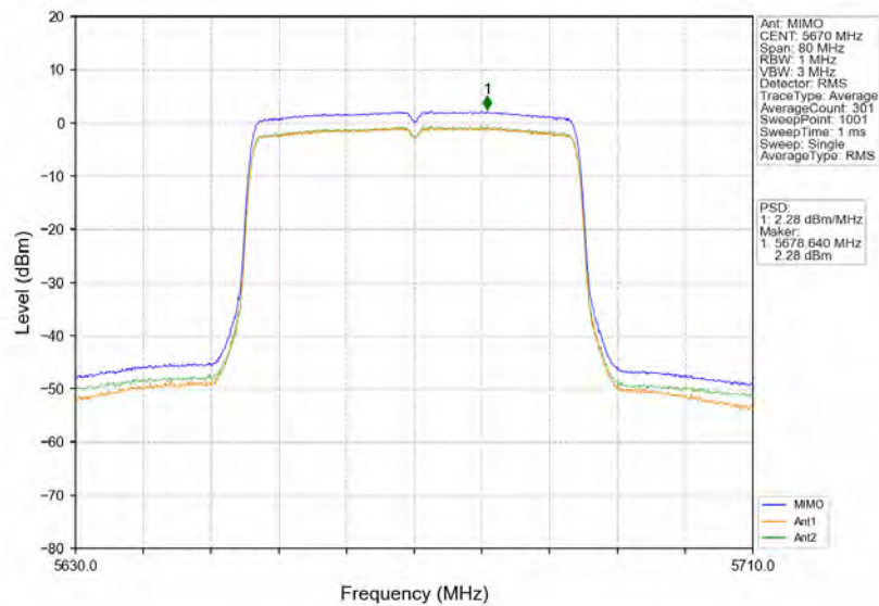
802.11ax(HEW40)_HCH_5670MHz_RU484_Left_MIMO_NTNV
