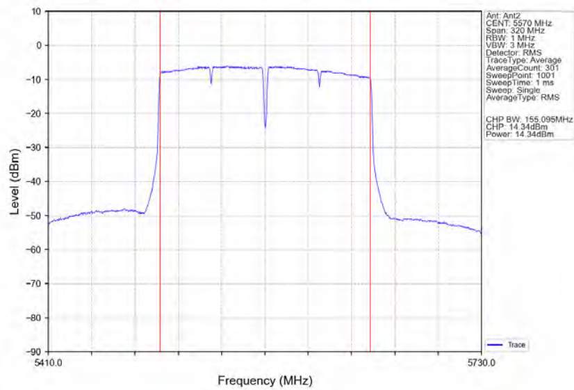
802.11ac(VHT160)_MCH_5570MHz_Ant2_NTNV
