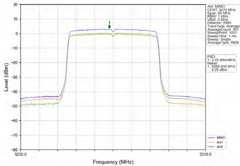
802.11ax(HEW40)_LCH_5270MHz_RU484_Left_MIMO_NTNV
