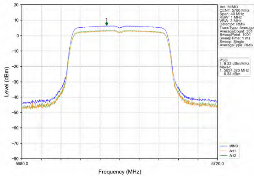
802.11ax(HEW20)_HCH_5700MHz_RU242_Left_MIMO_NTNV
