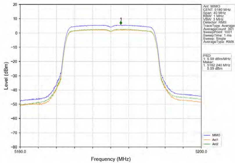
802.11ax(HEW20)_LCH_5180MHz_RU242_Left_MIMO_NTNV
