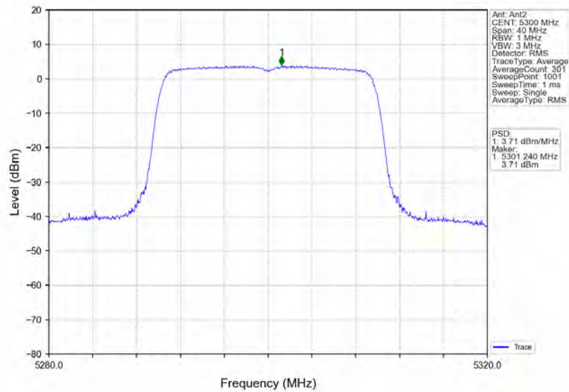
802.11ax(HEW20)_MCH_5300MHz_RU242_Left_MIMO_NTNV
