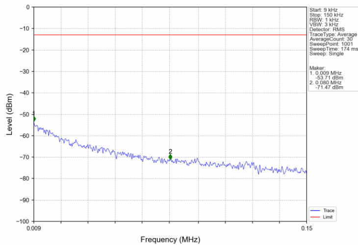
Band66_10MHz_QPSK_LCH_1715MHz_RB_1_0_NTNV
