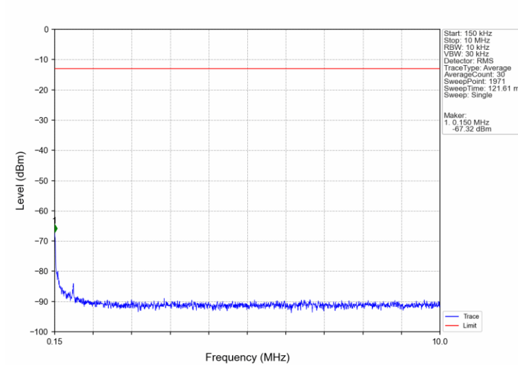
Band66_10MHz_16QAM_MCH_1745MHz_RB_1_0_NTNV
