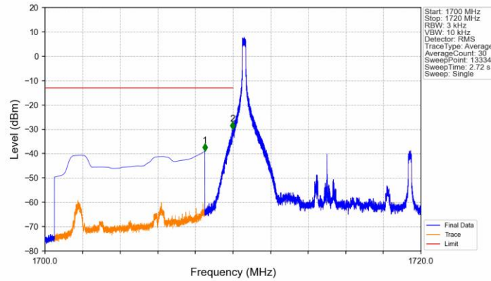
Band66_10MHz_QPSK_LCH_1715MHz_RB_1_0_NTNV
