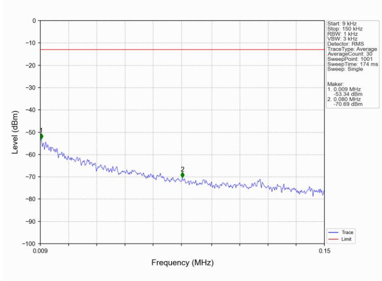
Band66_10MHz_16QAM_MCH_1745MHz_RB_1_0_NTNV
