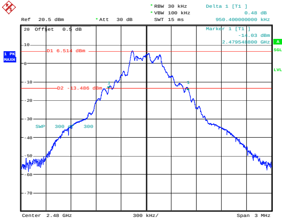
GFSK_High 0.950MHz
