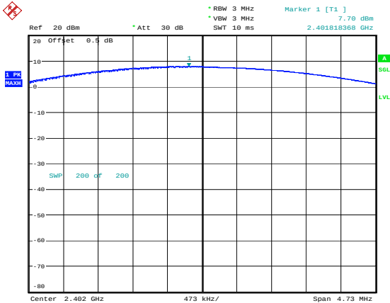
GFSK_Low 7.70dBm
