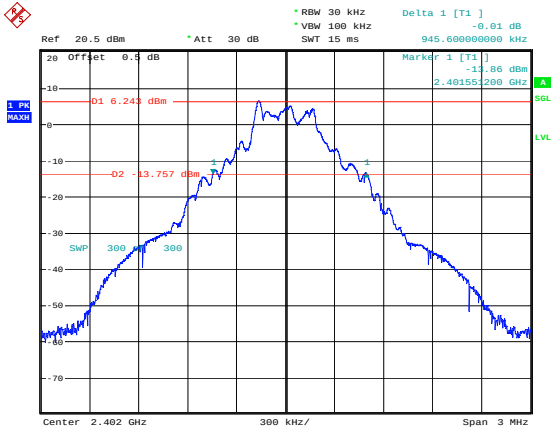
GFSK_Low 0.946MHz
