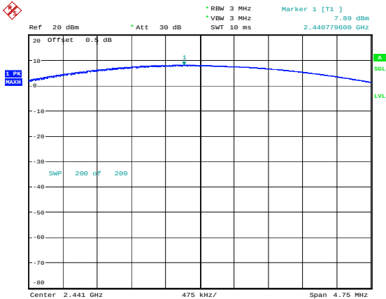
GFSK_Middle 7.89dBm
