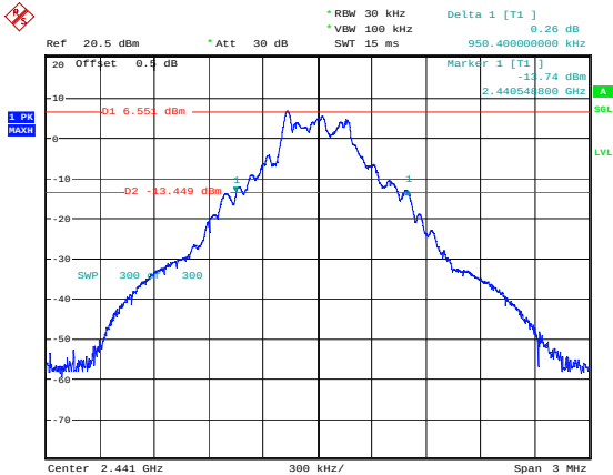
GFSK_Middle 0.950MHz
