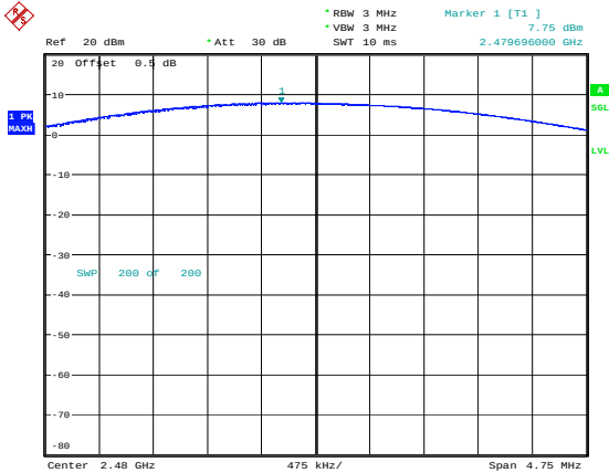
GFSK_High 7.75dBm
