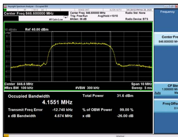
(Plot E3: WCDMA 850MHz Channel = 4233 Occupied bandwidth)
