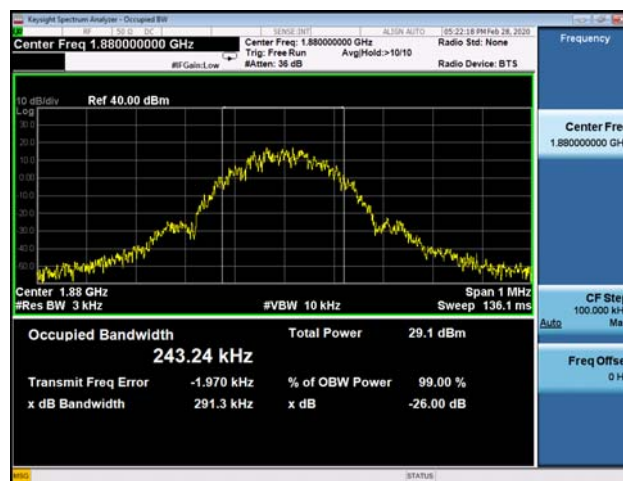
(Plot D2: EDGE 1900MHz Channel = 661 Occupied bandwidth)
