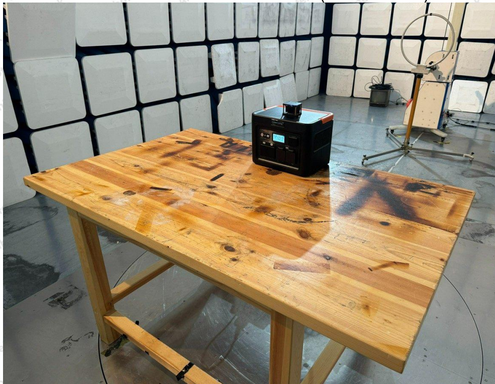
Photo of Radiation Emission Test (below 30MHz)
