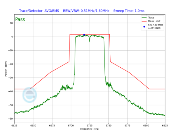
Plot 7-568. SP In-Band Emission Plot Antenna WF7a (40MHz 802.11ax RU484 (UNII Band 7) – Ch. 155)
