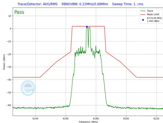
Plot 7-514. SP In-Band Emission Plot Antenna WF8 (20MHz 802.11ax RU26 (UNII Band 5) – Ch. 45)
