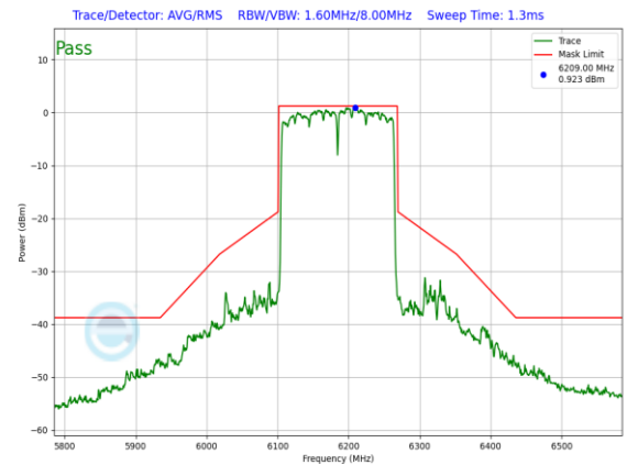
Plot 7-560. SP In-Band Emission Plot Antenna WF7a (160MHz 802.11ax RU996x2 (UNII Band 5) – Ch. 47)
