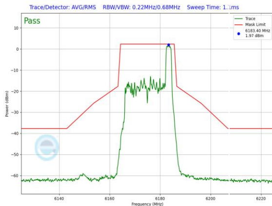
Plot 7-515. SP In-Band Emission Plot Antenna WF8 (20MHz 802.11ax RU26 (UNII Band 5) – Ch. 45)
