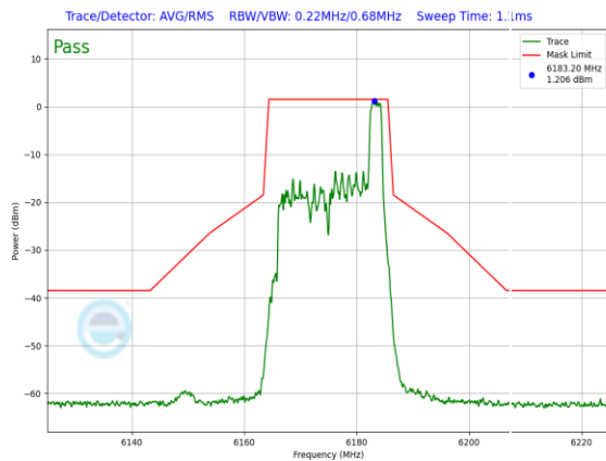
Plot 7-547. SP In-Band Emission Plot Antenna WF7a (20MHz 802.11ax RU26 (UNII Band 5) – Ch. 45)
