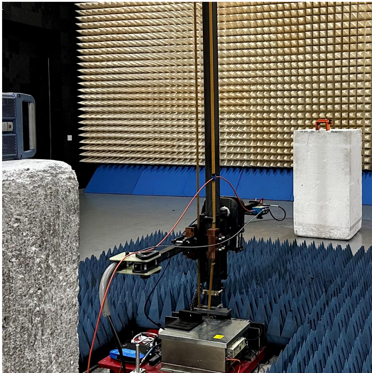
Spurious Emissions, 18GHz – 40GHz
