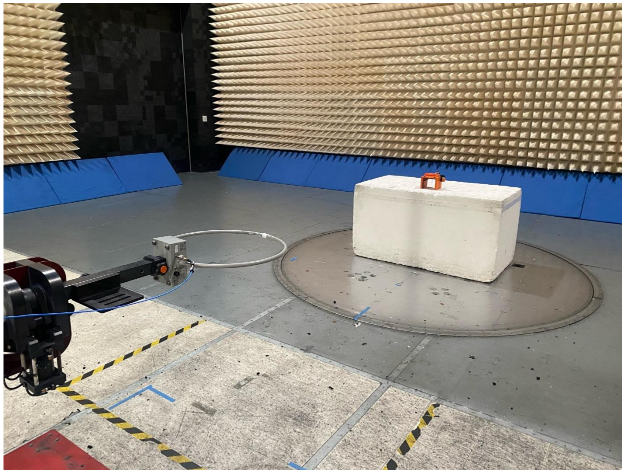
Spurious Emissions, 9kHz – 30MHz
