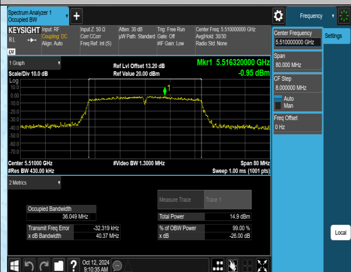
11AC40SISO-Ant2-5510
