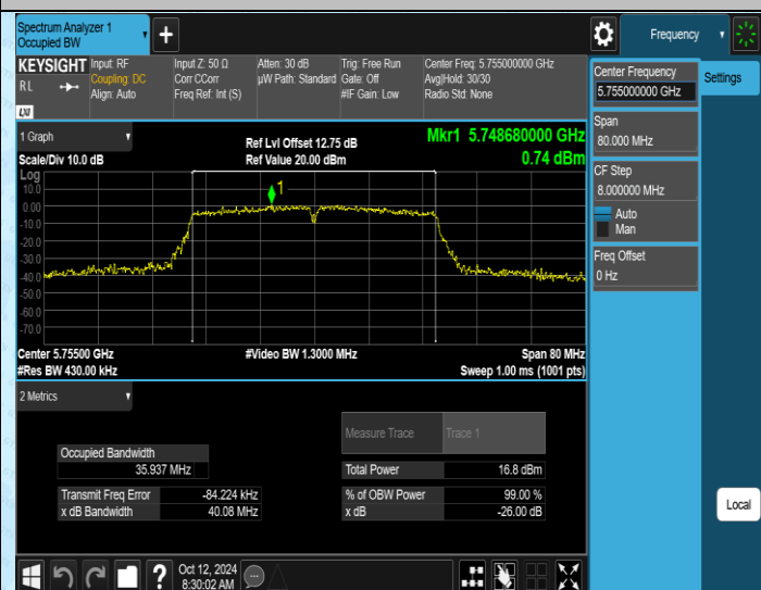
11N40SISO-Ant2-5755
