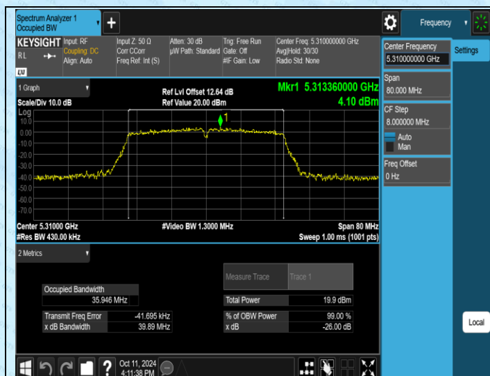
11AC40SISO-Ant1-5310
