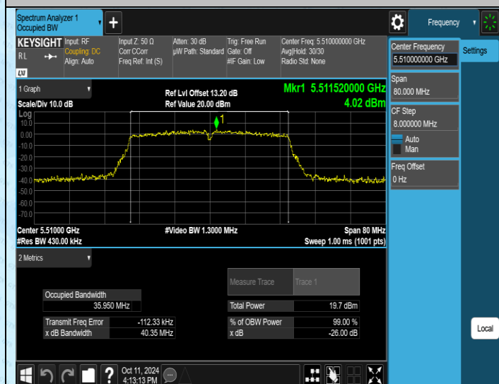
11AC40SISO-Ant1-5510
