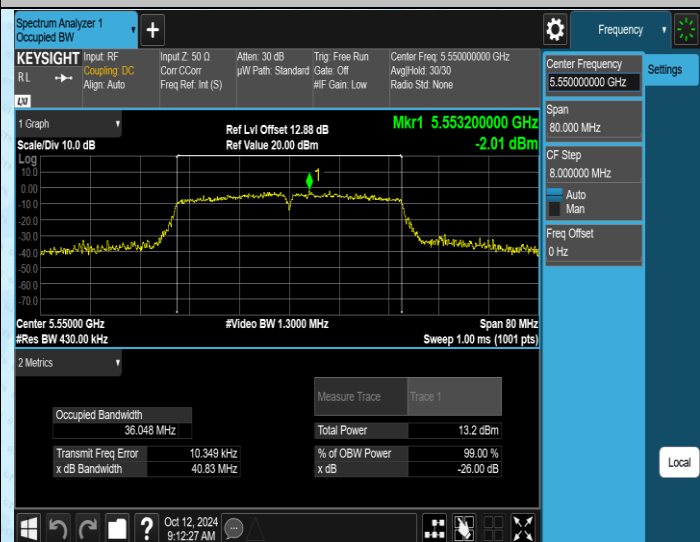
11AC40SISO-Ant2-5550
