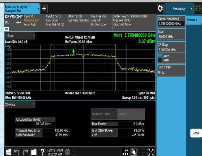
11N40SISO-Ant2-5795
