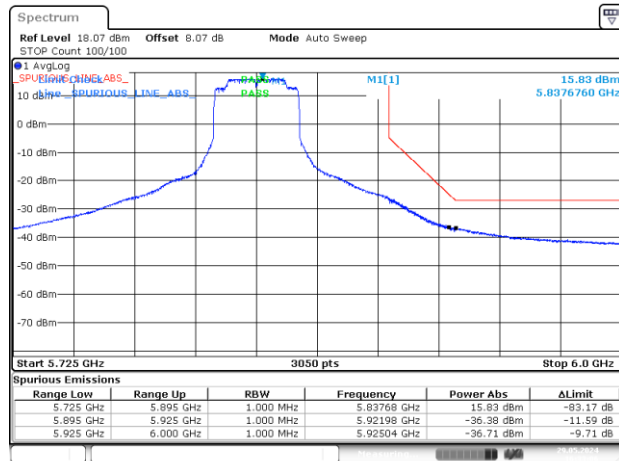
BE-NR-HIGH, SISO-A, 802.11ax/be40-MCS0, Ch167
