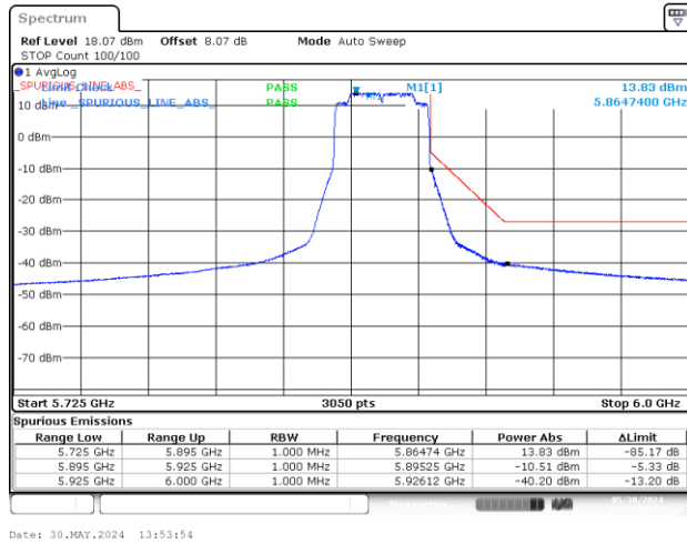
BE-NR-HIGH, SISO-B, 802.11ax/be40-MCS0, Ch175
