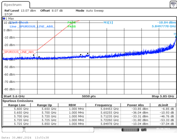
BE-NR-LOW, SISO-B, 802.11ax/be40-MCS0, Ch175
