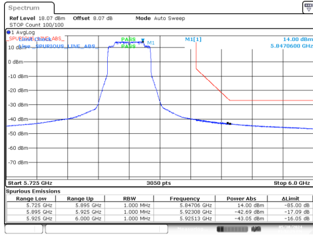
BE-NR-HIGH, SISO-B, 802.11ax/be40-MCS0, Ch167
