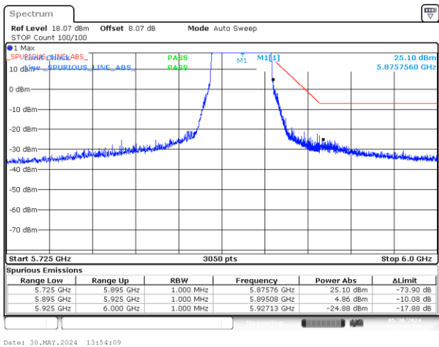
BE-NR-HIGH-PEAK, SISO-B, 802.11ax/be40-MCS0, Ch175
