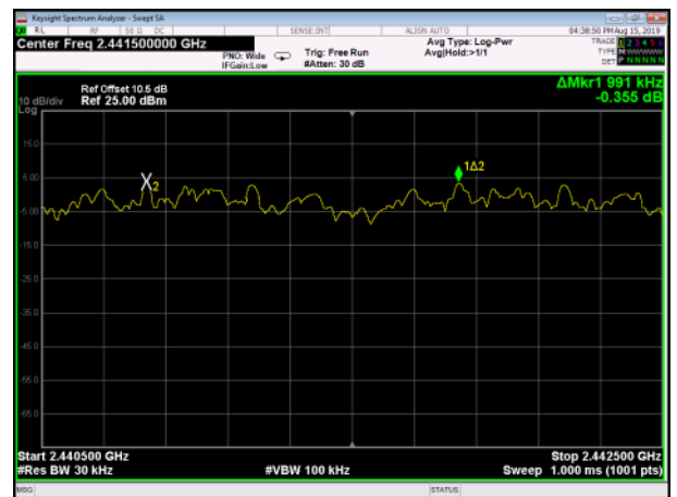
8DPSK,Hopping3DH5,2440.5~2442.5
