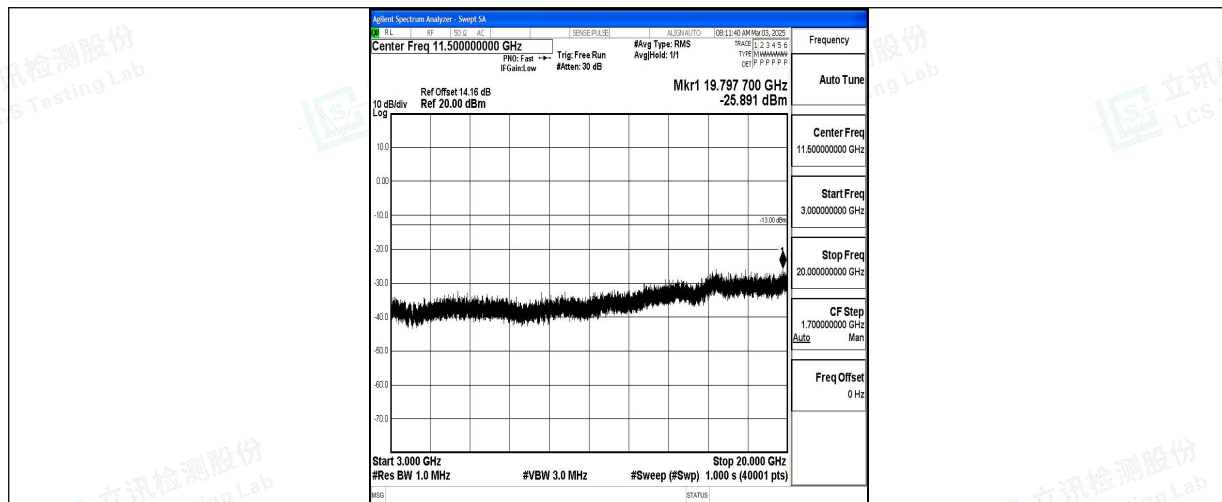
Band66_1.4MHz_QPSK_131979_1RB#0_3000~20000_3000~20000
