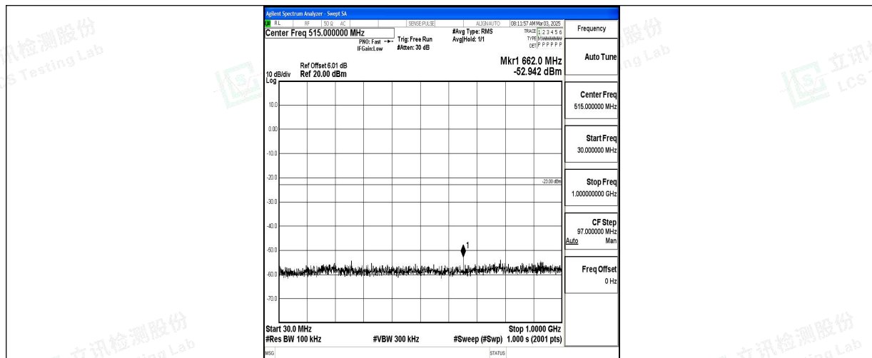
Band66_1.4MHz_16QAM_131979_1RB#0_30~1000_30~1000
