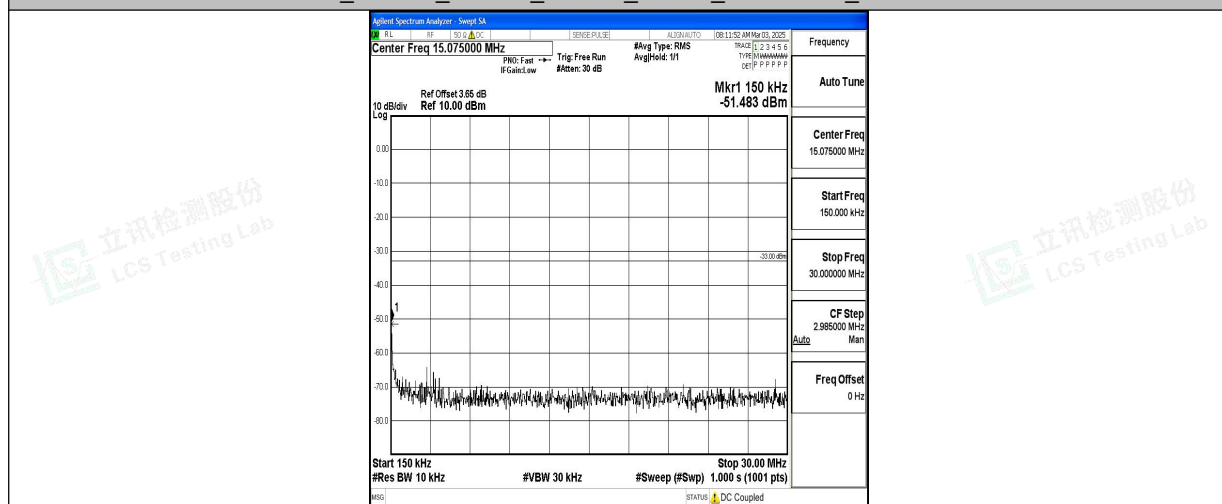
Band66_1.4MHz_16QAM_131979_1RB#0_0.15~30_0.15~30
