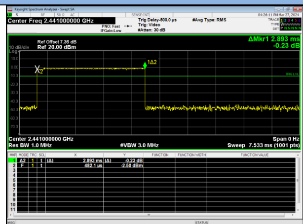
π/4-DQPSK / 2-DH5
