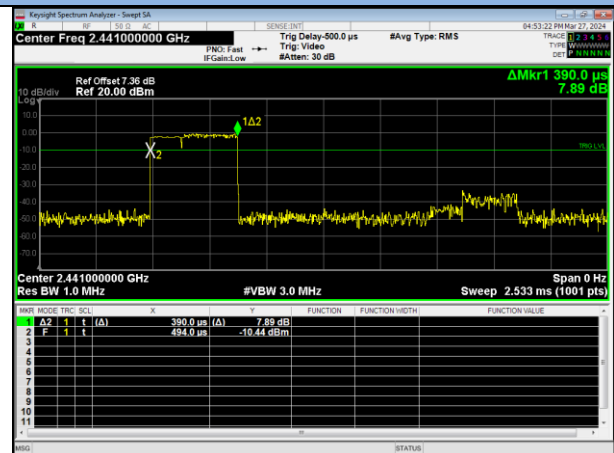
π/4-DQPSK / 2-DH5
