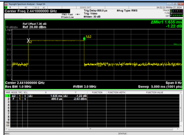
π/4-DQPSK / 2-DH1
