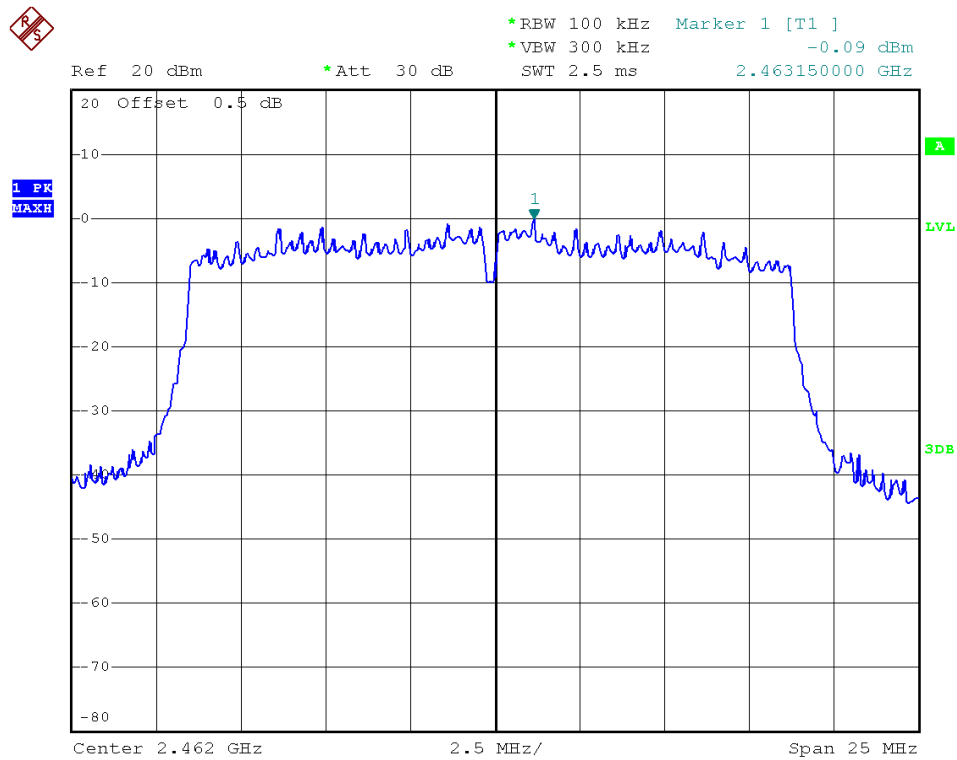
802.11n20 - Channel 11
