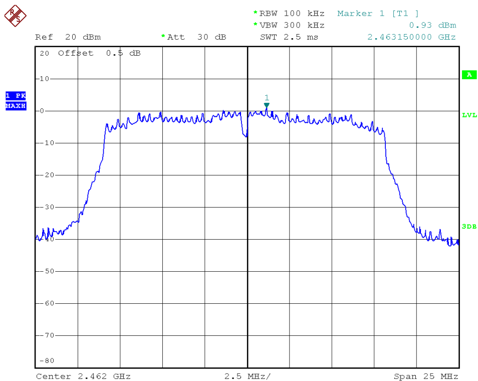
802.11g - Channel 11
