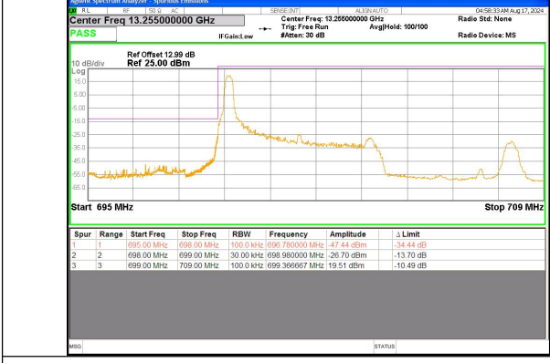
Band 12 5MHz/701.5/Low QPSK 1@0
