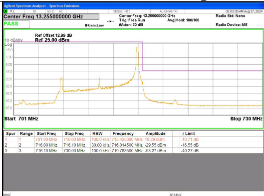
Band 12 10MHz/711.0/High QPSK 1@49
