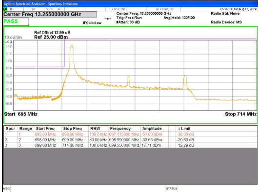
Band 12 10MHz/704.0/Low 16QAM 1@0
