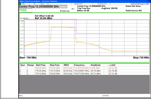
Band 12 5MHz/713.5/High QPSK 25@0
