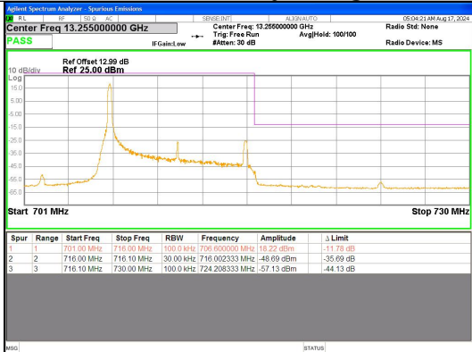
Band 12 10MHz/711.0/High 16QAM 1@0
