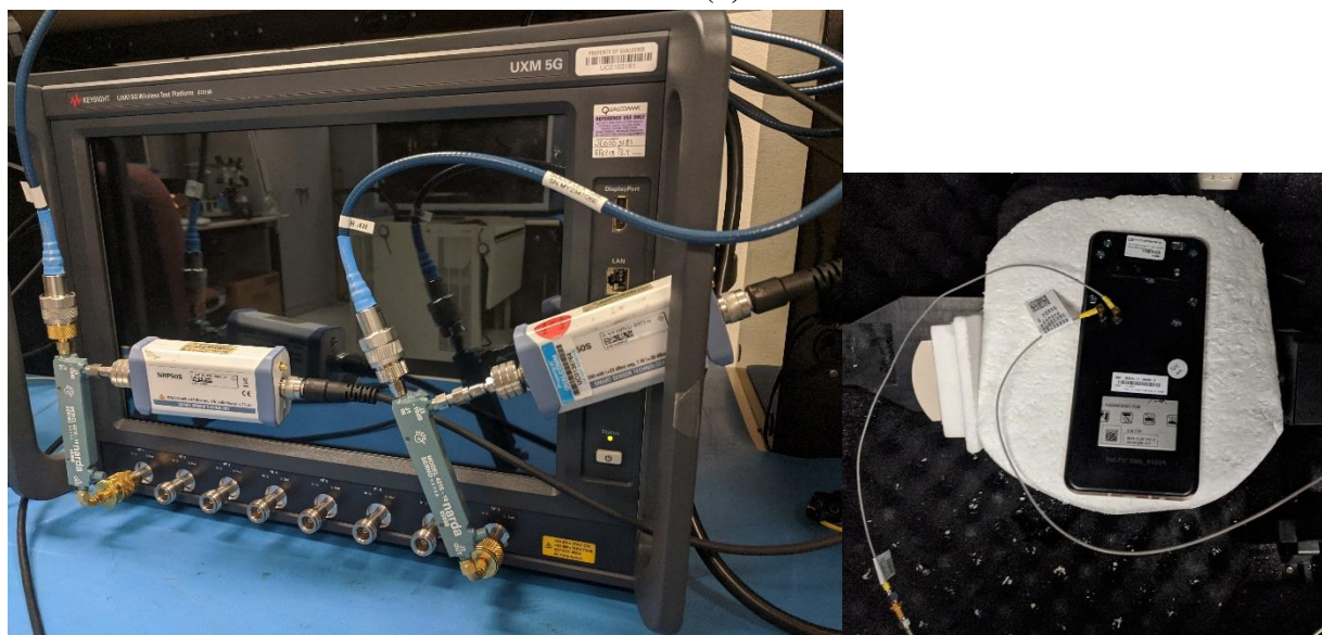
Figure 5-1 Conducted power measurement setup
