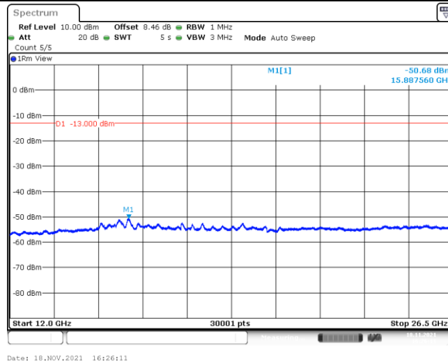
Band8-1.4MHz-QPSK-21648-1-5-Low-30-1000--35.96-PASS
