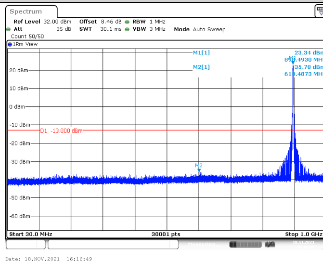
Band8-1.4MHz-16QAM-21632-6-0-Low-1000-5000--41.34-PASS
