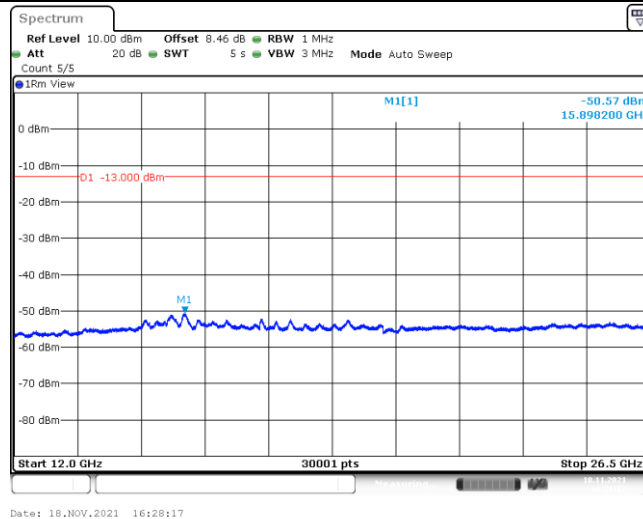
Band8-1.4MHz-16QAM-21648-1-5-Low-30-1000--36.55-PASS
