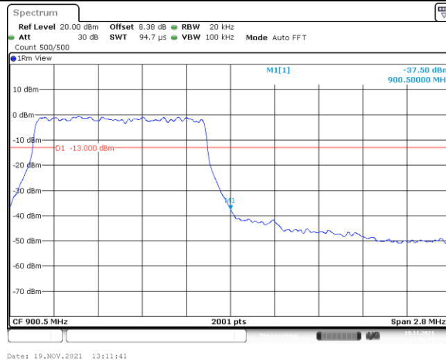
Band8-1.4MHz-16QAM-21632-1-0-Low--29.61-PASS
