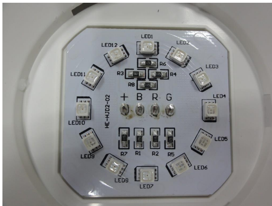
LED module
