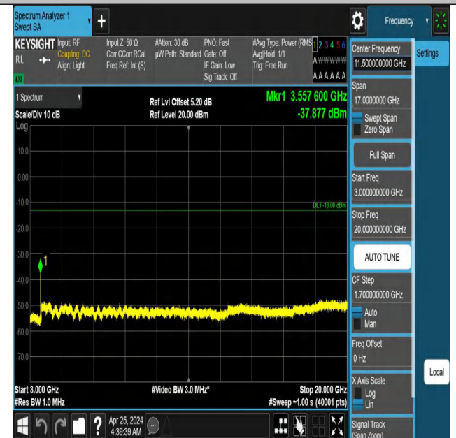
Band66_20MHz_QPSK_132572_1RB#99_3000~20000_3000~200
