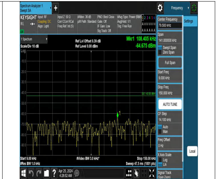
Band66_15MHz_QPSK_132047_1RB#74_0.009~0.15_0.009~0.15
