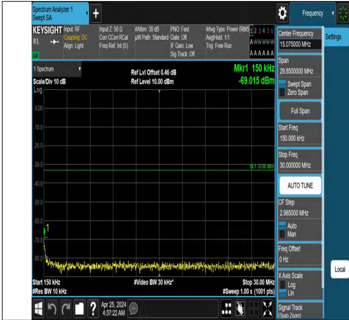
Band66_20MHz_QPSK_132072_1RB#99_0.15~30_0.15~30
