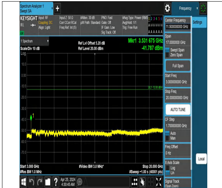
Band66_15MHz_QPSK_132597_1RB#0_3000~20000_3000~20000
