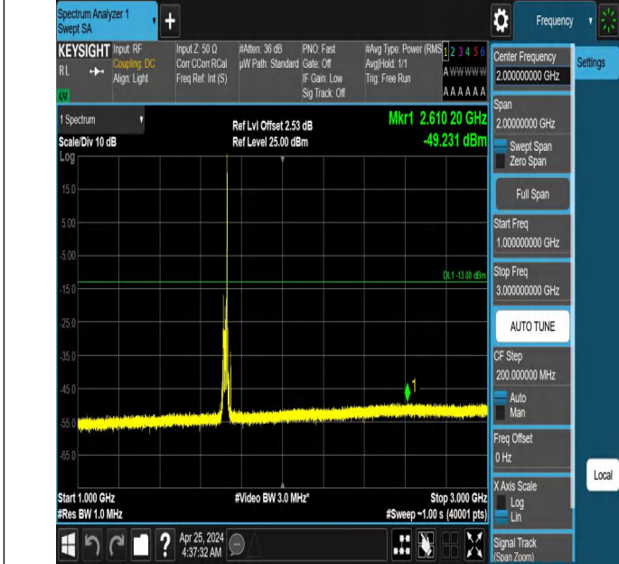
Band66_20MHz_QPSK_132072_1RB#99_1000~3000_1000~300
