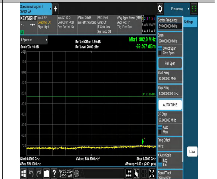
Band66_15MHz_QPSK_132047_1RB#74_30~1000_30~1000
