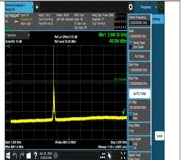
Band66_20MHz_QPSK_132322_1RB#0_1000~3000_1000~3000
