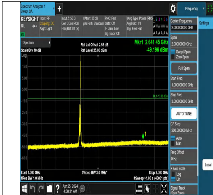
Band66_20MHz_QPSK_132322_1RB#99_1000~3000_1000~3000
