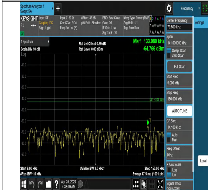
Band66_20MHz_QPSK_132572_1RB#0_0.009~0.15_0.009~0.15
