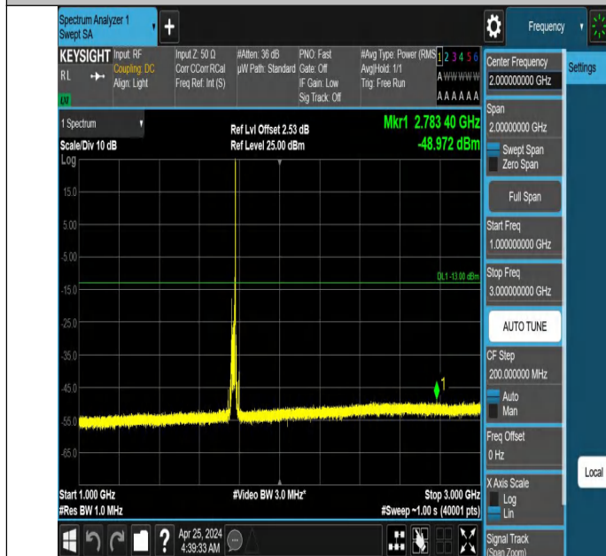
Band66_20MHz_QPSK_132572_1RB#99_1000~3000_1000~300
