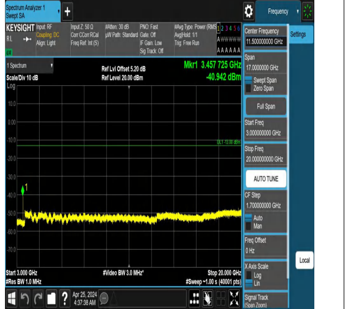
Band66_20MHz_QPSK_132072_1RB#99_3000~20000_3000~200
