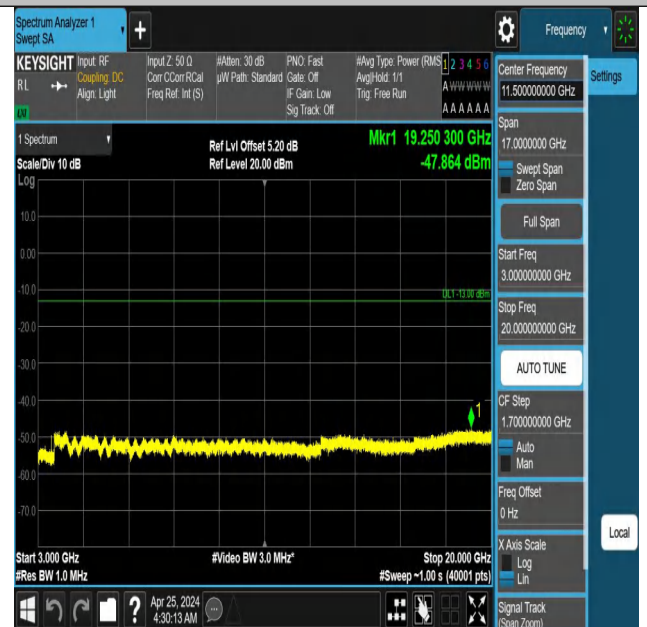
Band66_15MHz_QPSK_132322_1RB#74_3000~20000_3000~200
