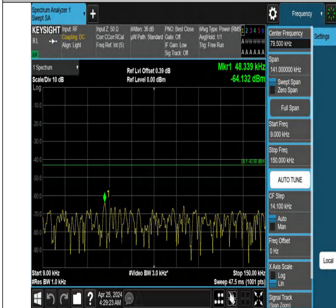
Band66_15MHz_QPSK_132322_1RB#0_0.009~0.15_0.009~0.15
