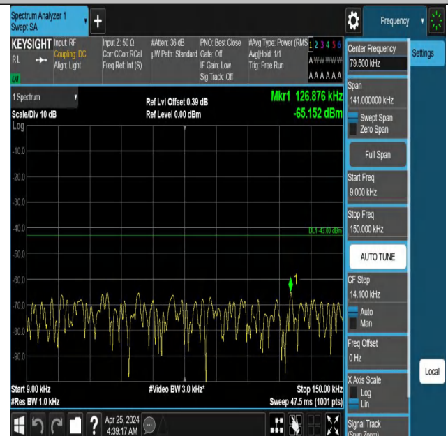
Band66_20MHz_QPSK_132572_1RB#0_1000~3000_1000~3000
