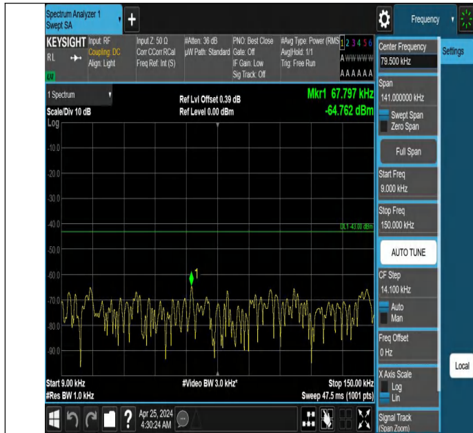
Band66_15MHz_QPSK_132597_1RB#0_0.009~0.15_0.009~0.15
