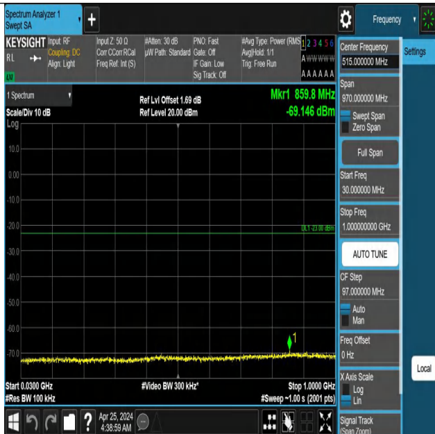
Band66_20MHz_QPSK_132572_1RB#0_30~1000_30~1000
