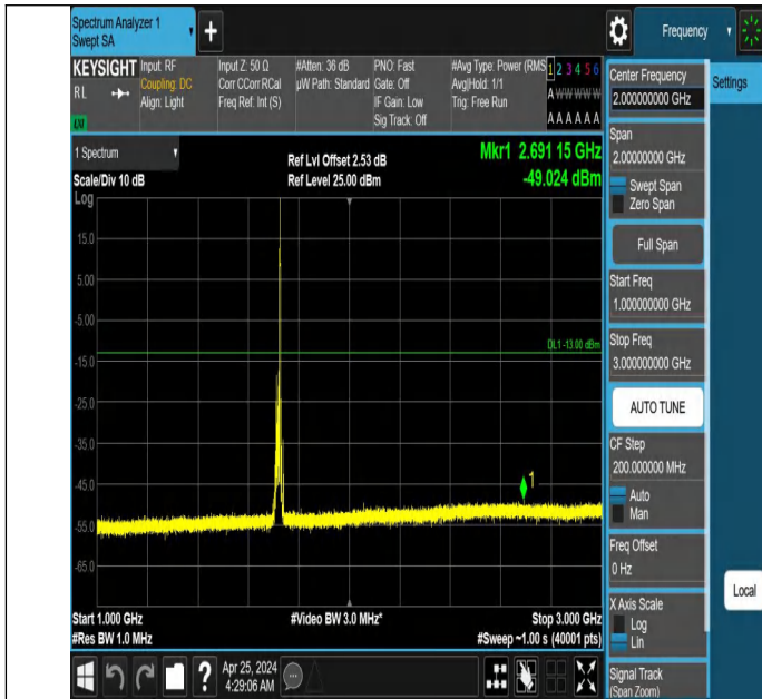
Band66_15MHz_QPSK_132047_1RB#74_1000~3000_1000~300
