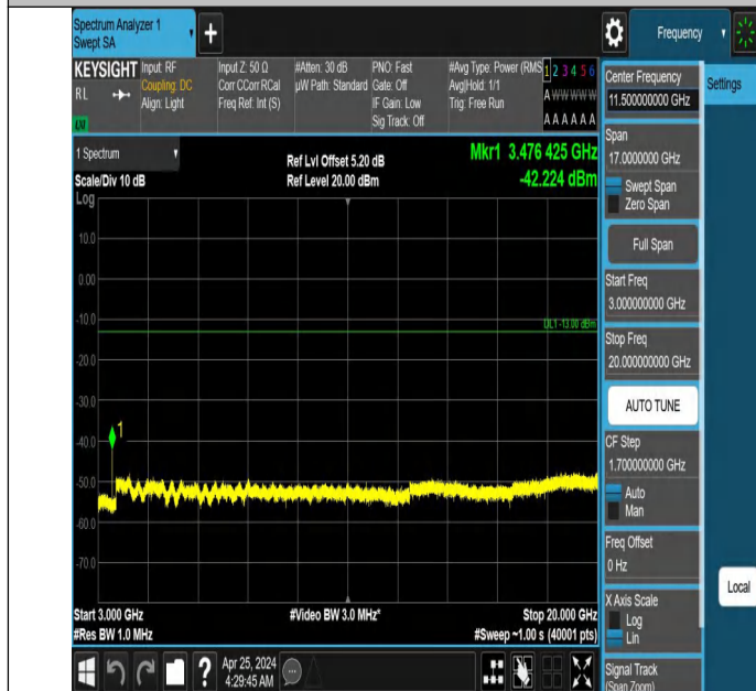
Band66_15MHz_QPSK_132322_1RB#0_3000~20000_3000~200
