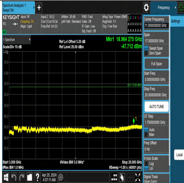
Band66_20MHz_QPSK_132072_1RB#0_3000~20000_3000~200
