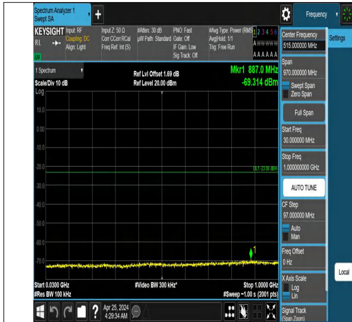
Band66_15MHz_QPSK_132322_1RB#0_30~1000_30~1000
