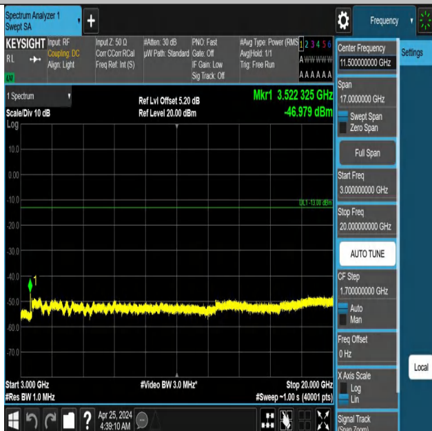
Band66_20MHz_QPSK_132572_1RB#0_3000~20000_3000~200
