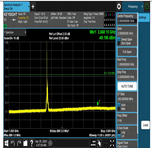
Band66_20MHz_QPSK_132072_1RB#0_1000~3000_1000~3000
