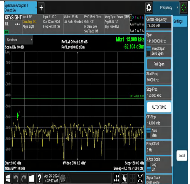
Band66_20MHz_QPSK_132072_1RB#99_0.009~0.15_0.009~0.15
