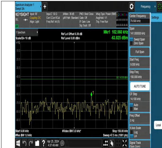
Band66_20MHz_QPSK_132322_1RB#0_0.009~0.15_0.009~0.15
