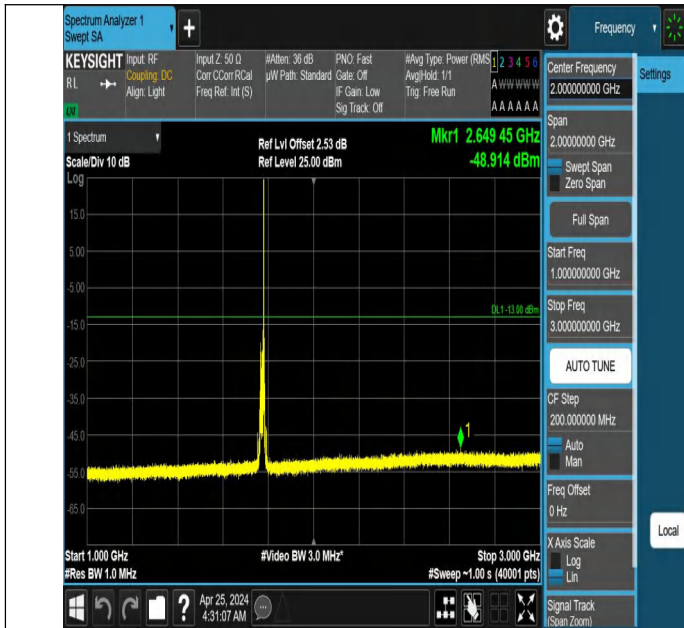
Band66_15MHz_QPSK_132597_1RB#74_1000~3000_1000~300
