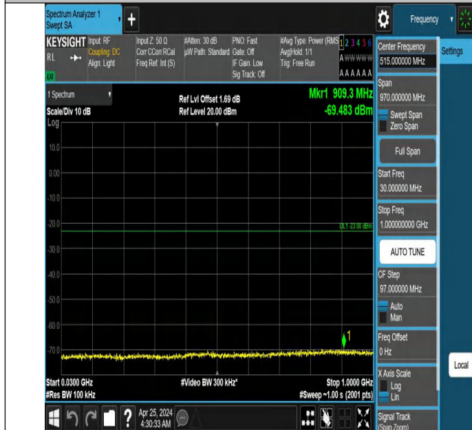
Band66_15MHz_QPSK_132597_1RB#0_30~1000_30~1000
