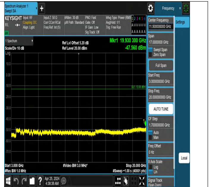
Band66_20MHz_QPSK_132322_1RB#99_3000~20000_3000~20000
