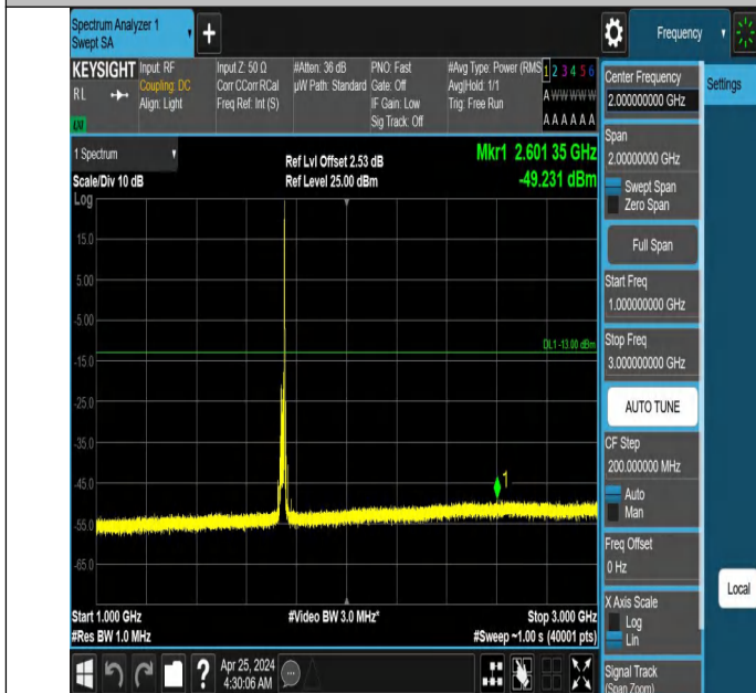
Band66_15MHz_QPSK_132322_1RB#74_1000~3000_1000~300
