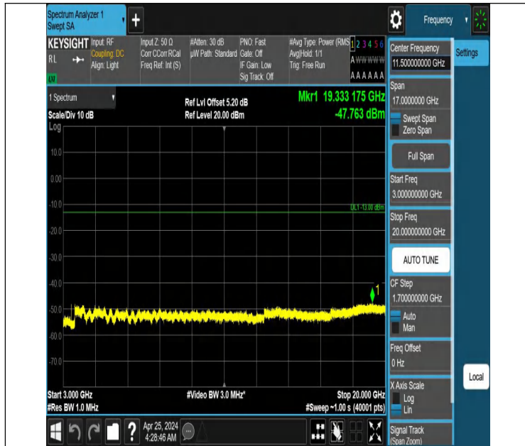
Band66_15MHz_QPSK_132047_1RB#0_3000~20000_3000~20000
