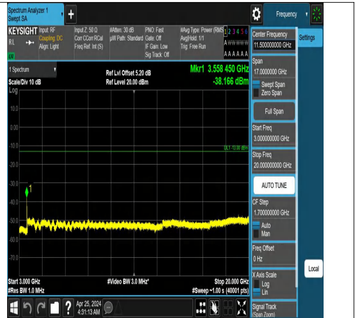
Band66_15MHz_QPSK_132597_1RB#74_3000~20000_3000~200
