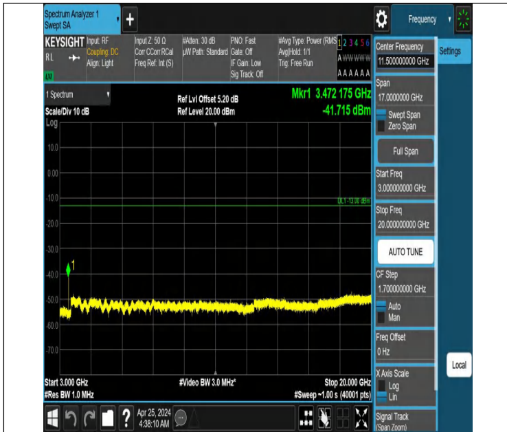
Band66_20MHz_QPSK_132322_1RB#0_3000~20000_3000~20000
