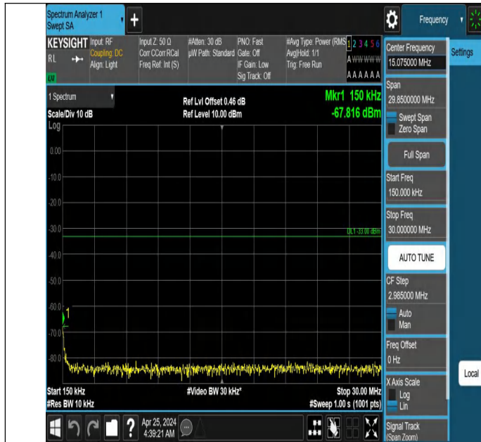
Band66_20MHz_QPSK_132572_1RB#99_0.15~30_0.15~30
