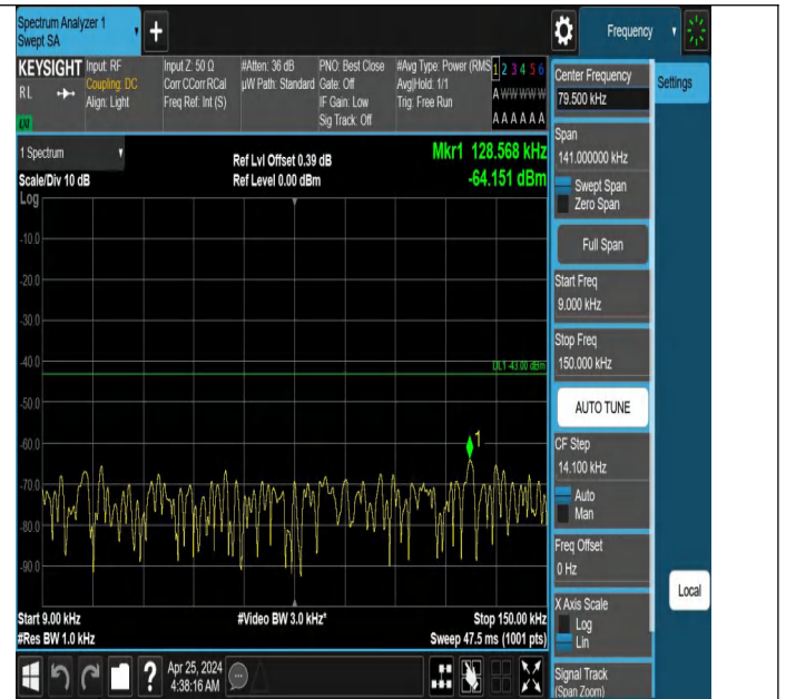
Band66_20MHz_QPSK_132322_1RB#99_0.009~0.15_0.009~0.15
