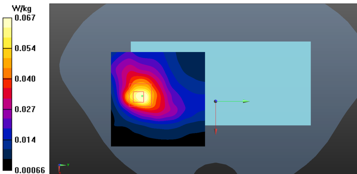
Fig.26 Bluetooth Body
