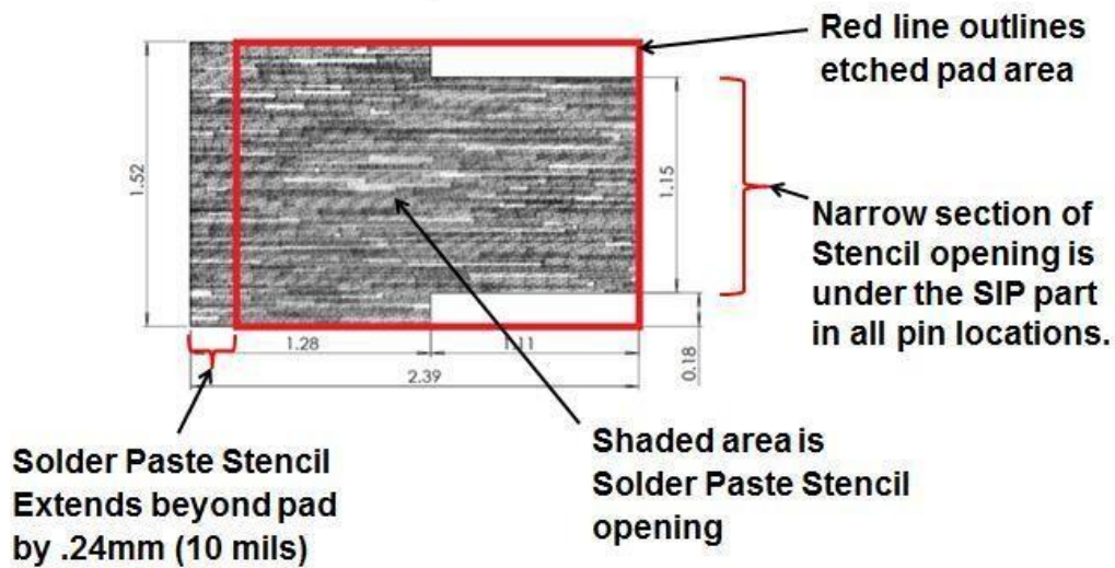
Figure 8-7: Recommended Solder Stencil Opening with Etched Pad for RS500
