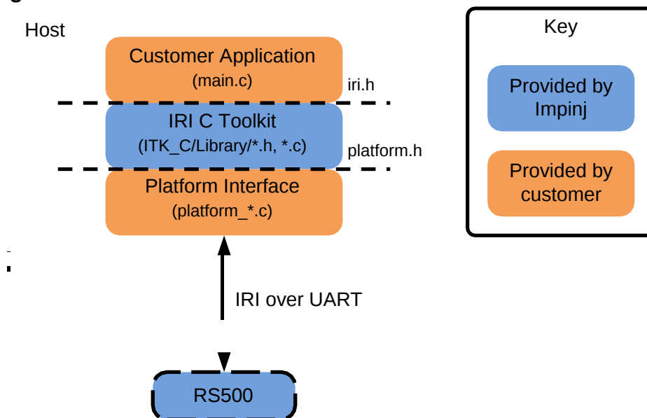
Figure 6-1: Host and Reader Firmware Stack
