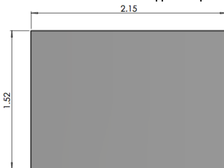
Figure 8-4: RS500 Recommended Etched Copper Footprint – Single Pad
