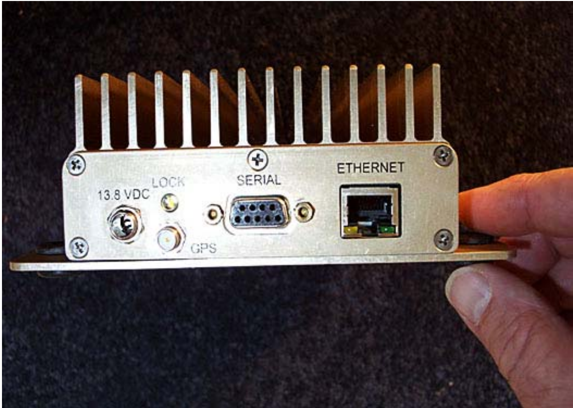
Front
