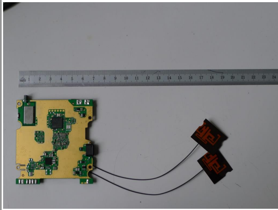
EUT INTERNAL DETAIL (B)
